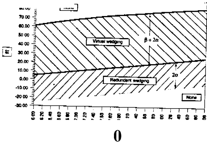
Fig. 3: \beta_{i,j} of virtual and redundant wedging for the contacts in Fig. 2: \alpha = 20^\circ , \beta_i = 90^\circ , a = 15^\circ and d_1 = 4.0 cm, d_2 = 7.0 cm, d_3 = 8.0 cm
