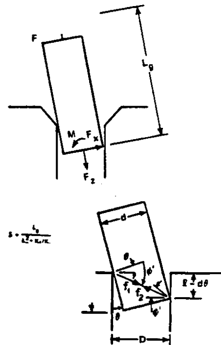
Fig. 6: Wedging diagram for two-dimensional peg insertion tasks
