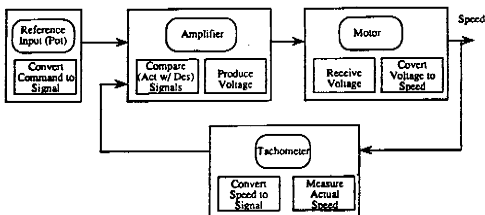
Fig. 6. The transformation of the FBD of Figure 5
