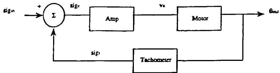
Equivalent Control Block Diagram
