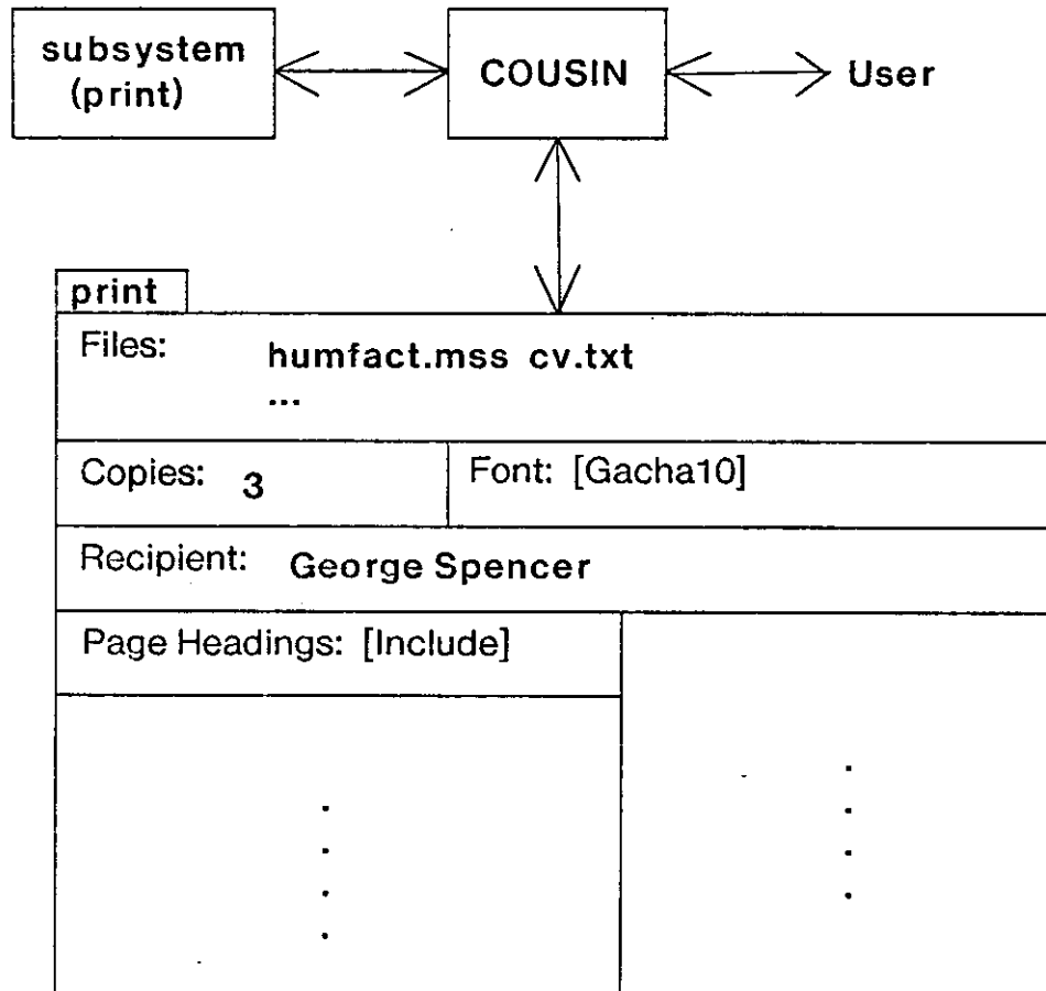
Figure 1: Communication by Form-Filling
