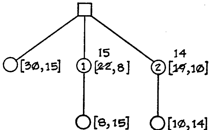
Figure 3 - The DISPROVEREST Strategy
