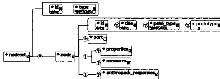
Figure 3: Specification of Vertices in DyNetML
