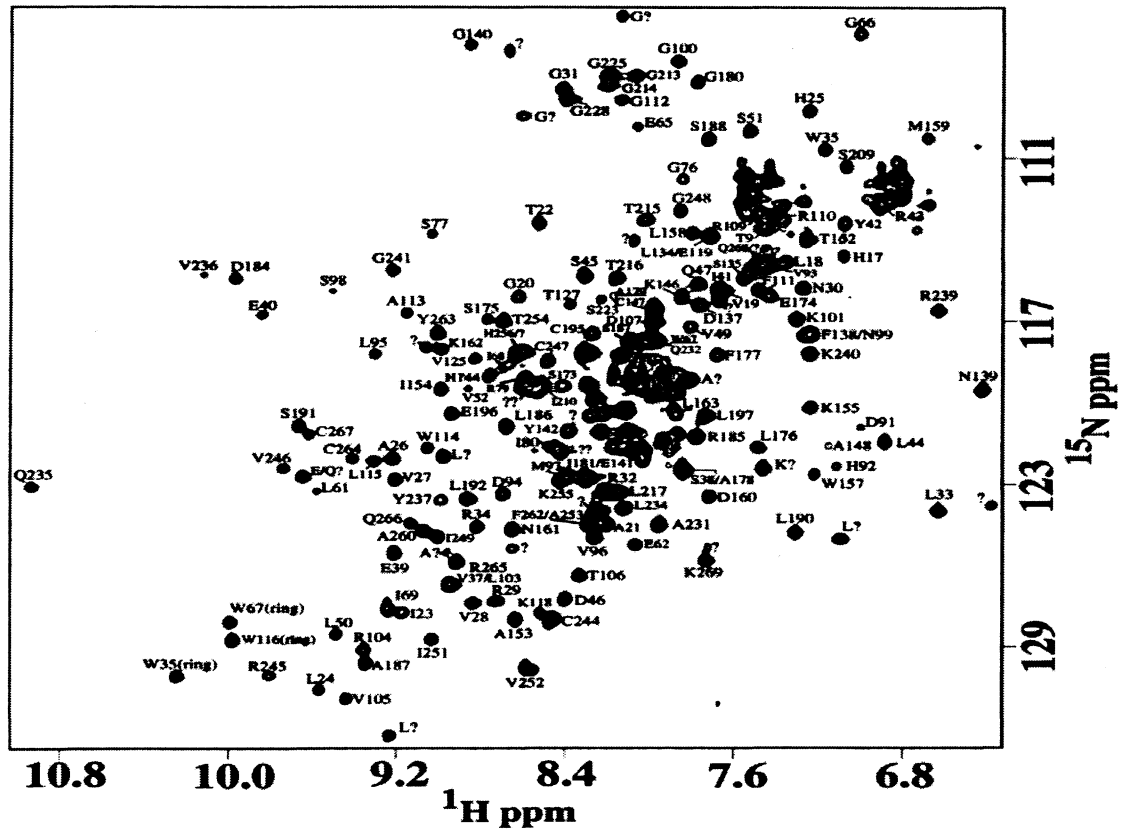
Figure 1: Two-dimensional ^1\text{H}/^{15}\text{N} Heteronuclear Single-Quantum Coherence (HSQC) NMR spectra of an E. coli DNA glycosylase, Fpg. (from http://www.emsl.pnl.gov/homes/msd/bionmr/Buchko_Fpg_poster/Fpg.htm )
