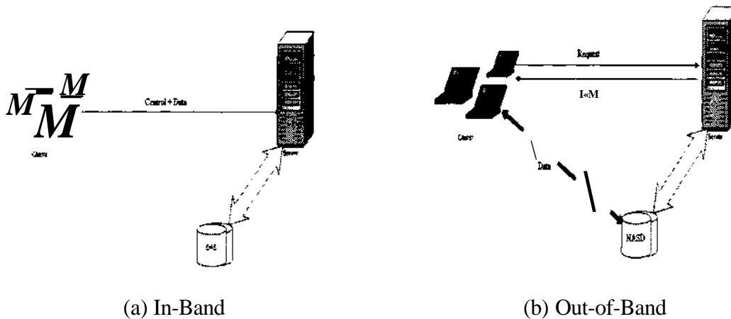
Figure 1: Two ways of data access in a file level network attached storage. The in-band approach does not scale as it might get bottlenecked at the network link and/or the server. In the out-of-band scenario, the clients make requests to the server. The server hands them a "layout" of the requested file on disk. The client then uses this layout to access the storage directly for the data it needs.
