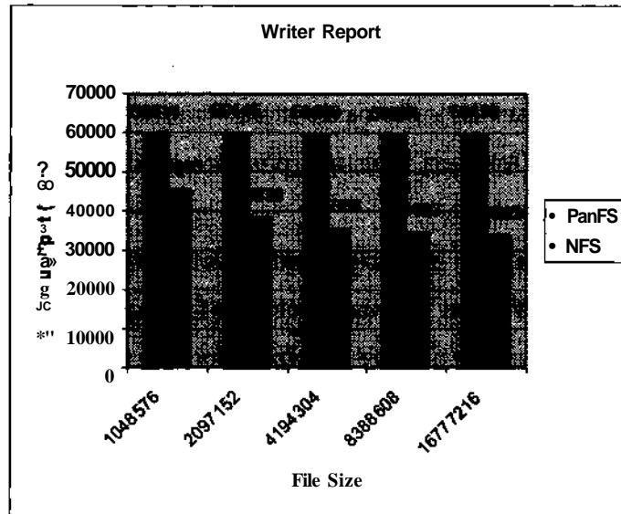
Figure 2: Sequential Write Performance for large file sizes
