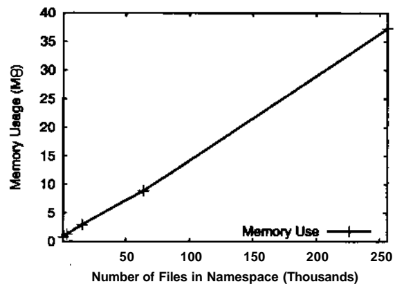
Figure 6: Memory use of the namespace tree.
