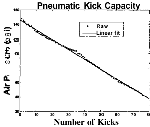
Figure 14. Number of Kicks v. Reservoir Pressure
