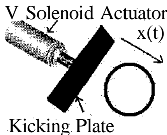
Figure 8. Solenoid Kicker Schematic
