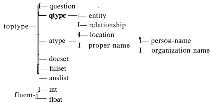
Figure 6: Partial type hierarchy for JAVELIN. The three numeric types (fluent, int , float) and toptype are automatically defined by the PLEXIS planner.
