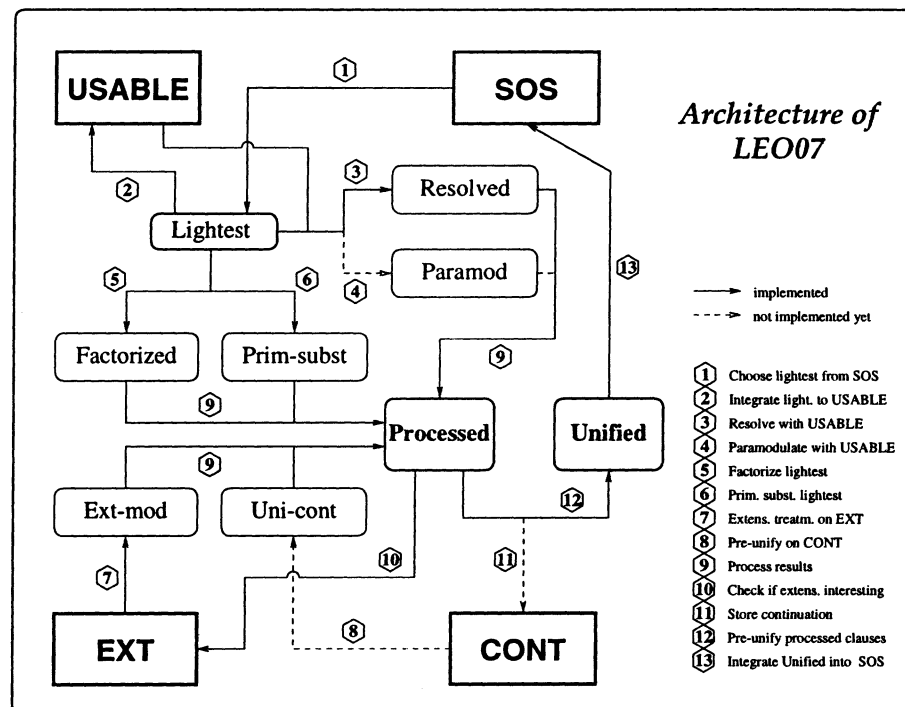
Figure 5: The refutation strategy LEO07
