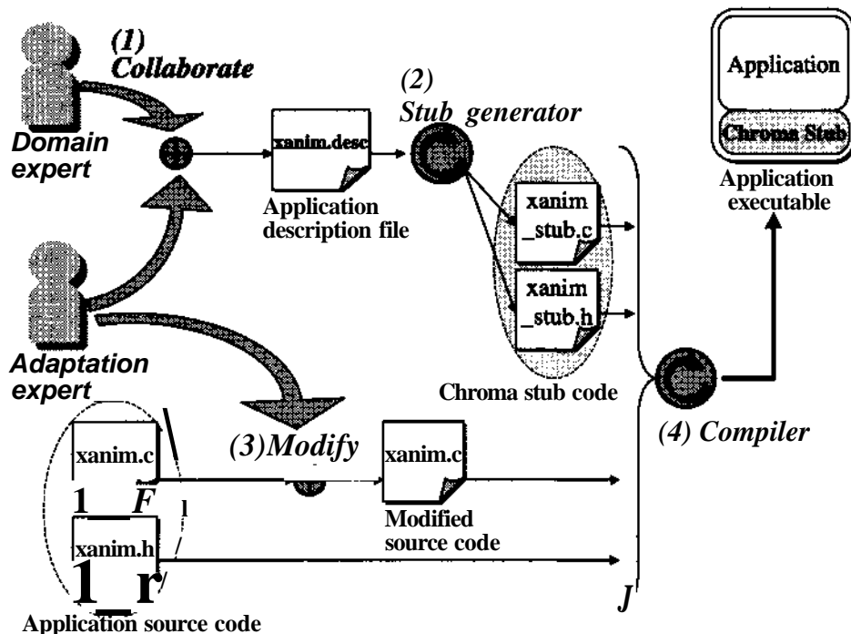
Figure 1: Process for adding adaptation to an application
