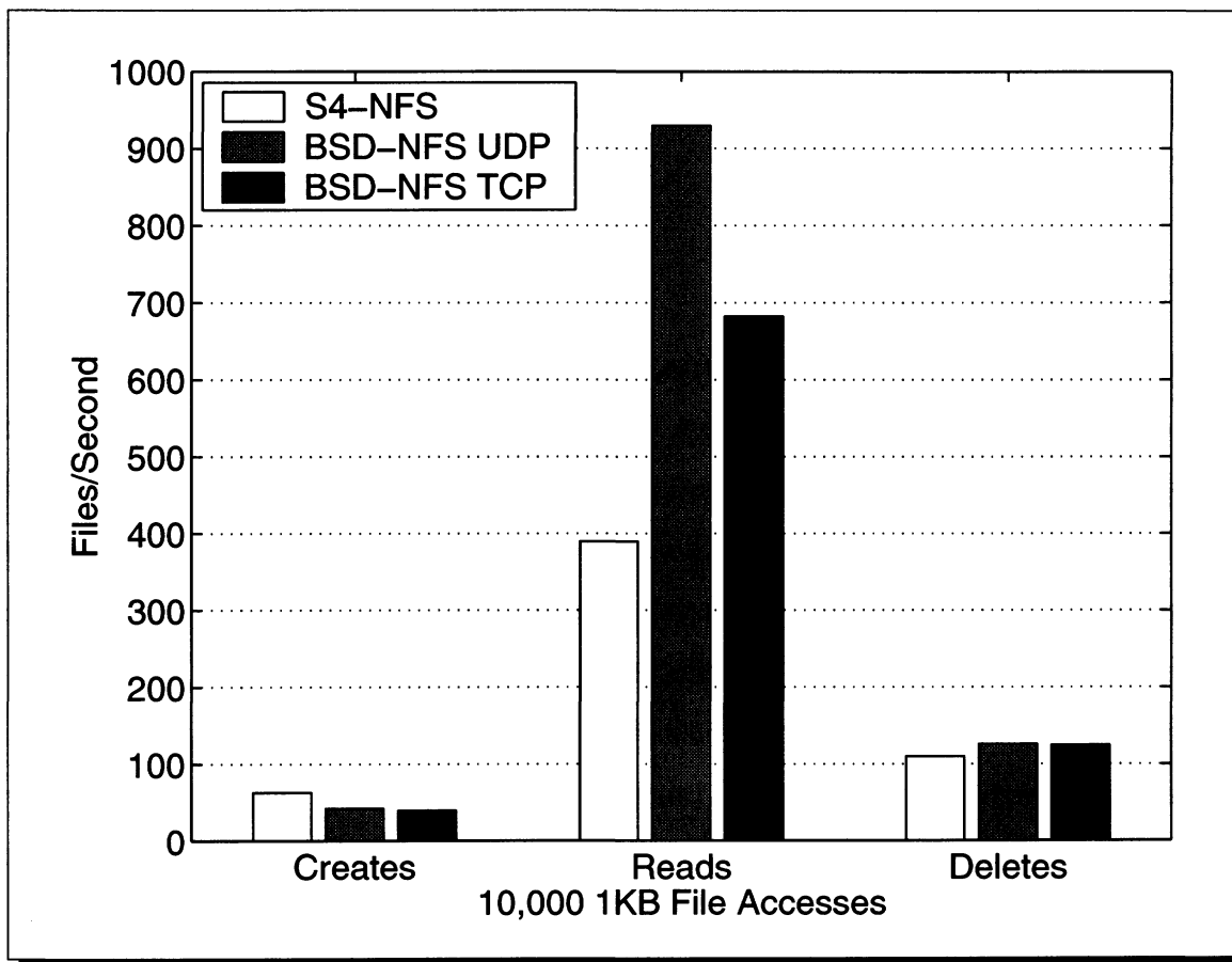
Figure 7: Small-file performance.
