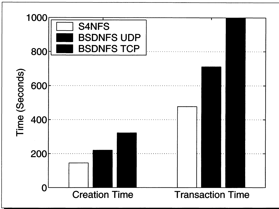
Figure 9: Postmark benchmark.
