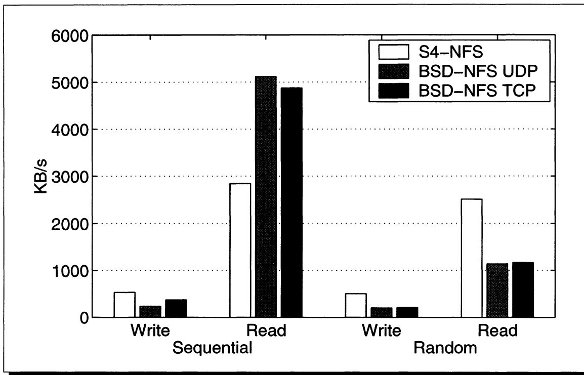
Figure 8: Large-file performance.
