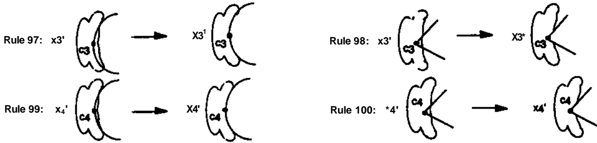
Figure 7. Completion rules
