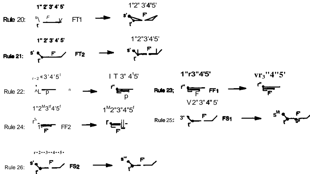
Figure 4. Filter rules
