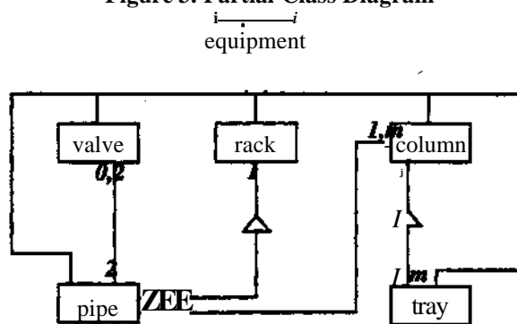
Figure 3. Partial Class Diagram 4
