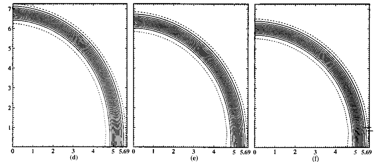
Figure 7: Optimum shapes for different objective functions: (a) \mathbb{S} , (b) \mathfrak{r} , (c) \mathfrak{S} , (d) \hat{\mathbb{S}} , (e) \hat{\mathfrak{r}} , (f) Q .
