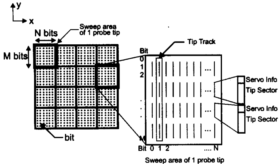
Figure 3: Data organization of MEMS-based storage. The illustration depicts a small portion of the magnetic media sled. Each rectangle outlines the area accessible by a single probe tip, with a total of 16 tip regions shown. (A full device contains thousands of tips and tip regions.) Each region stores N \times M bits, organized into vertical "tip sectors" containing encoded data and ECC bits. These tip sectors are demarcated by "servo information" strings that identify the sector and track information encoded on a disk. To read or write data, the media passes over the active tip(s) in the \pm Y direction while the tips access the media.
