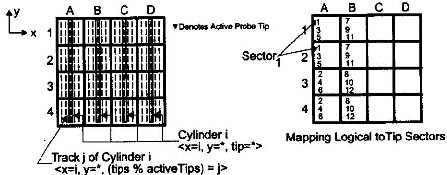
Figure 4: Cylinders, Tracks, and Sectors. Cylinder_i is defined as all of the columns of data with the same X coordinate: \langle x = i, y, tip \rangle . Track_{i,j} is the subset of a cylinder that is accessible by the concurrently active tips: \langle x = i, y, (tip \% activeTips) = j \rangle . (Note that activeTips=4 in this figure and that the tips are linearly numbered such that A1=0, A2=1 , etc.) Each logical sector in the figure to the right consists of two tip sectors. For example, Sector_1 consists of the first tip sectors of the two upper tip regions, A1 and A2.
