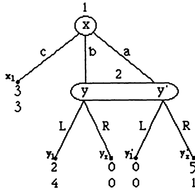
Figure 1: A two-person game of imperfect information.
