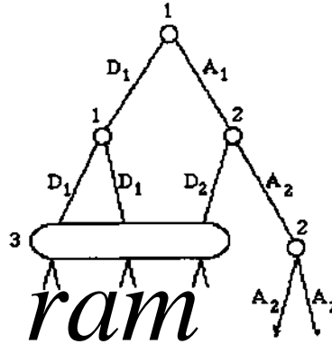
Figure 6: The "balanced" version of figure 5.
