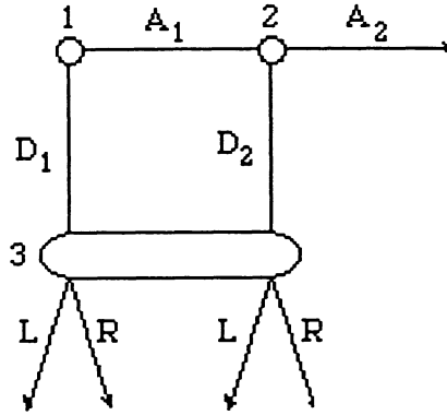
Figure 5: An unbalanced tree.
