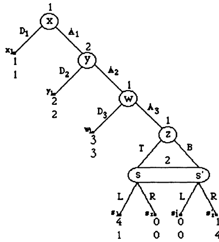
Figure 3: A more complex two-person game.
