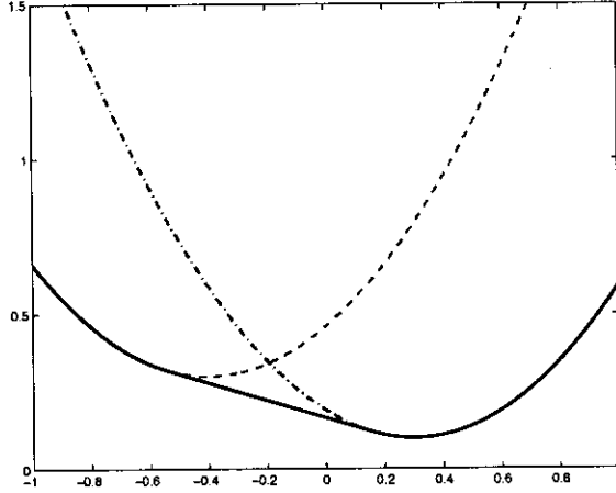
Figure 3: Given two functions F (dashed line) and G (dash-dot), we can define \text{conv min}(F, G) (solid line) to be the pointwise greatest convex function H such that H(y) \leq \min(F(y), G(y)) for all y .
