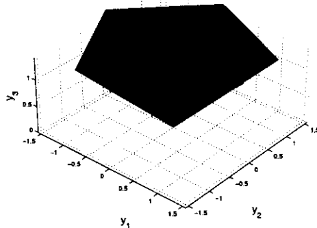
Figure 5: Hypothesis space \mathcal{Y} after including constant component, together with the cone \bar{\mathcal{Y}} containing \mathcal{Y} .
