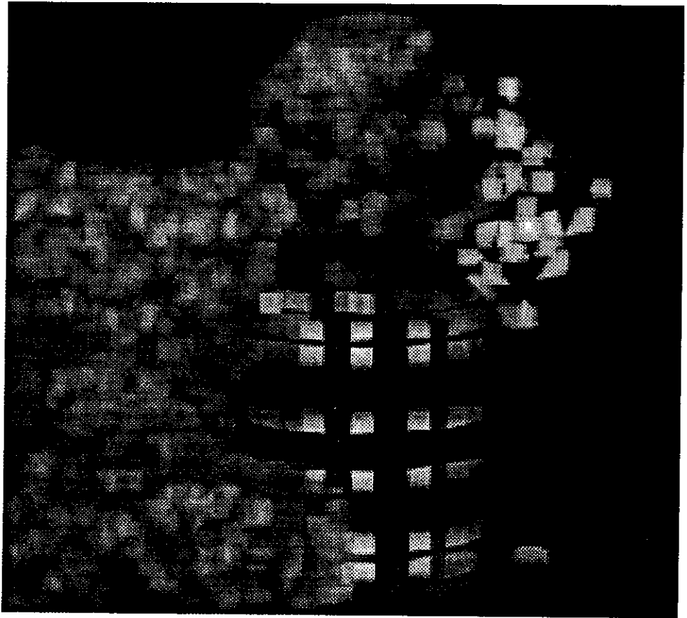
Figure 5.3: The minor eigenvalue of G (see equation (3.2)) for the first frame in the stream (figure (5.1)). Brighter areas correspond to higher values. The intensities in this display were compressed logarithmically. The square patterns reflect the shape of the 15 \times 15 window used by the detector (and the tracker).
