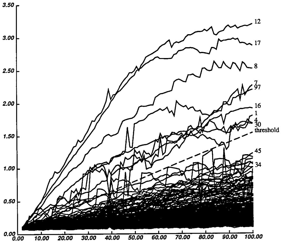
Figure 5.9: Cumulative root-mean-squared residues between the current and the first frame for all of the features selected by our method. Units are intensity levels per pixel, versus the frame number. Features 7, 8, 12, 16, 17, and 97 are occluded during the stream.
