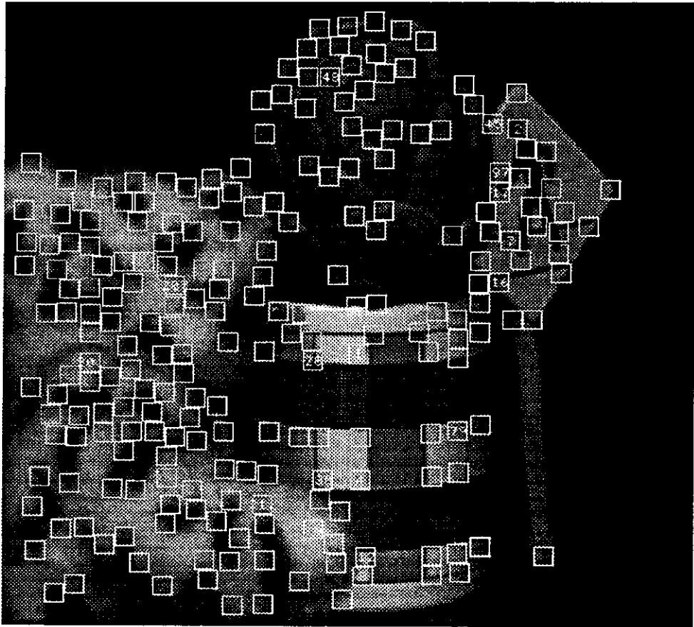
Figure 5.5: The non-overlapping features produced by thresholding the eigenvalues of figure 5.3 with a value of 10. Some features are numbered for reference in the text.
