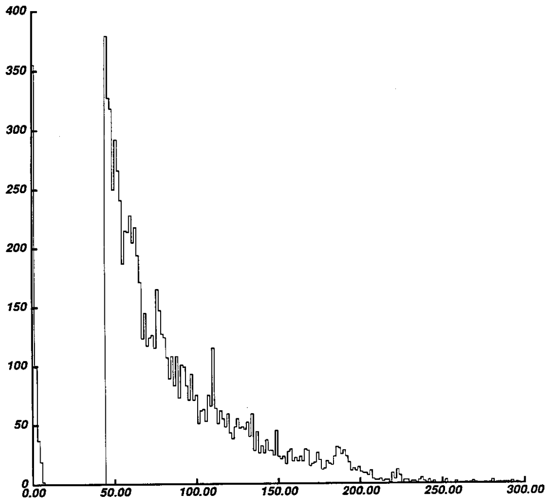
Figure 5.4: Histogram of the minor eigenvalues. Notice the wide gap between the near-zero values, corresponding to the background and to uniform regions in frame 1, and the upper cluster.
