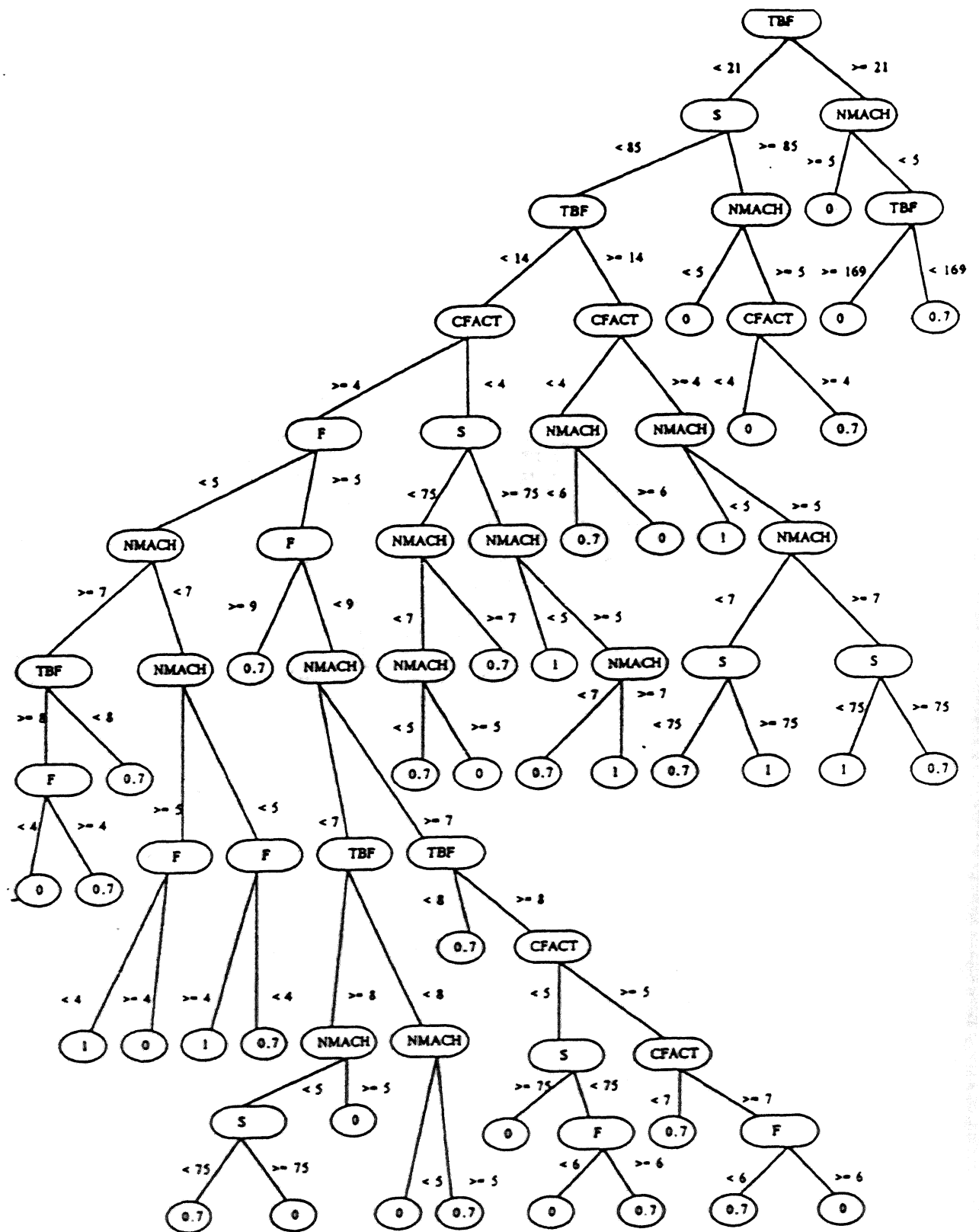
Figure 3: Decision Tree for Selecting \theta
