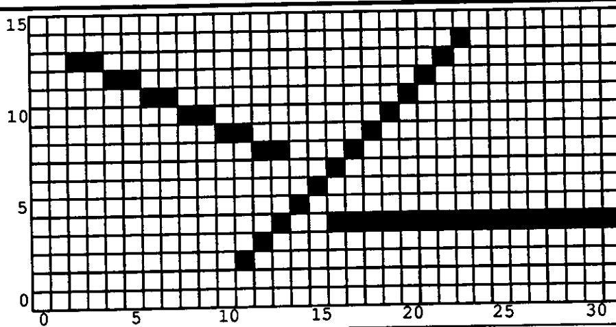
Figure 13: The pixels generated by a line drawing routine. In this example the endpoints are \langle(11, 2) : (23, 14)\rangle , \langle(2, 13) : (13, 8)\rangle , and \langle(16, 4) : (31, 4)\rangle . The algorithm allocates 12, 11 and 16 pixels respectively for the three lines.
