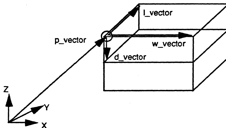
Figure 4. Definition of a Face Feature.
