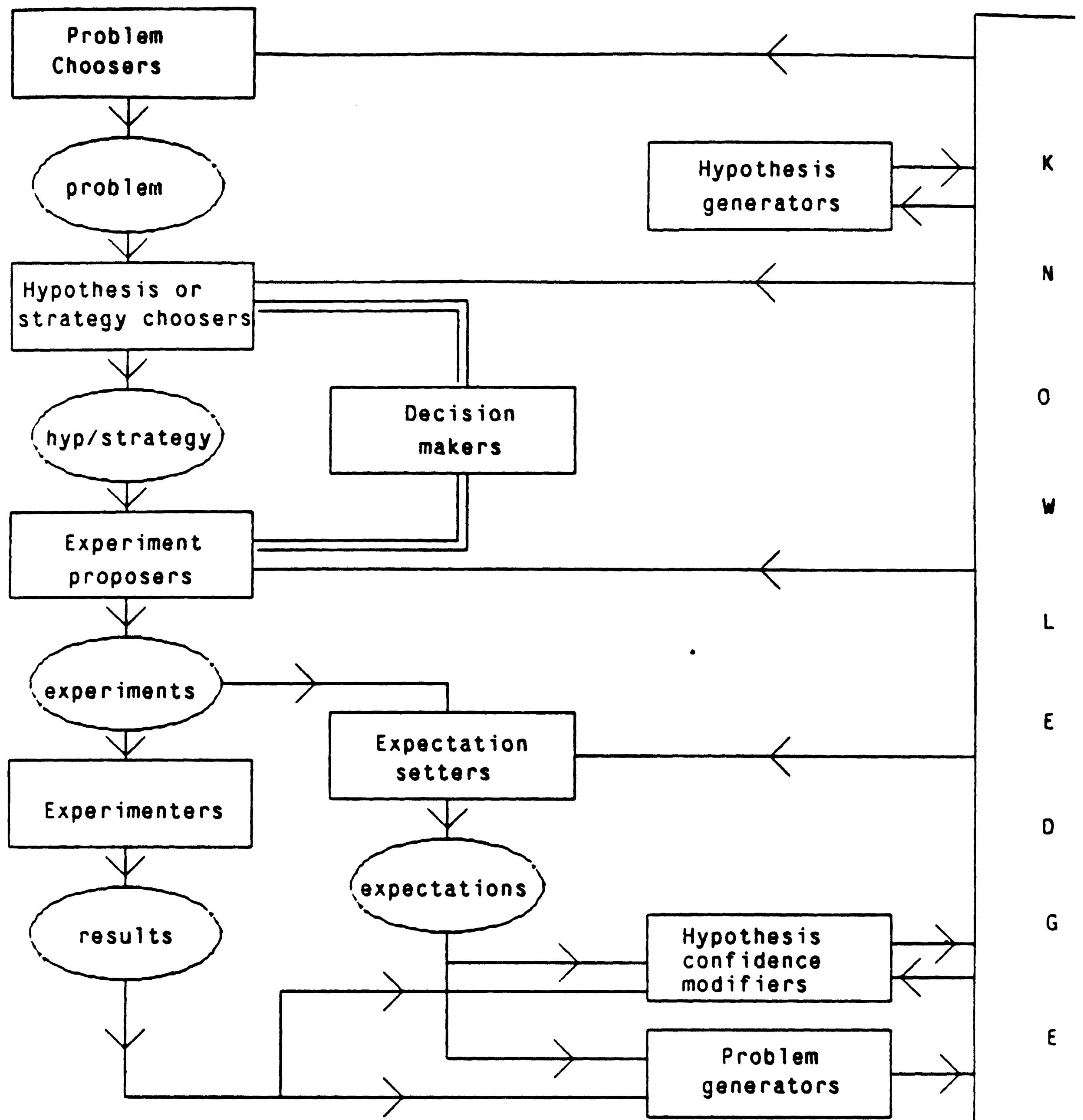
Figure 2-2: Interaction of heuristics
