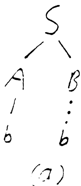
Figure 5: Two grammars for the string ba , and partial derivations for bb .
