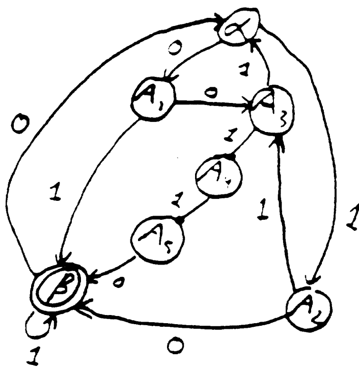
f) The final M' L(M') = L
