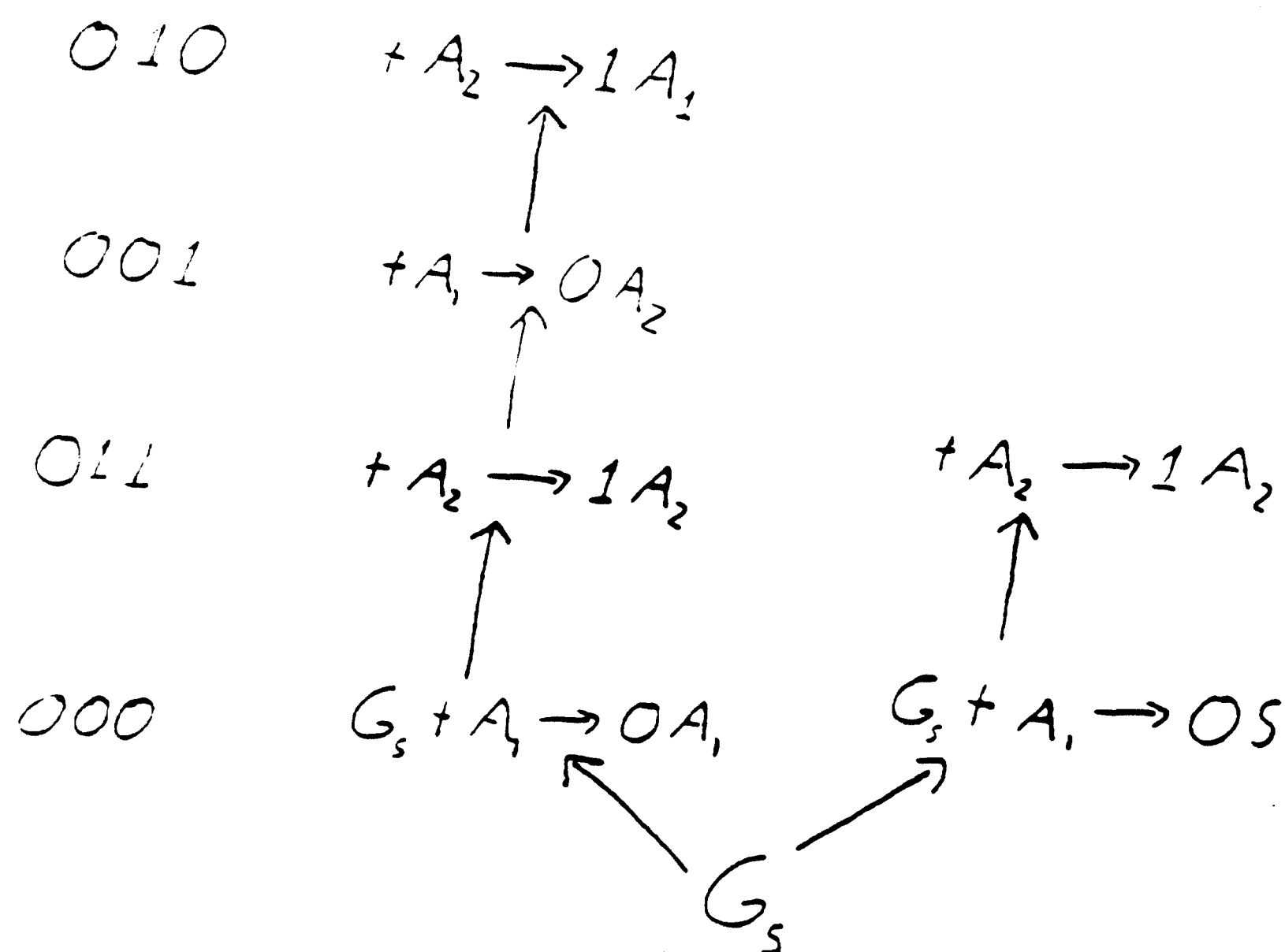
Figure 12: Tree of grammars derived for the language 0(0 + 1)^* .
