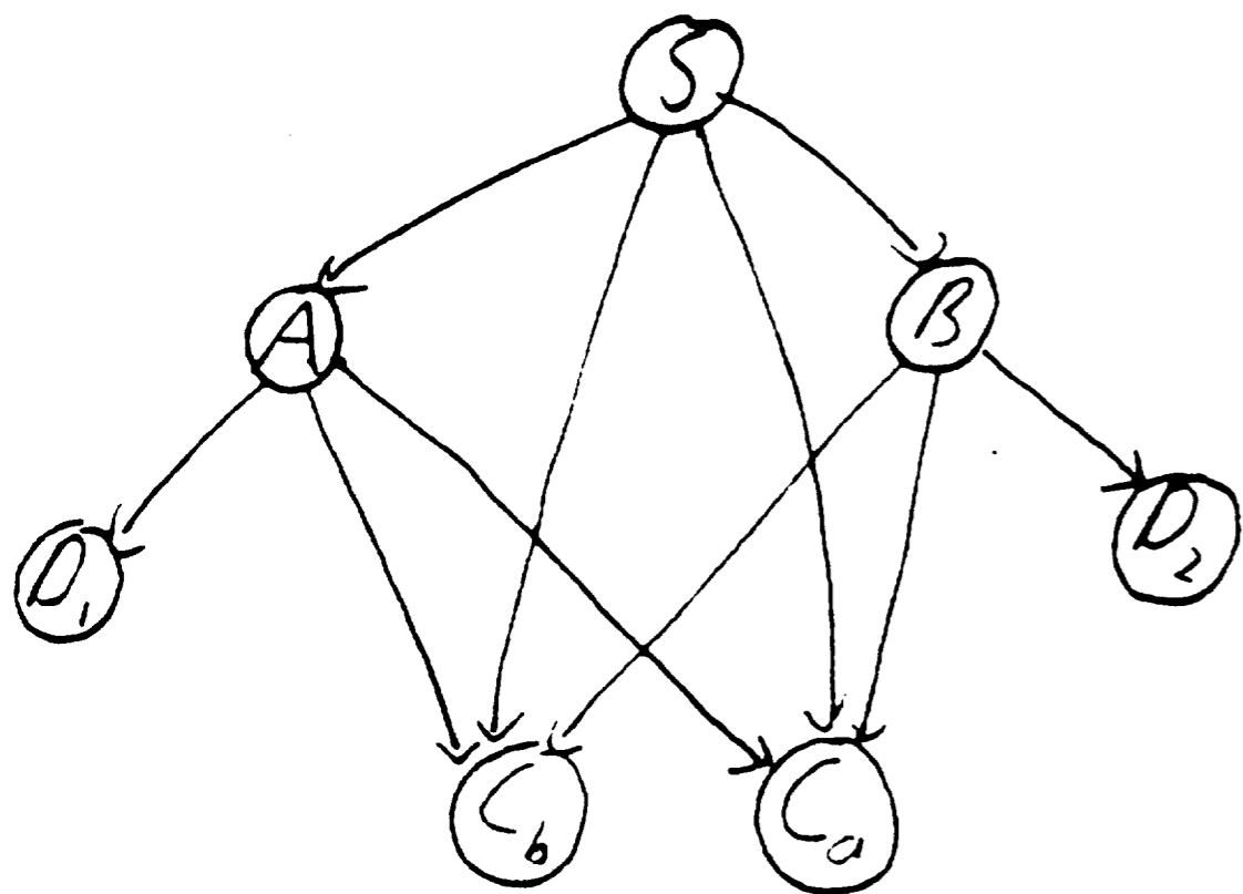
c) T' , the largest acyclic subgraph of T
