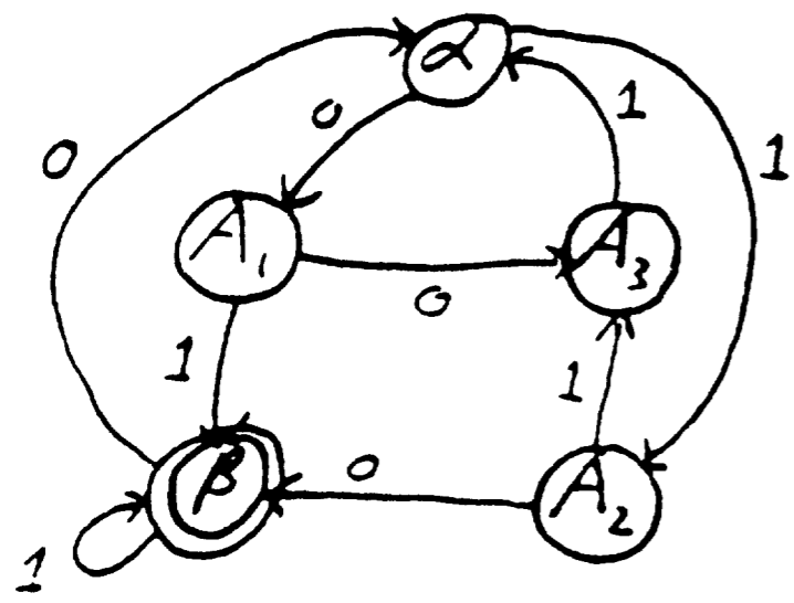
a) The machine M
