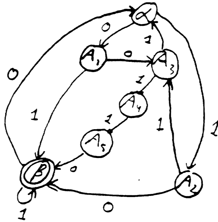
f) The final M' L(M') = L
