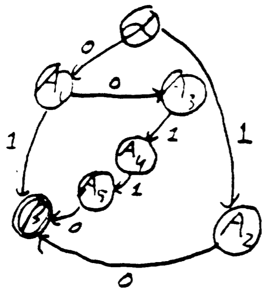
c) The final machine M_S . The path with yield 110 from A_3 to B corresponds to the path A_3 \alpha A_2 B in M .
