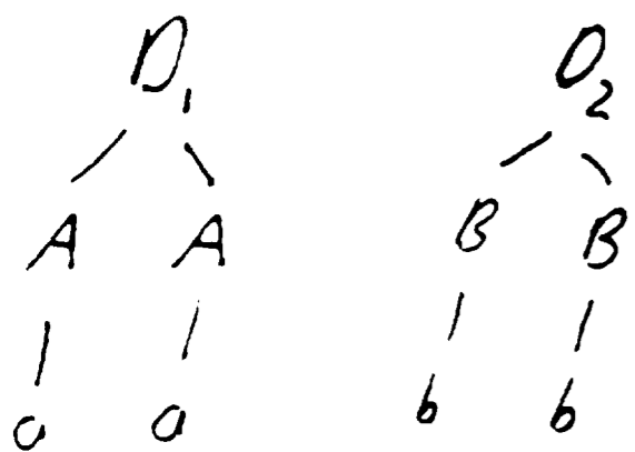
e) Derivation Trees for a shortest derivation for D_1 and D_2 in G .
