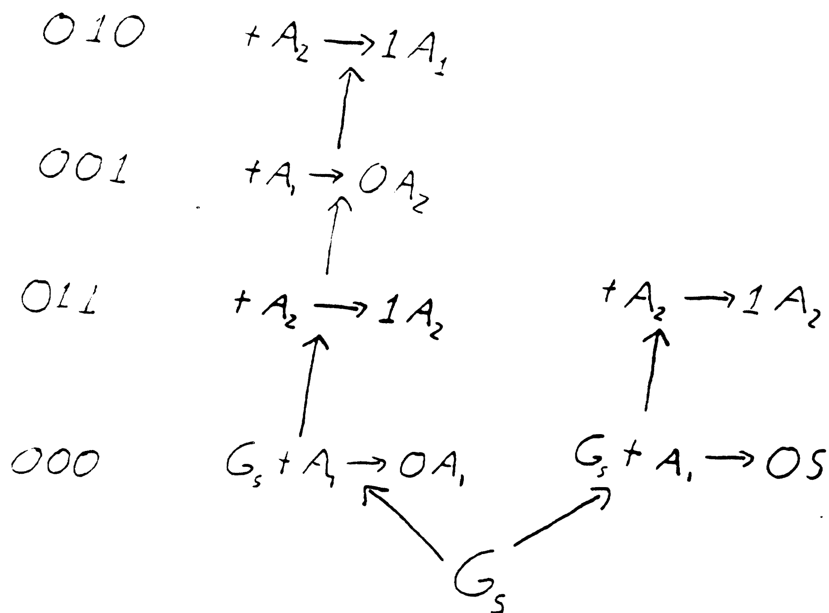
Figure 12: Tree of grammars derived for the language 0(0 + 1)^* .
