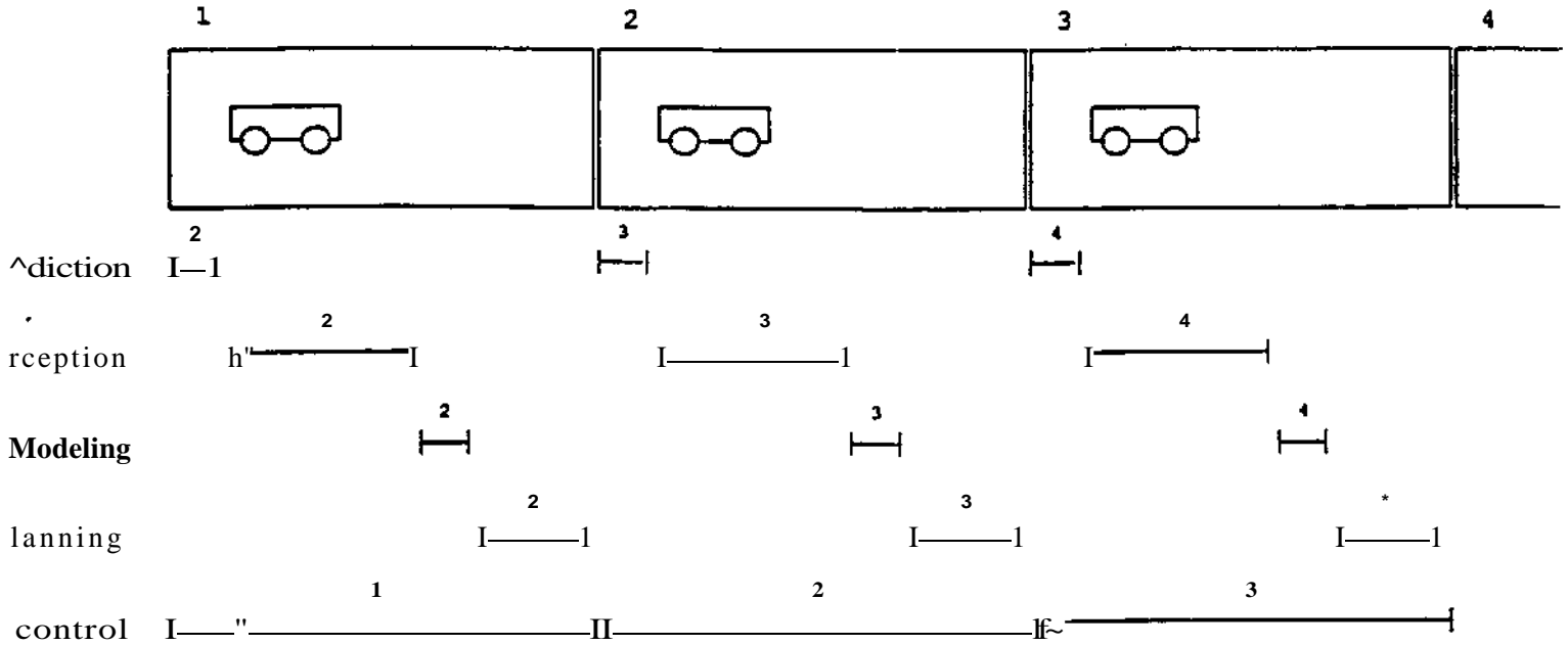
Figure 19: Badly-Balanced Execution of the Driving Pipeline
