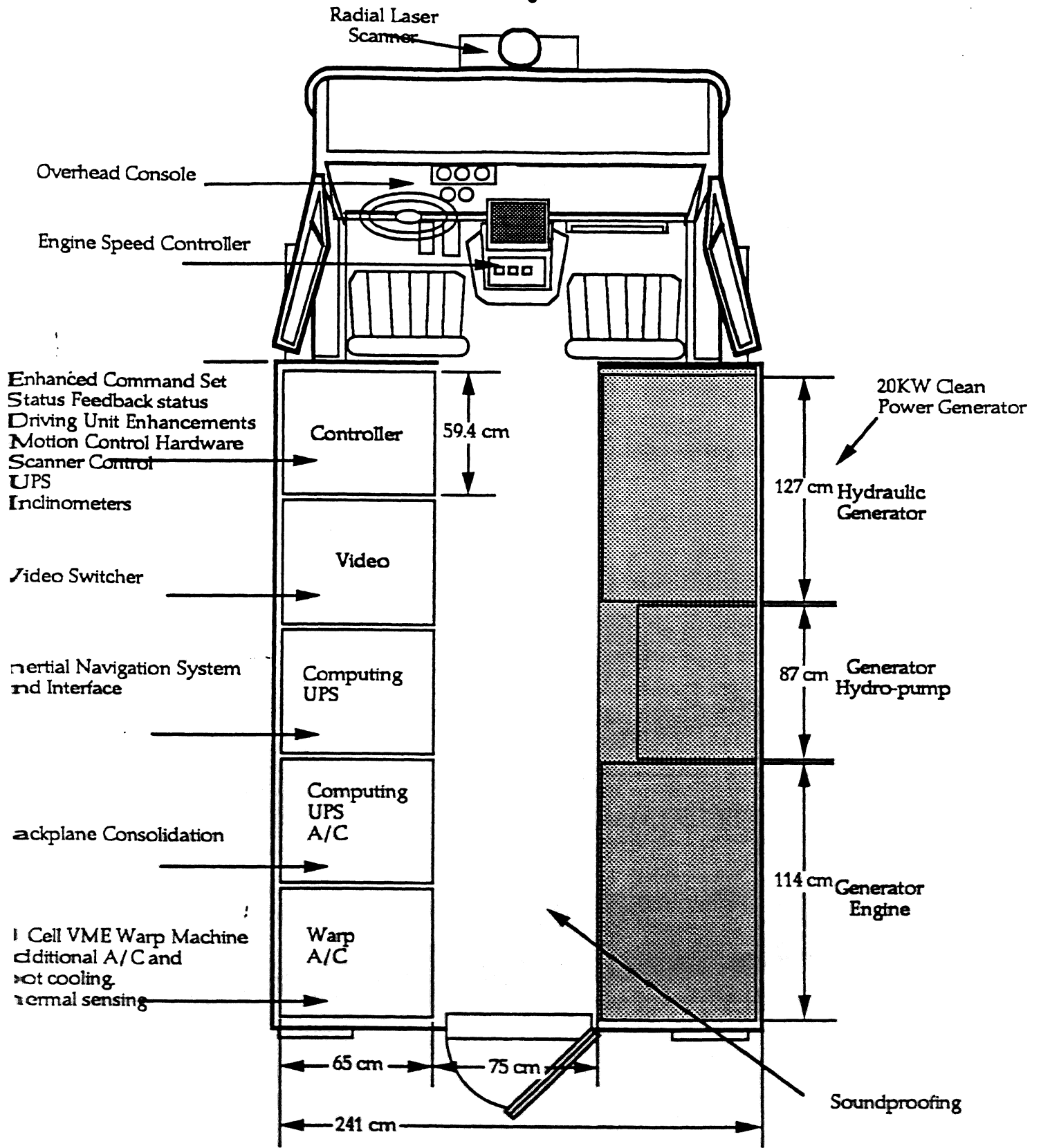
Figure 1: Improvements in the NAVLAB Vehicle
