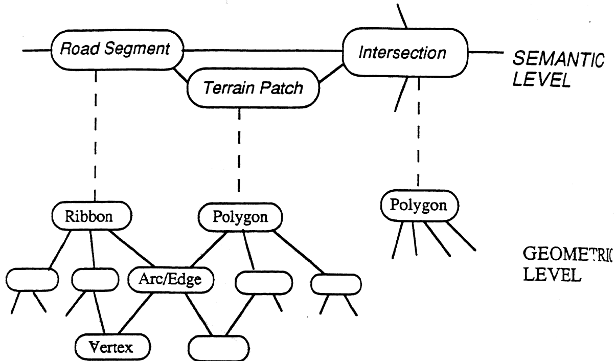
Figure 7: The Semantic/Geometric Network in CODGER II
