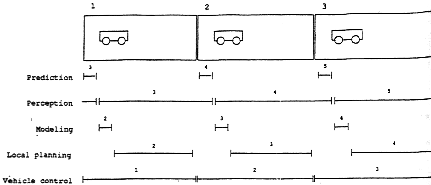
Figure 20: Parallel Execution Pattern in the Map Navigation Mode
