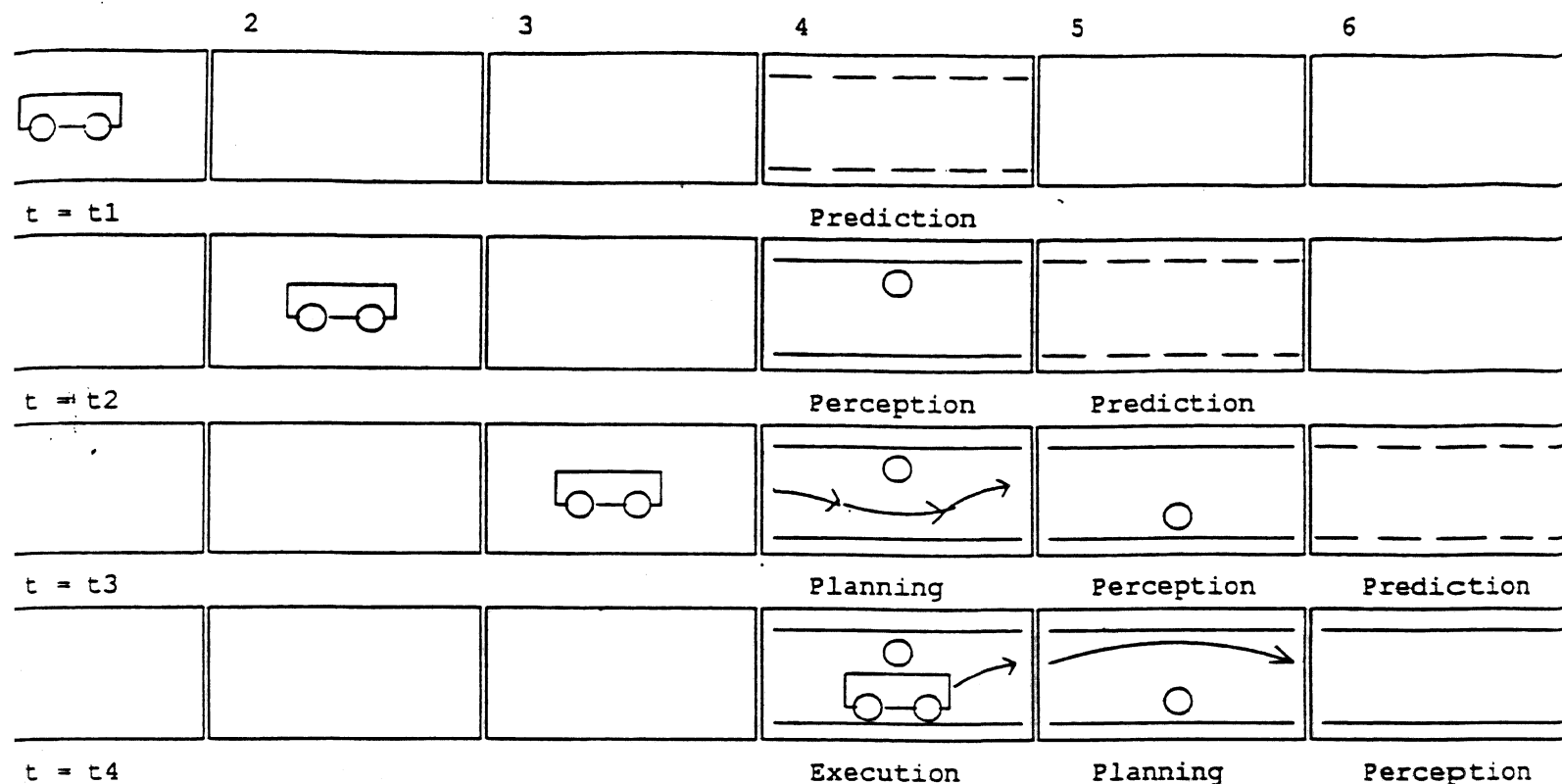
Figure 18: Pipelined Execution of the Driving Pipeline
