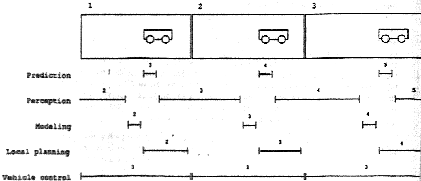
Figure 21: Parallel Execution Pattern in the Map Building Mode
