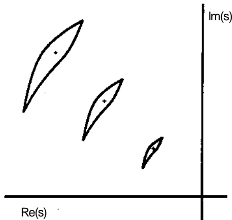
Figure 1: The control bound maps for open-loop plants with the same damping are the same shape, but have sizes which increase with natural frequency.
