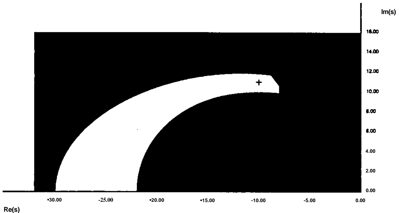
Figure 5: All closed-loop systems designed using a pole selected from the white region will meet all requirements and not violate constraints.
