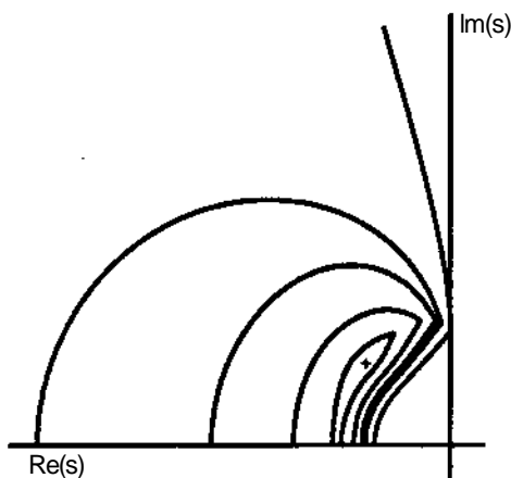
Figure 3: As the bound on control effort increases, the region of obtainable closed-loop systems increases in size and distorts in shape. Past a limiting value, the region becomes semi-infinite.
