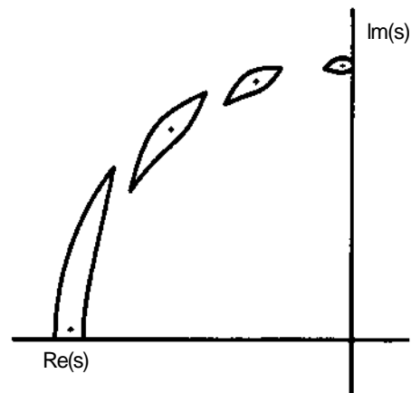
Figure 2: Control bound maps are elongated as the open-loop damping is increased while the natural frequency is constant.
