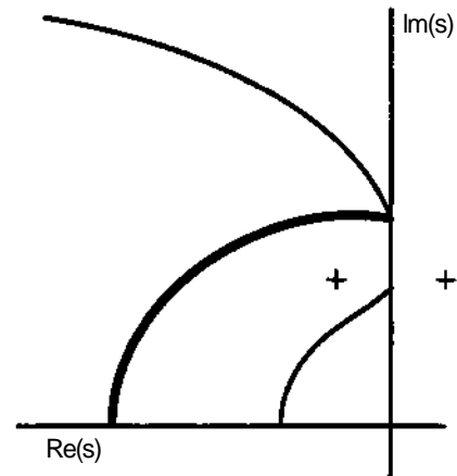
Figure 4: Maps for unstable open-loop plants are always semi-infinite regions. The region of obtainable closed-loop systems for the unstable open-loop plant is to the upper left of the thicker line.
