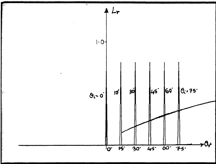
(a) \sigma_h = 0.001 , T = 0.01 , \lambda = 0.5
