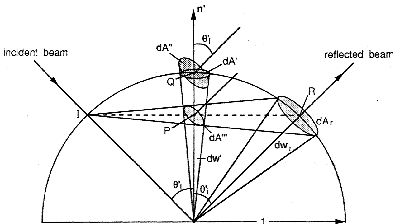
Figure 17: The source-viewer plane, illustrated to establish the relationship between d\omega' and d\omega_r .
