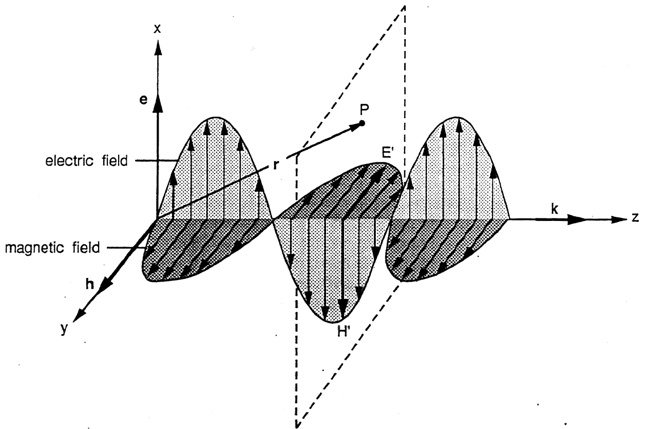
Figure 6: A plane electromagnetic wave.
