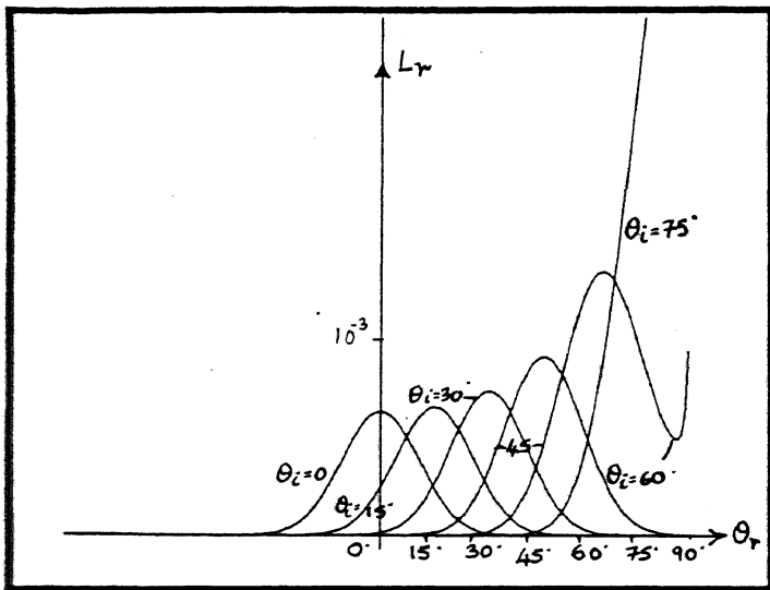
(c) \sigma_h = 0.001 , T = 0.015 , \lambda = 0.0001
