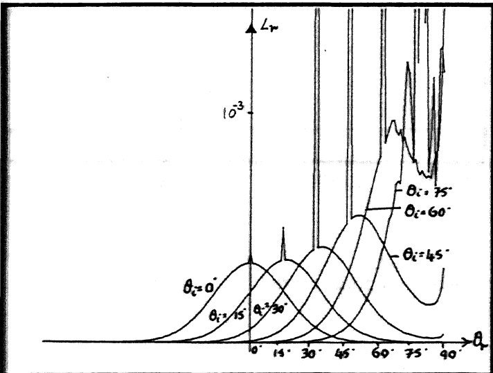
(e) \sigma_h = 0.001 , T = 0.01 , \lambda = 0.003
