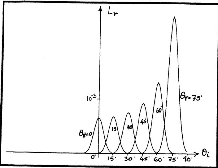
(a) \sigma_h = 0.003 , T = 0.01 , \lambda = 0.001
