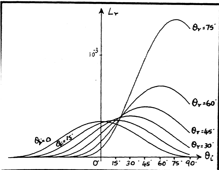
(e) \sigma_h = 0.002 , T = 0.01 , \lambda = 0.001
