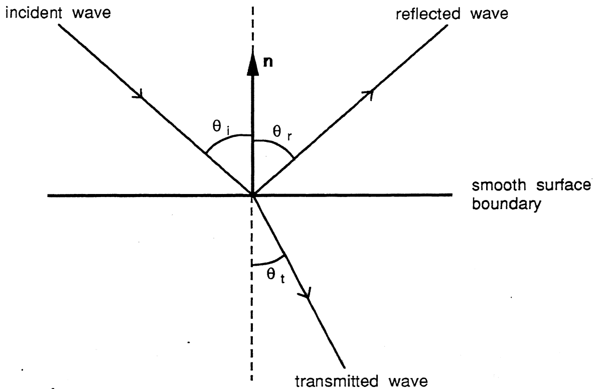
Figure 8: Light waves incident on a smooth surface.
