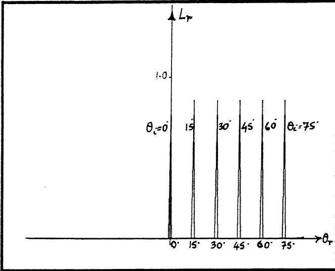
(a) \sigma_h = 0.001 , T = 0.05 , \lambda = 0.5
