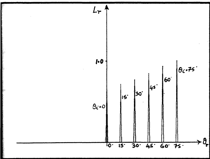
(c) \sigma_h = 0.001 , T = 0.01 , \lambda = 0.02
