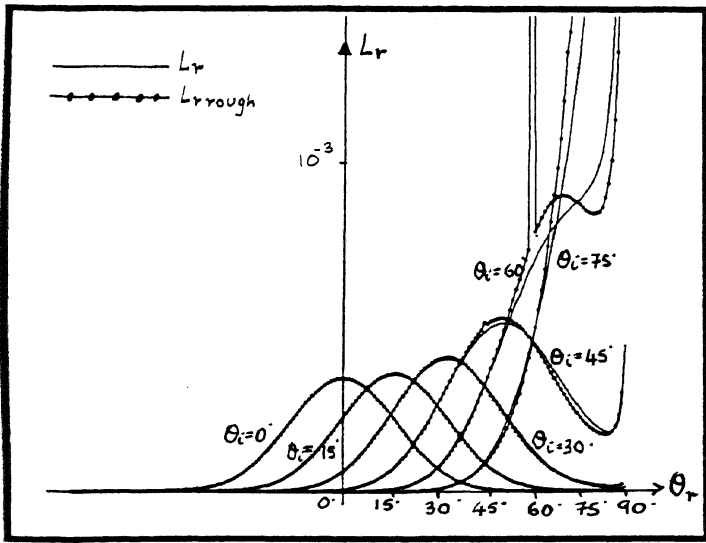
(a) \sigma_h = 0.001 , T = 0.01 , \lambda = 0.0001
