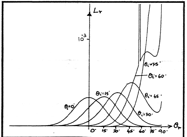
(f) \sigma_h = 0.001 , T = 0.01 , \lambda = 0.002
