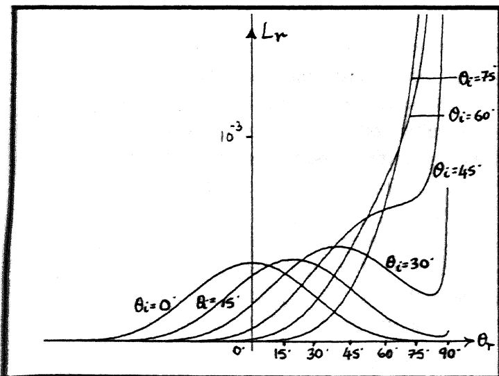
(e) \sigma_h = 0.001 , T = 0.007 , \lambda = 0.0001
