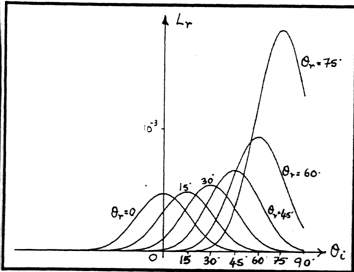
(c) \sigma_h = 0.001 , T = 0.01 , \lambda = 0.001
