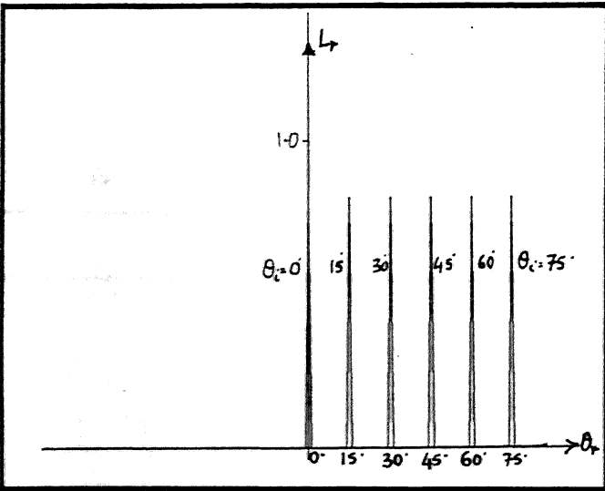
(c) \sigma_h = 0.001 , T = 0.01 , \lambda = 0.5
