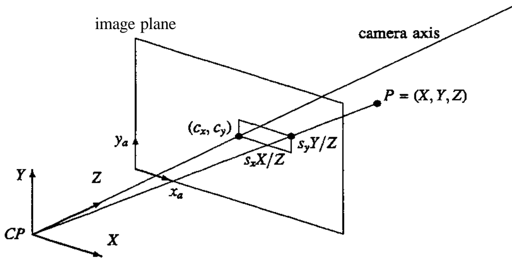
Figure 2: Camera model
