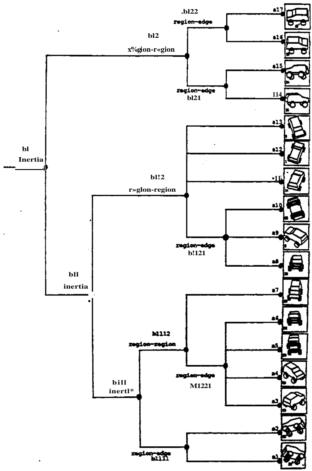
Figure 3: Interpretation tree for a toy wagon
