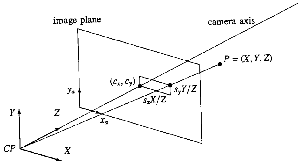
Figure 2: Camera model
