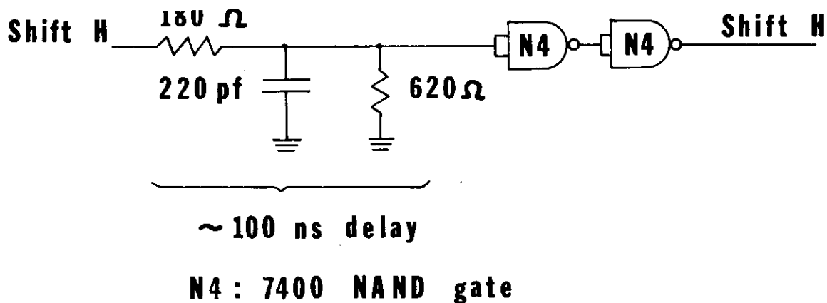
Figure 13. The 100 ns delay
