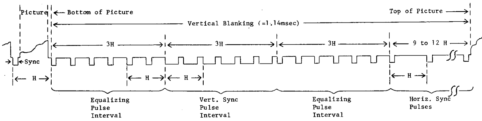
6(a). Composite Video Format
