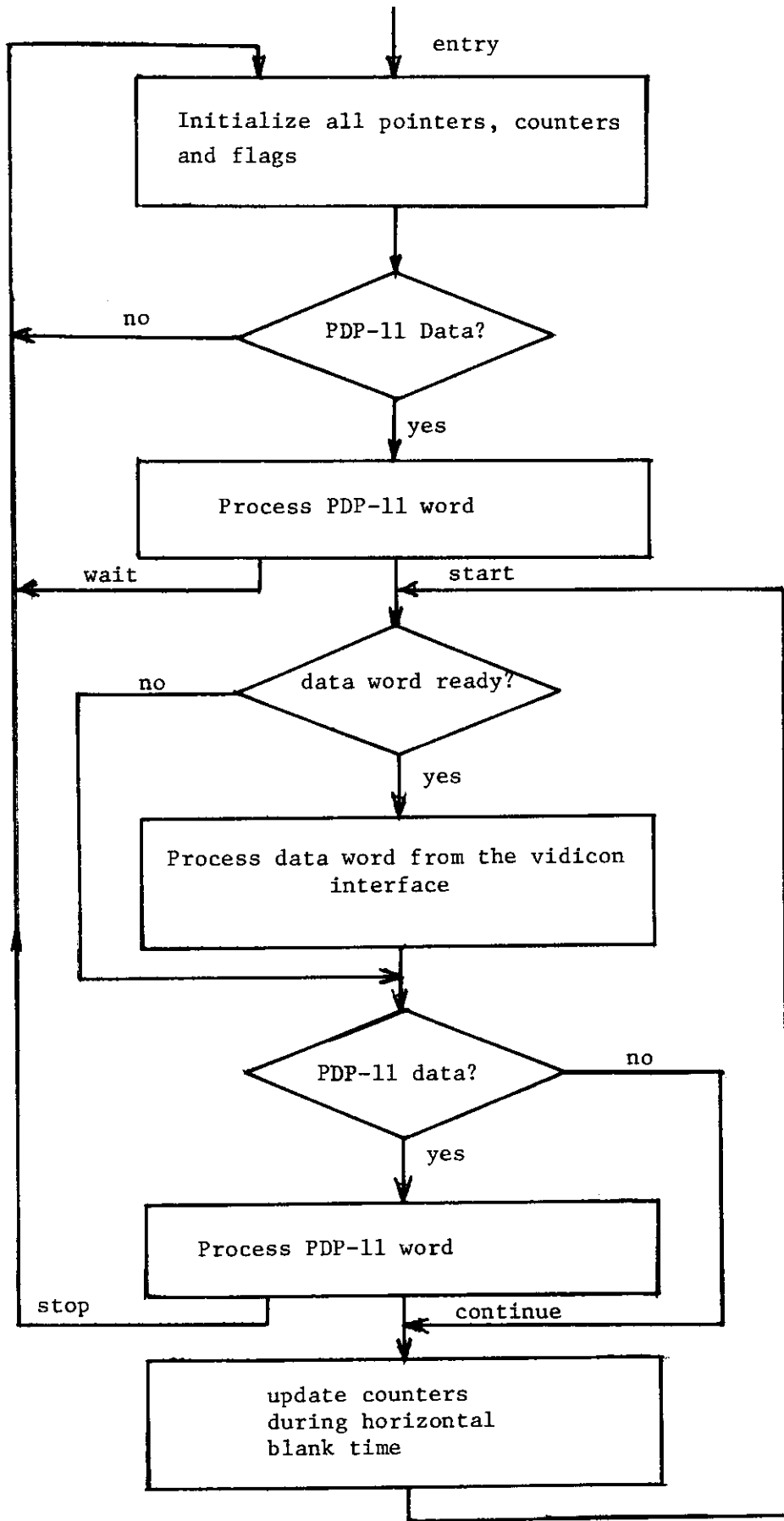
Figure 18. Flow Diagram of Video Processor and Device Interface.
