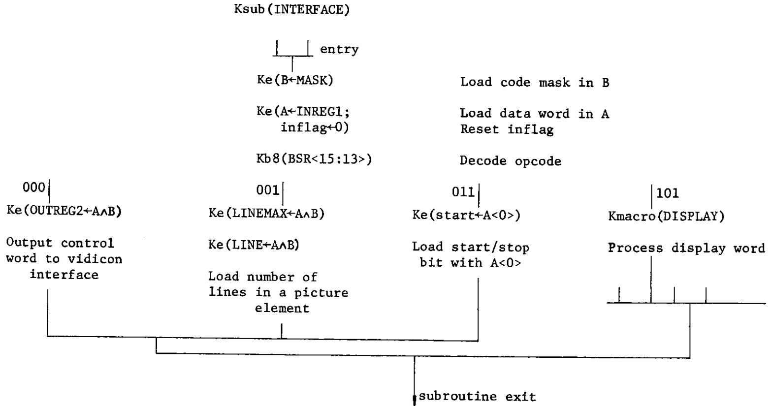
Figure 20. RTM Subroutine INTERFACE
