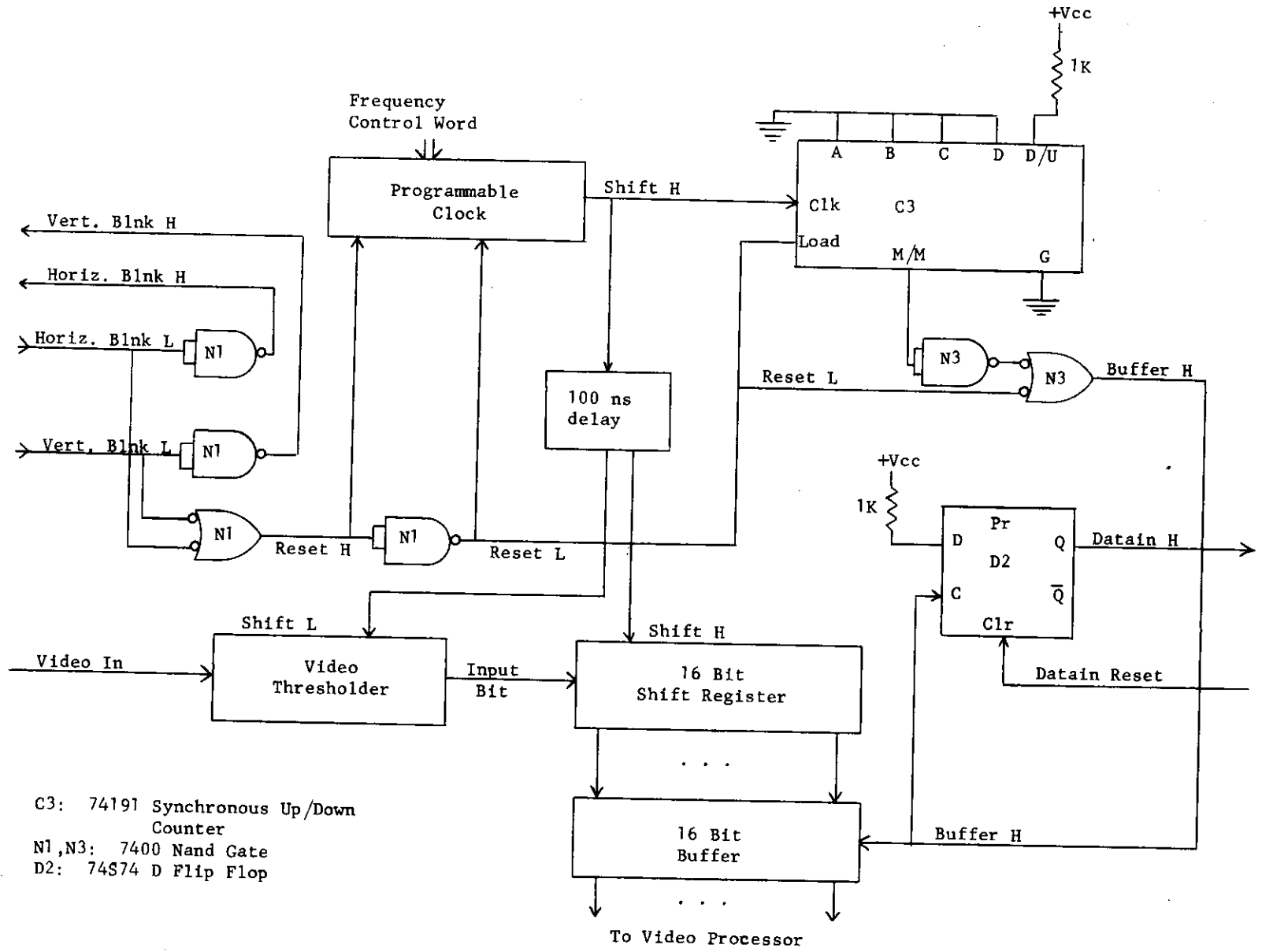
Figure 10. Diagram of Vidicon Interface
