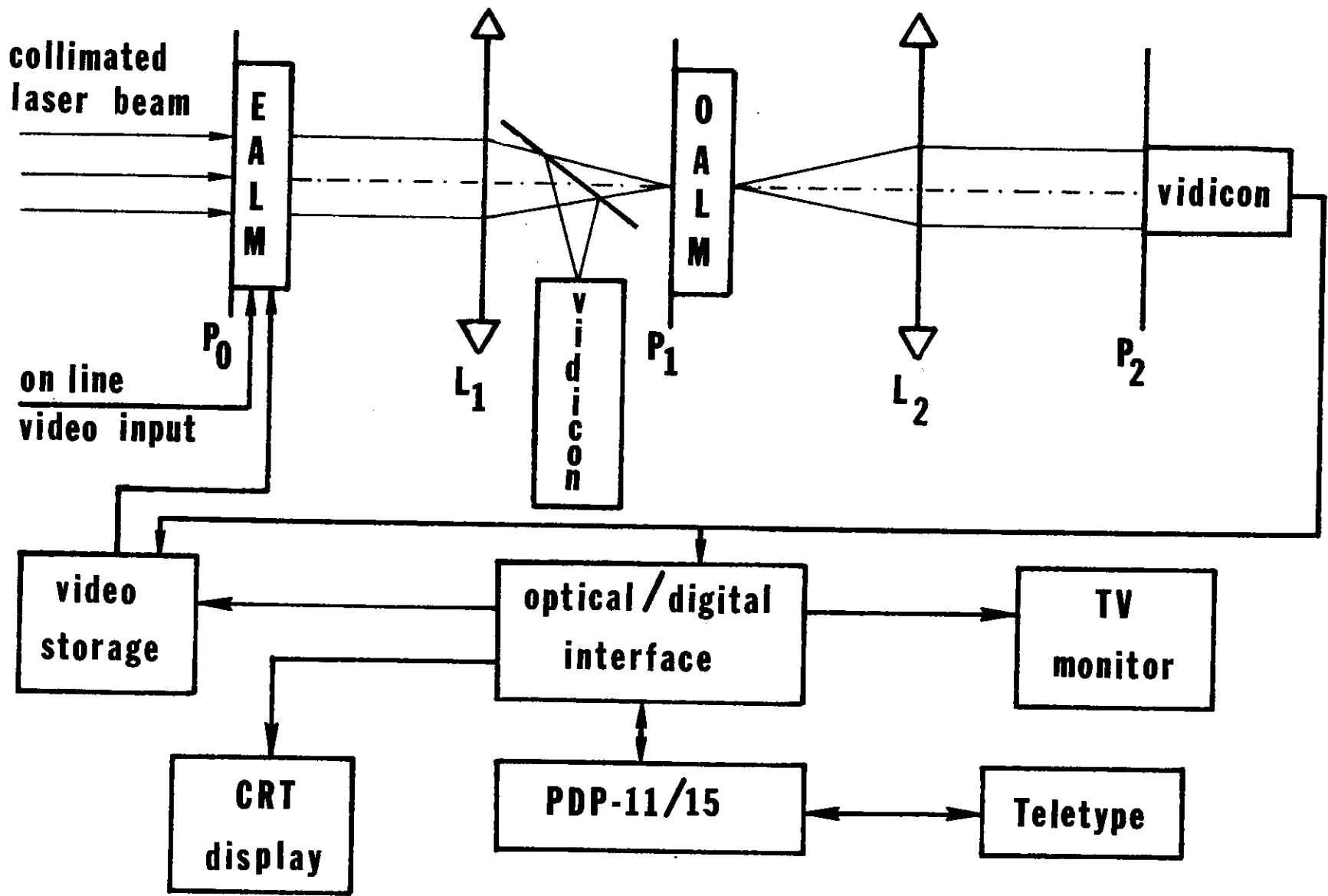
Figure 1. The hybrid optical/digital processor system. For simplicity, only the data paths for the output plane ( P_2 ) vidicon are shown. Paths for the Fourier transform plane ( P_1 ) vidicon are identical. The P_1 plane is viewed via a beam splitter.
