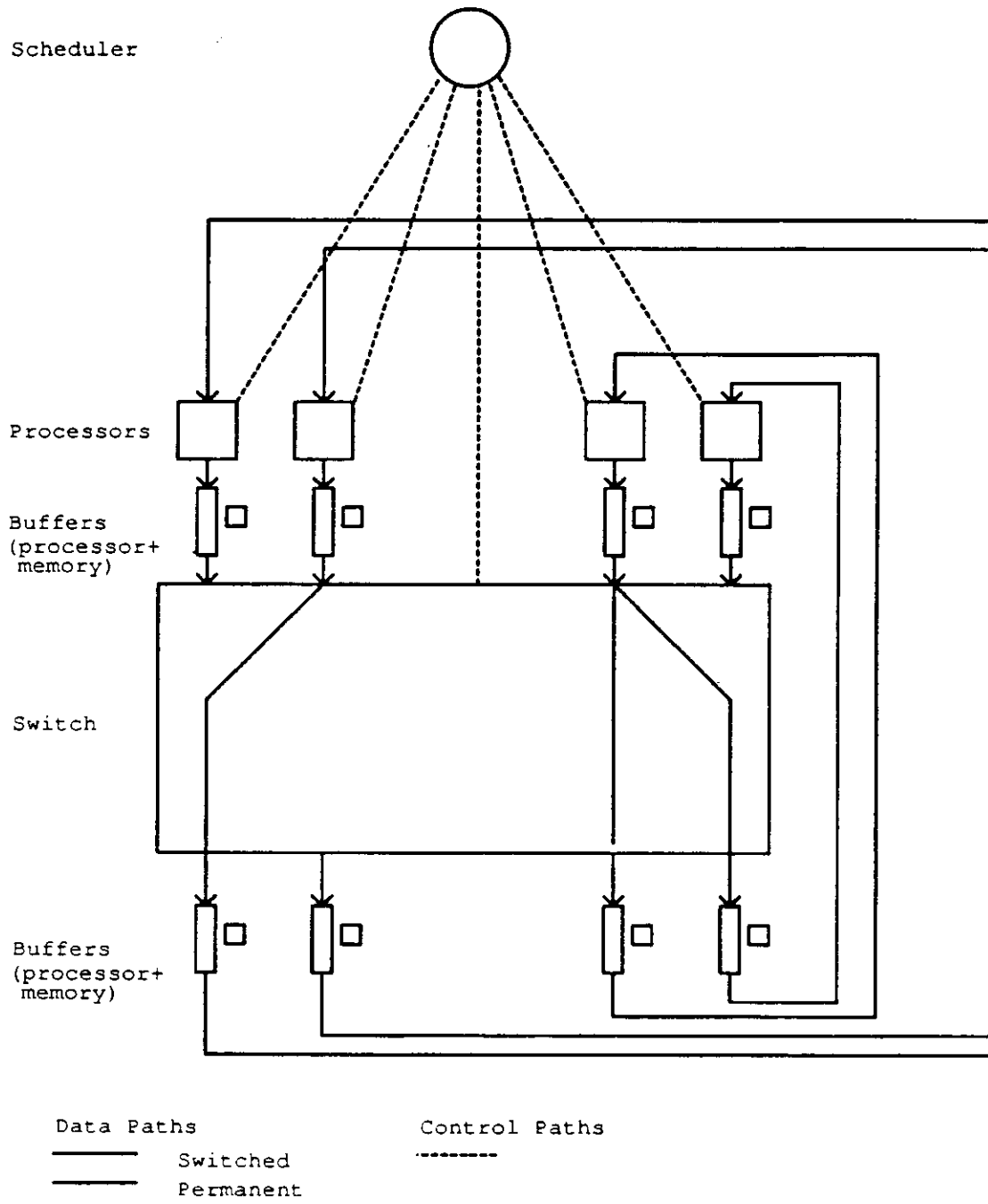
Figure 1 -- Physical Components
