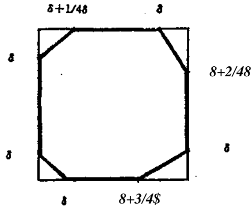
Figure 2*4: The constructed polygon.
