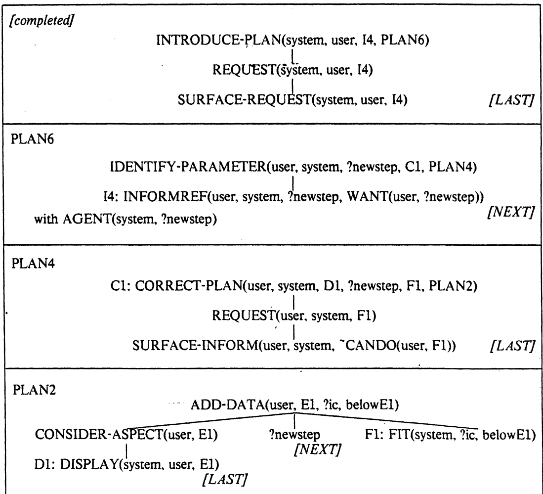
Figure 4.16: If the System had Prompted
