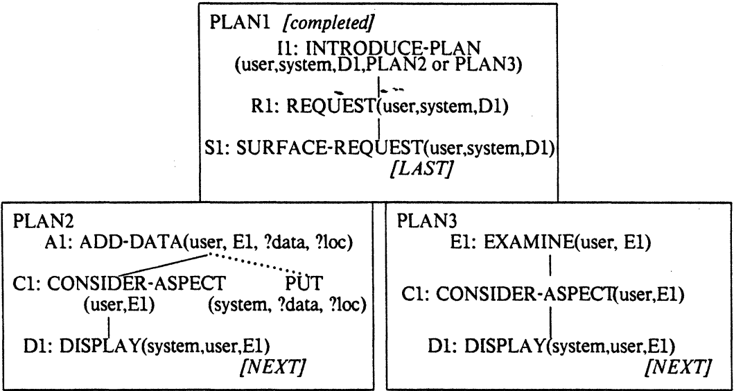
Figure 6.7: The Need for Multiple Sets of Assertions
