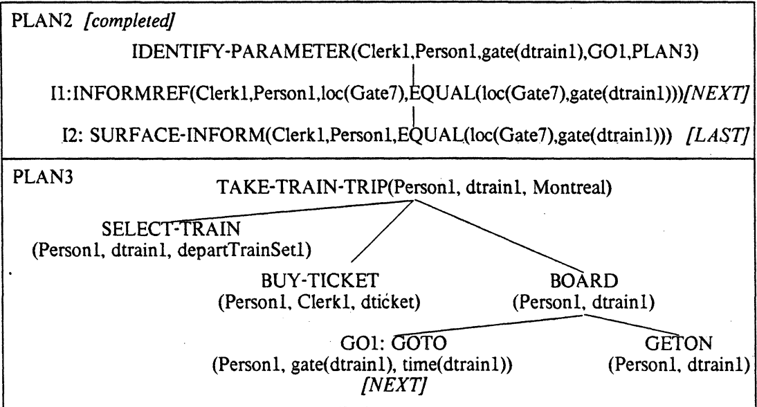
Figure 4.7: The Plan Stack after the Clerk's Response
