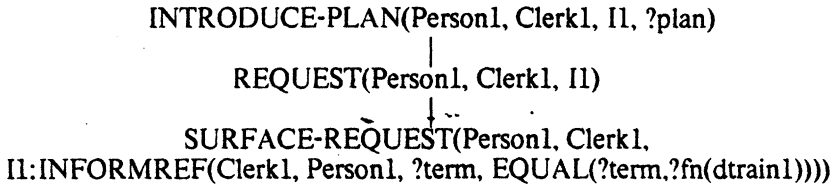
Figure 4.3: Chaining Produces an Intermediate Plan Recognition Structure
