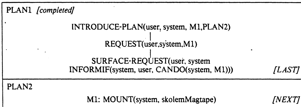
Figure 5.2: The Plan Stack After the First Utterance
