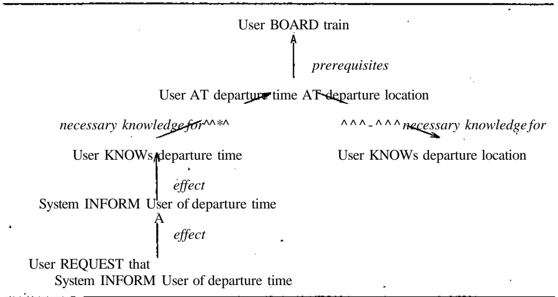
Figure 7.1: Plan Recognition and Helpful Behavior
