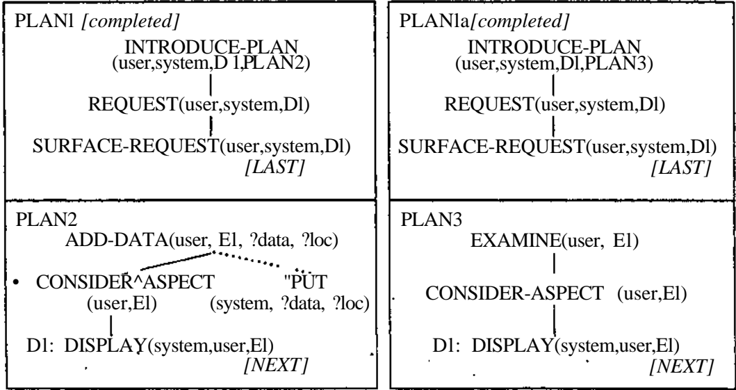
Figure 4.12: The Two Plan Stacks after the First Utterance
