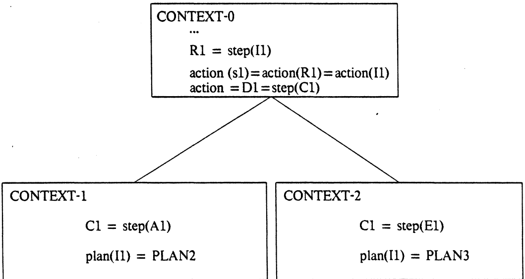
Figure 6.8: An Example Equality Context Tree with Inheritance
