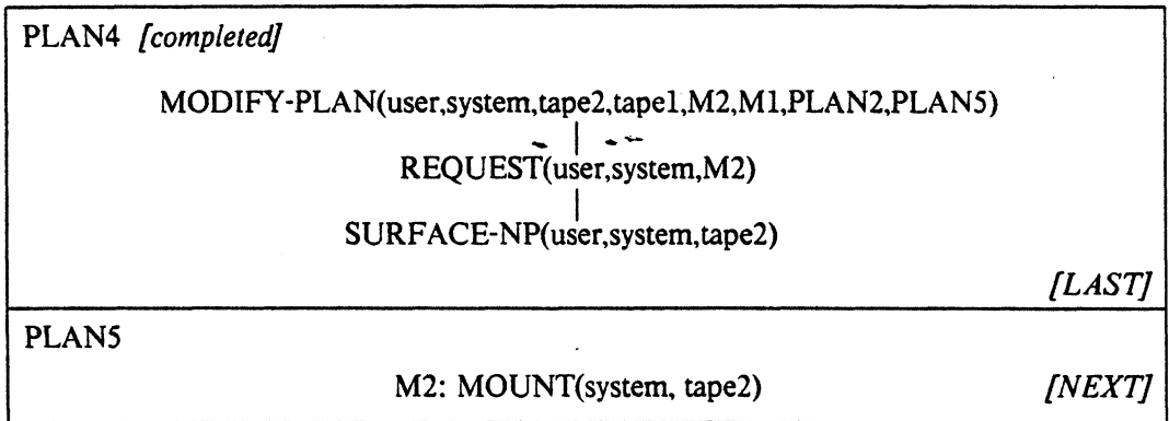
Figure 5.4: The Modified Plan Stack
