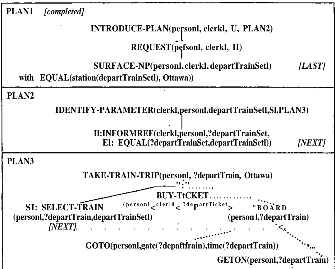
Figure 5.6: The Stack after the Initial Fragment
