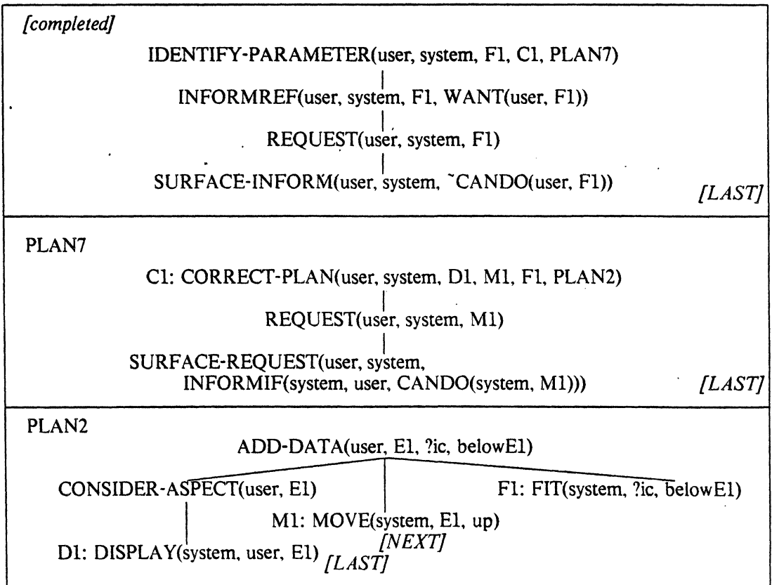
Figure 4.17: If the User's Utterances were Reversed
