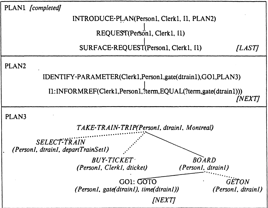
Figure 4.6: The Plan Stack after the First Utterance
