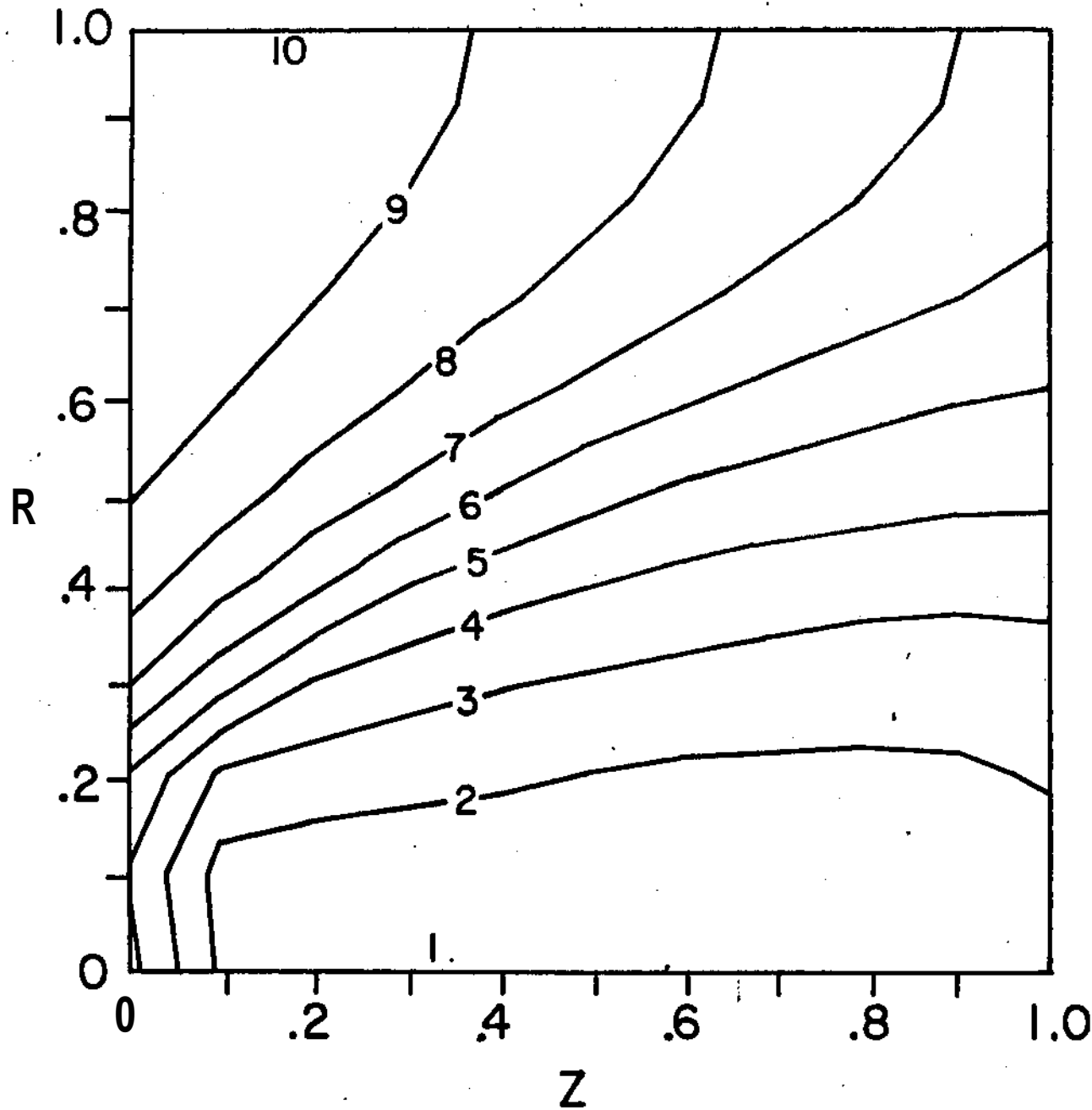
FIGURE 9. TEMPERATURE CONTOURS (CIRCULAR LINE SOURCE CASE; T-3.5)
