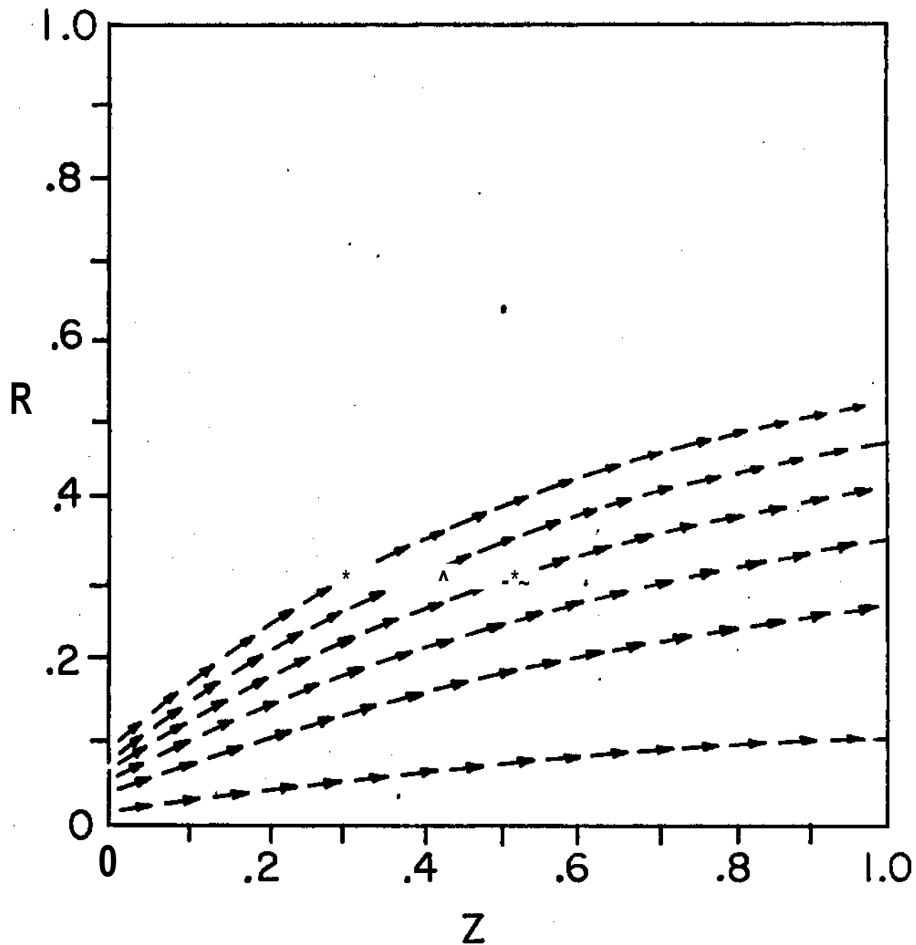
FIGURES. DROPLET VELOCITY VECTOR (BASE CASE; TIME • 3.0)
