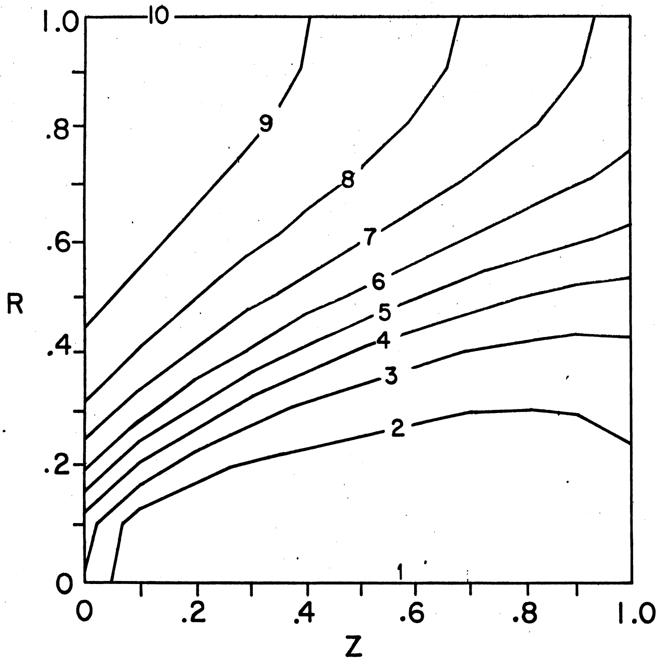
FIGURE 3. TEMPERATURE CONTOURS (BASE CASE; TIME = 3.0, STEADY STATE)
