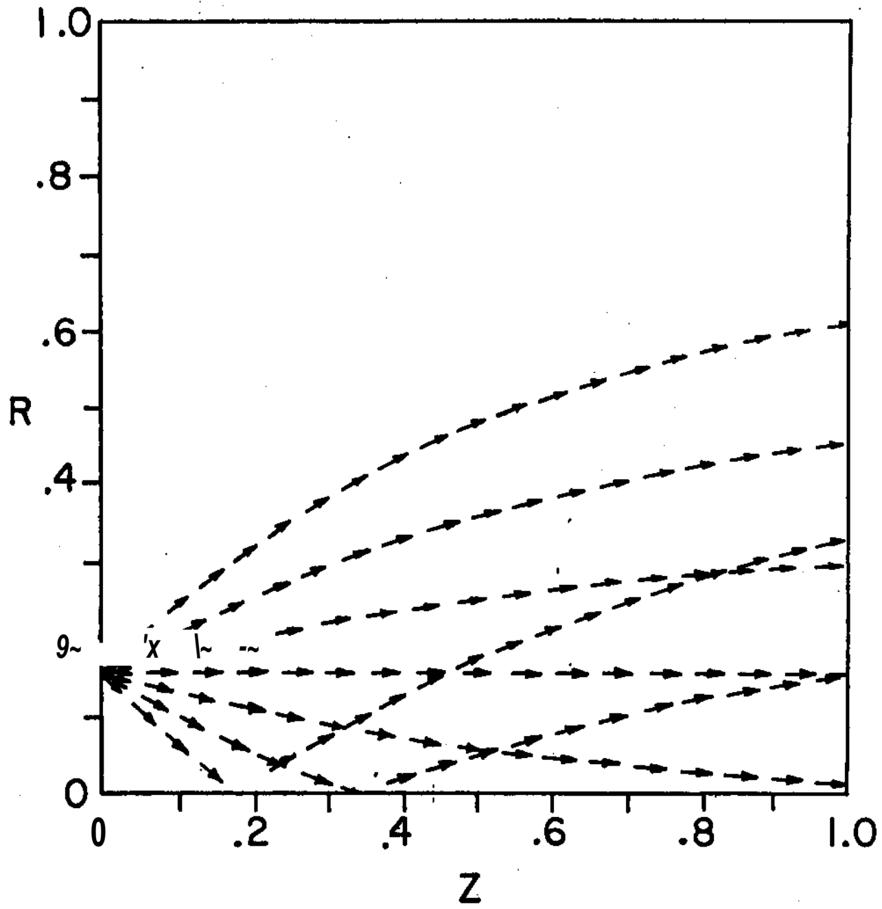
FIGURES. DROPLET VELOCITY VECTOR (CIRCULAR LINE SOURCE CASE; T = 3.5 , STEADY STATE)
