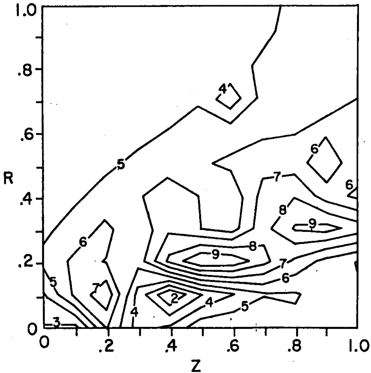
FIGURE 6. TEMPERATURE DIFFERENCE CONTOURS (NORMALIZED CHANGE, 3 CHARS. VS. 6CHARS.; TIME • 3.0)
