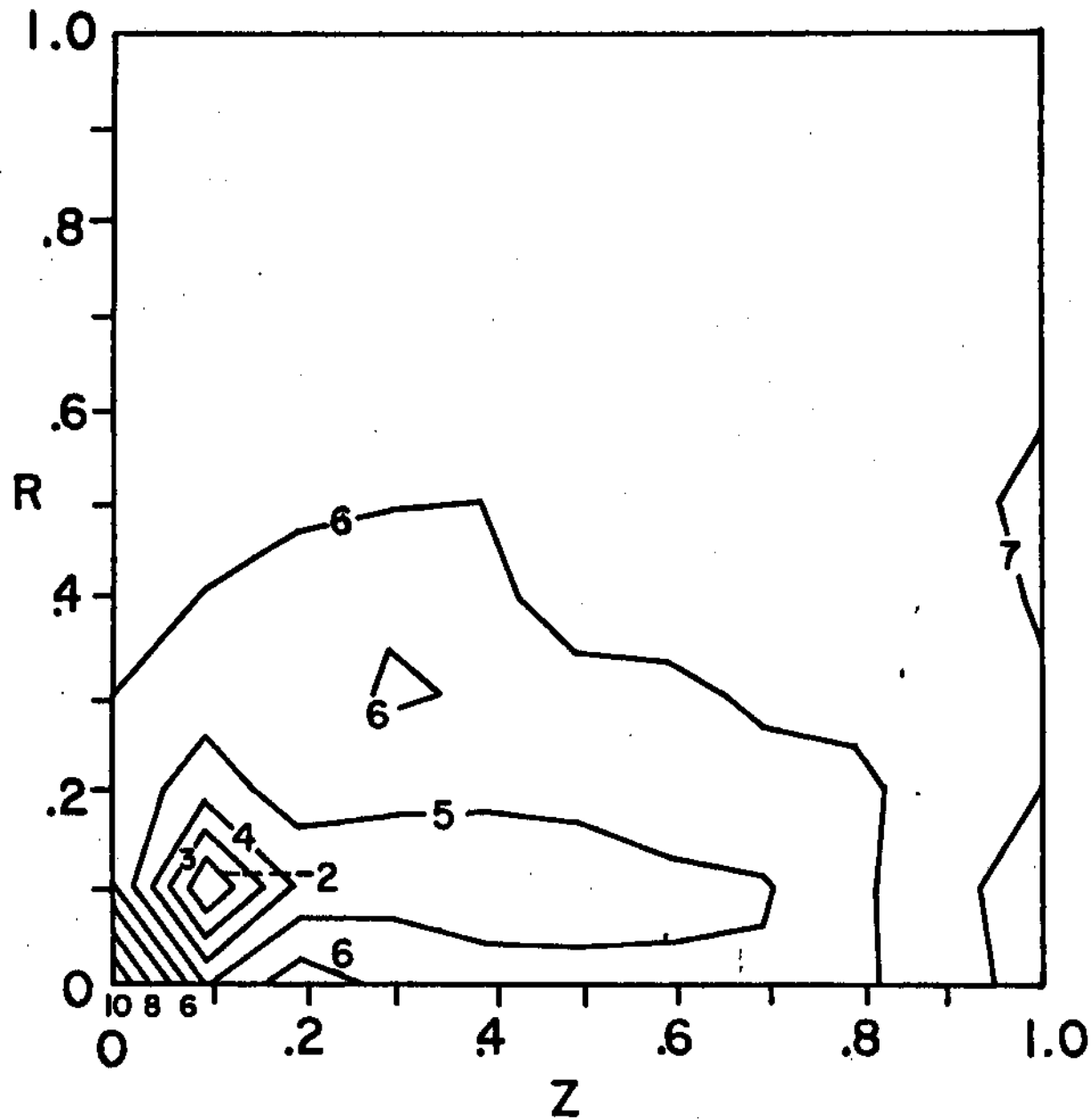
FIGURE 7. TEMPERATURE DIFFERENCE CONTOURS (NORMALIZED CHANGE, 10x 10 GRID VS. 20x20grid; TIME • 3.0)
