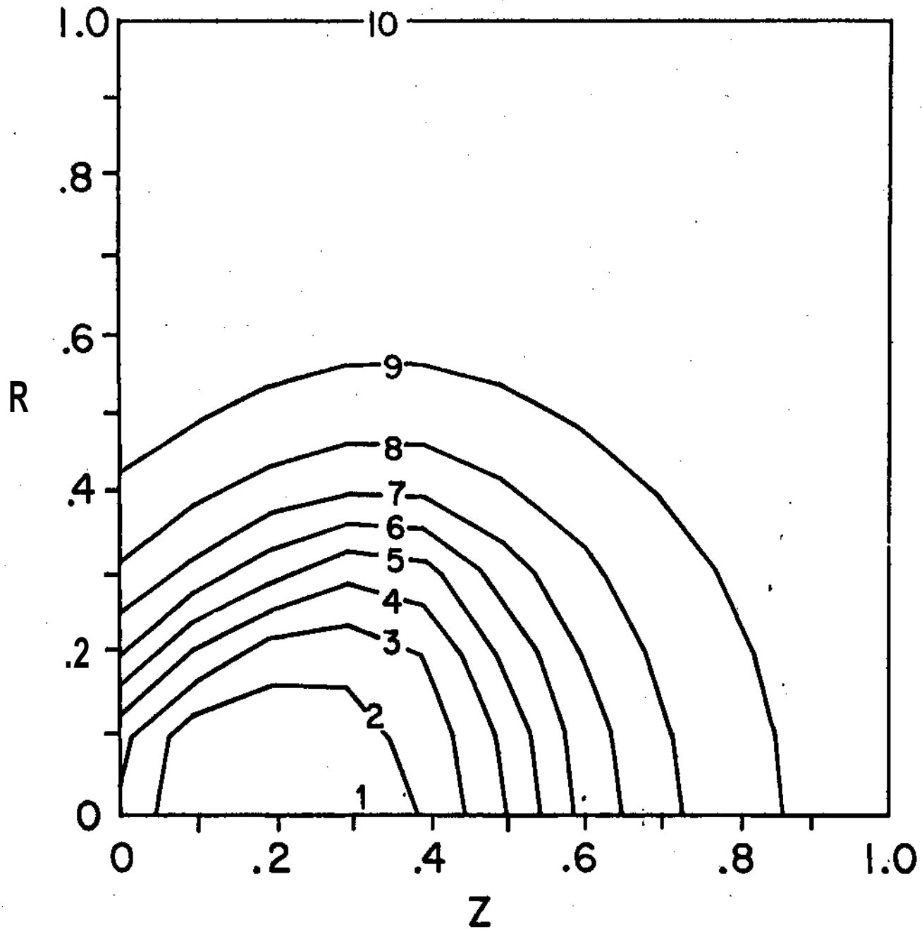
FIGURE 2. TEMPERATURE CONTOURS (BASE CASE; TIME - 0.5)
