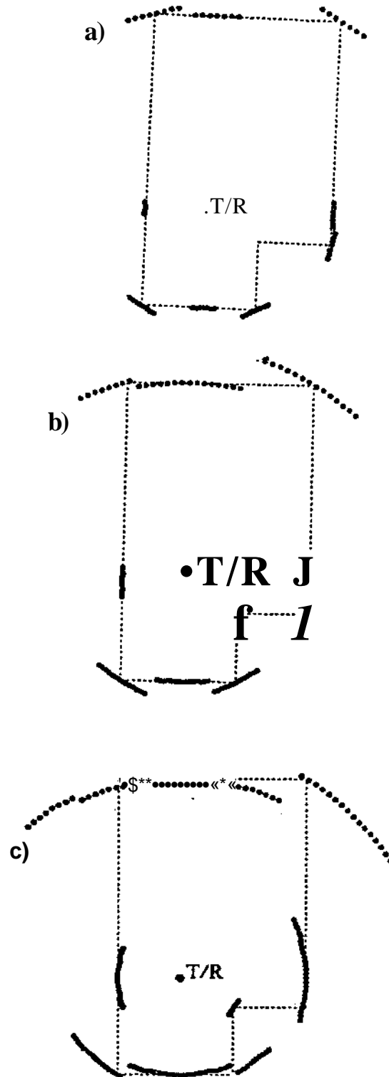
Figure 13: Sector sonar maps of CEWO using three different threshold settings: a) -20 dB, b) -40 dB, and c) -60 dB (relative to wall reflection).
