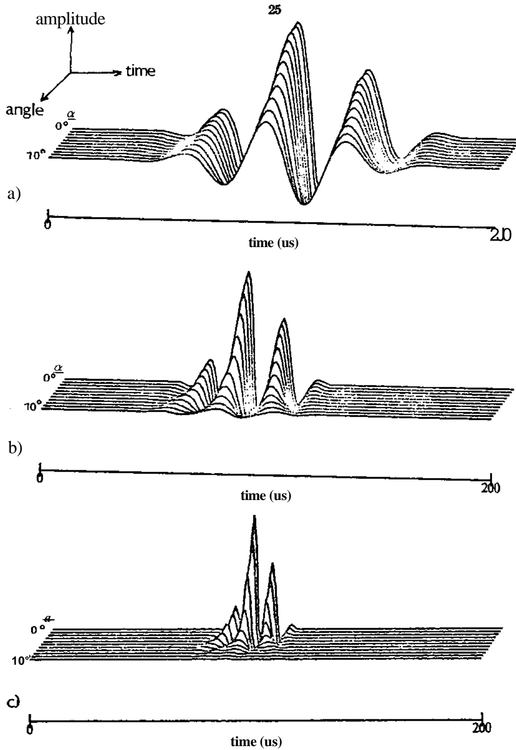
Figure 11: Convolution of pulse waveforms with T/R pair impulse response shown in Figure 7: a) 30 KHz, b) 60 KHz, c) 120 KHz.
