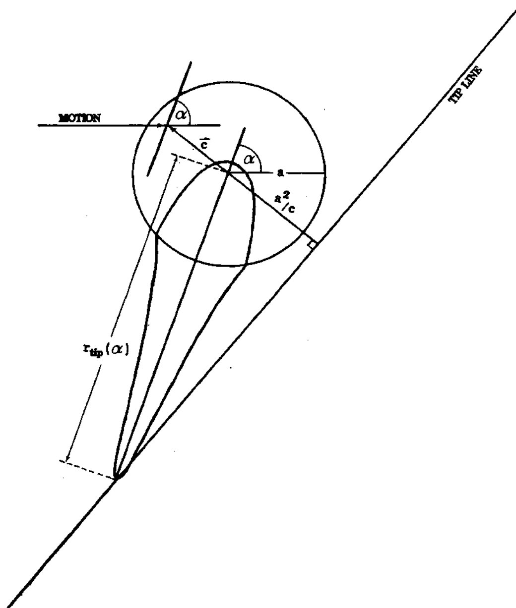
Figure 2-3: r_{np}(a) vs. ct_f and construction of the tip line
