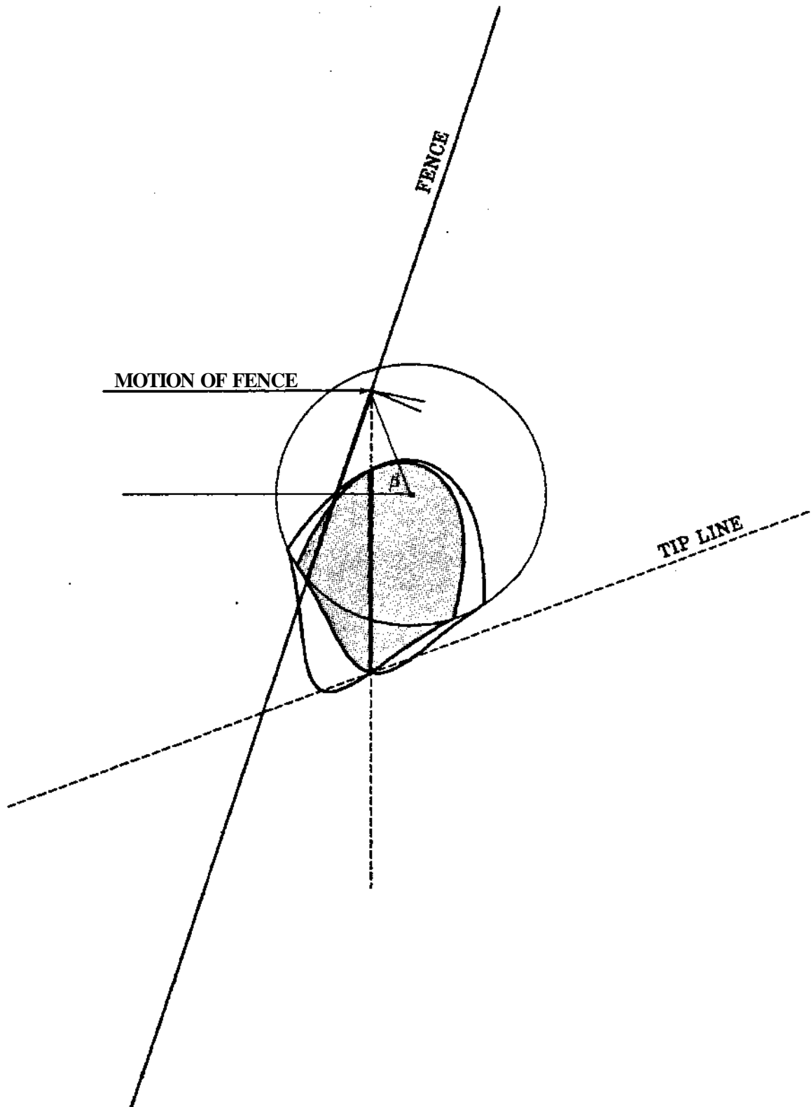
figure 4-3: Transition from sticking-iowest to sipping-lowest behavior
