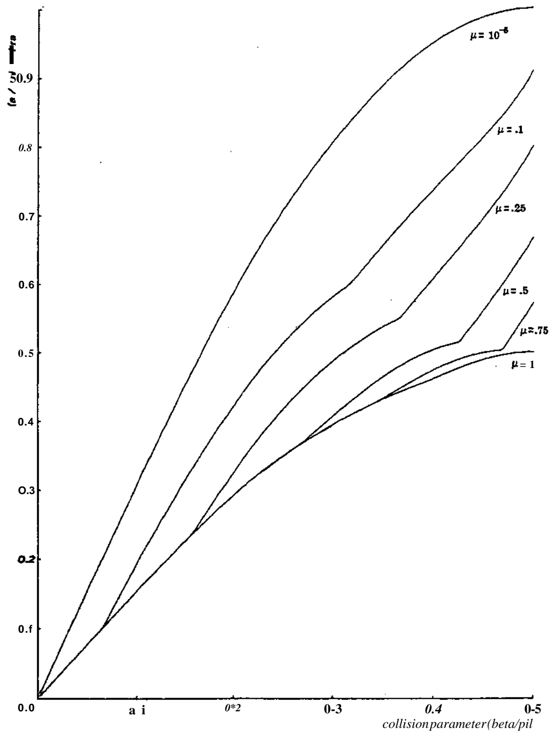
Figure 6-4: Radius r^*(J) of the critical circle as a function of collision parameter \beta l
