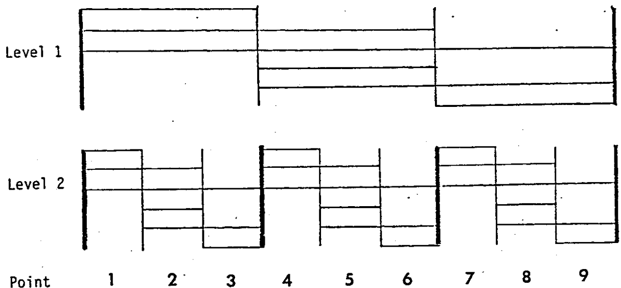
Figure 3.4 A 2-level 2-range.
