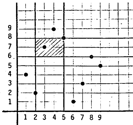
Fig.3.2 Point set F .
