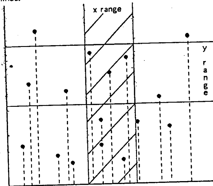
Figure 2.1. Illustration of projection.
