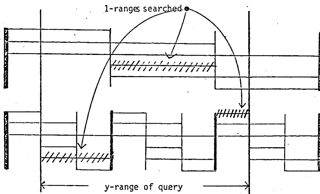
Figure 3.5 Querying a 2-level 2-range.
