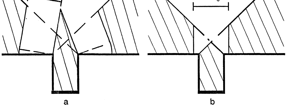
Figure 7. Two subgoals for the peg in hole. These subgoals may seem too big, but the planner can consult the sensors to further refine its idea of the robot's location.
