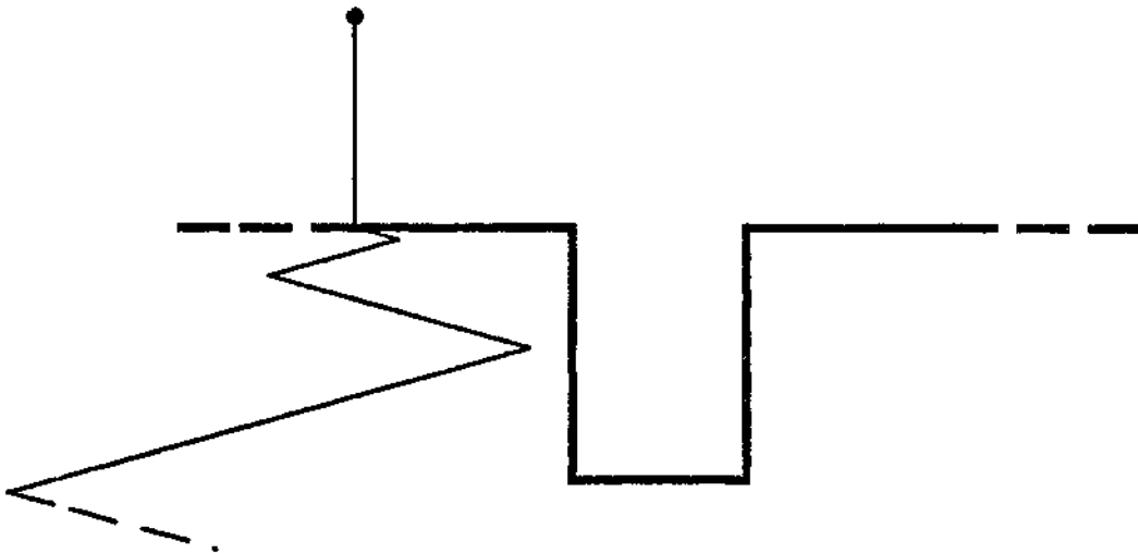
Figure 8. A problem requiring a finite, but unbounded, number of steps; e_c = \infty , e_v = e_g = 0 , l = C . The robot has no position feedback, and has no idea whether to search to the left or the right for the hole. In order to find the hole, the robot must sweep back and forth, in an ever-enlarging search. Such a plan must succeed eventually, but there is no upper bound on the number of motions.
