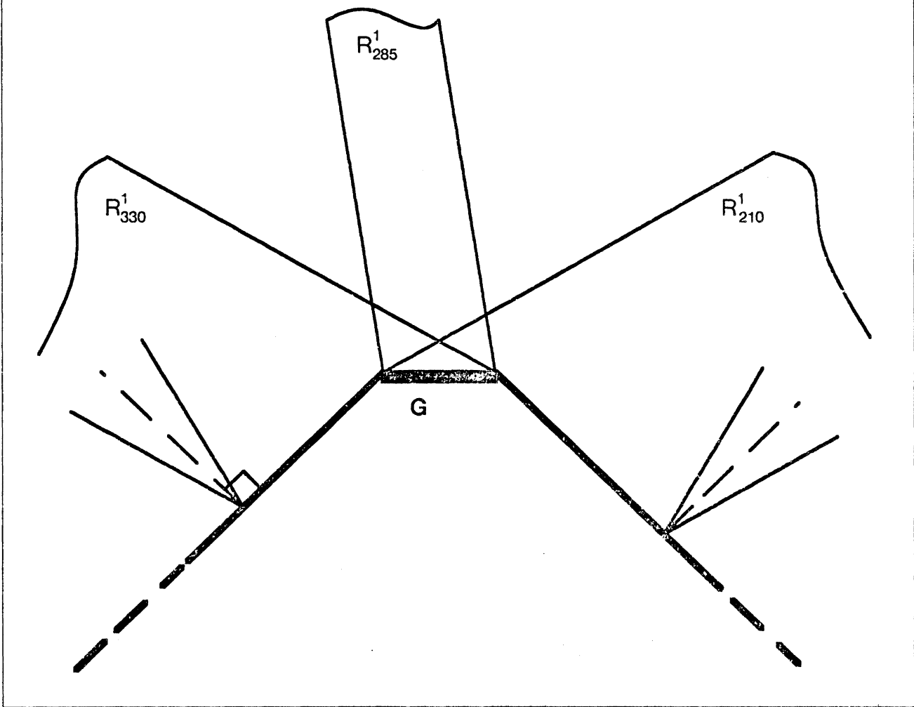
Figure 8a. The point-on-hill problem; \epsilon_c = \infty , \epsilon_v = \epsilon_s = 0 , I = C . Since the robot has no position feedback, it must rely on contact with the hill. A simple strategy is to proceed downwards until contact. If the robot tends to the left at termination, it can move up to the right to attain the goal. Otherwise it should move up to the left. The backtracking variation cannot solve this problem; since it considers only one subgoal at a time, it cannot derive an either-or strategy. The best subgoal chain that the backtracking variation can construct is shown through three levels, after which no improvement is possible. (a) shows typical convergence regions at the first level. The best single subgoal is R_{210}^1 , which is passed to the second level.
