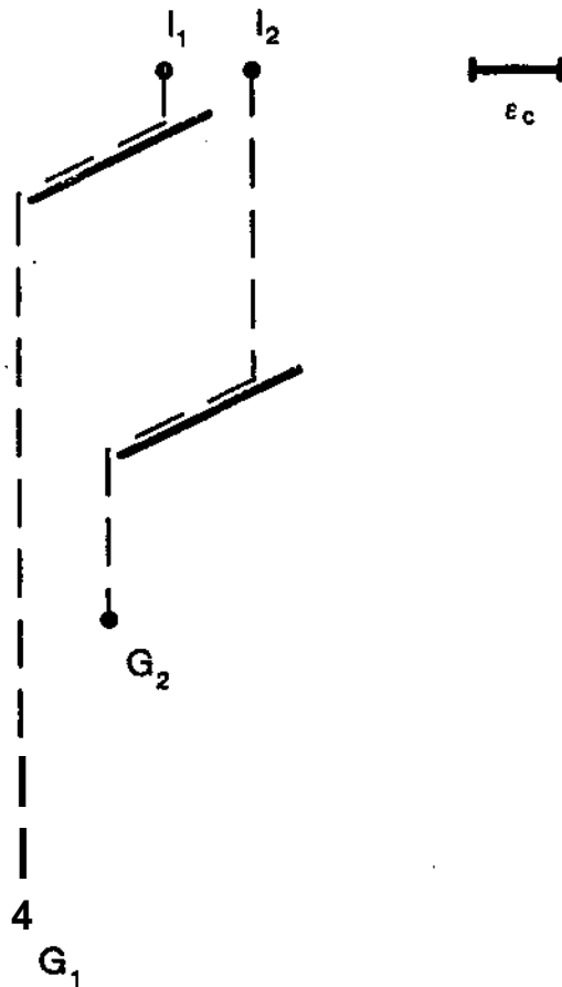
Figure 9. A problem exposing the deficiency of the stateless predicate; e_c is shown, e_v = e_a = 0 , l_1 = l_2 ( J^2 > G = G \setminus J ) ( 2 < \dots ). Solution of this problem with a single motion requires a decision to terminate based on sensory information obtained earlier in the motion. The memoryless predicate requires two motions in the worst case.
