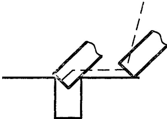
Figure 1, Two fine-motion strategies, (a) illustrates the value of tilting a peg before attempting to insert it in a hole. A comparable error causes failure without tilting, and success with tilting, (b) illustrates the use of the biased search. The peg is deliberately brought down to one side of the hole. This reduces or eliminates the chance of hitting the hole directly, but improves the chance of sliding into the hole on the second motion, because the direction to the hole is known.
