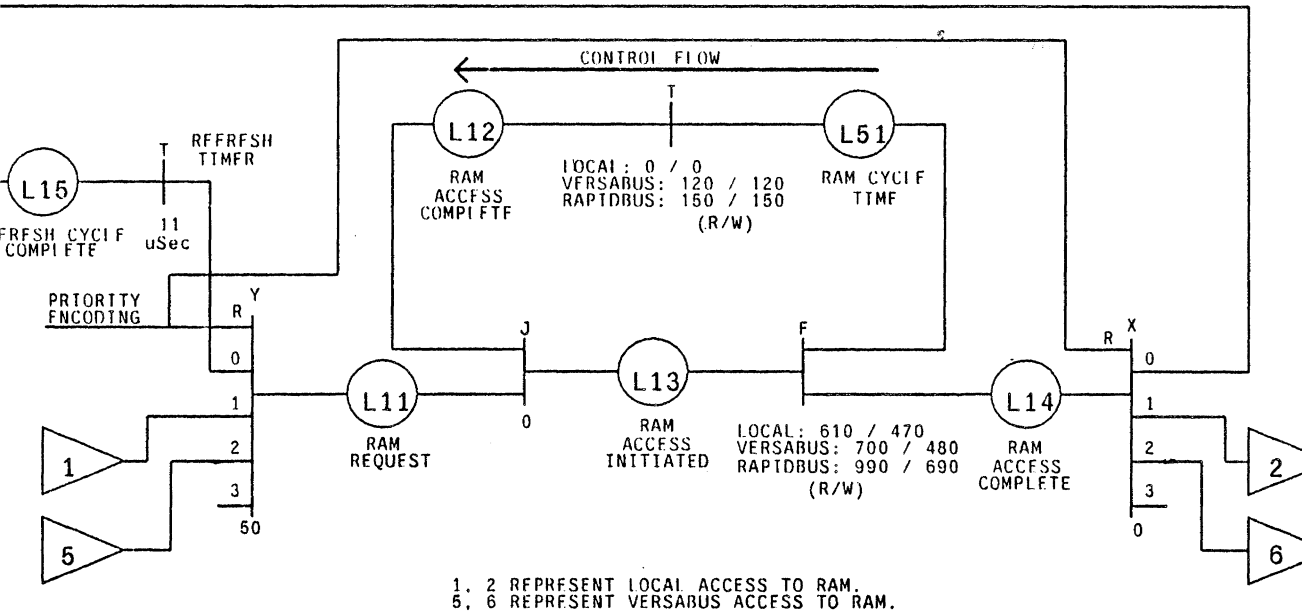
Figure 2-11: The local ram is dual ported to both the Versabus and the local processor bus.
