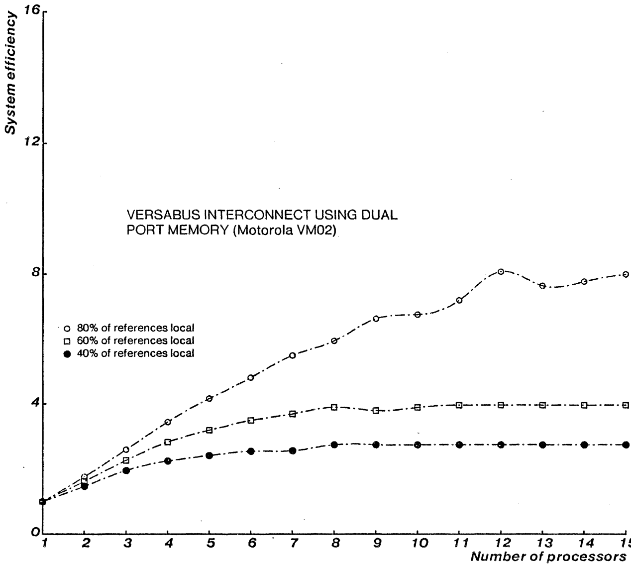
Figure 5-13: Versabus systems quickly saturate in a tightly coupled system such that increasing the number of processors does not improve the throughput.
