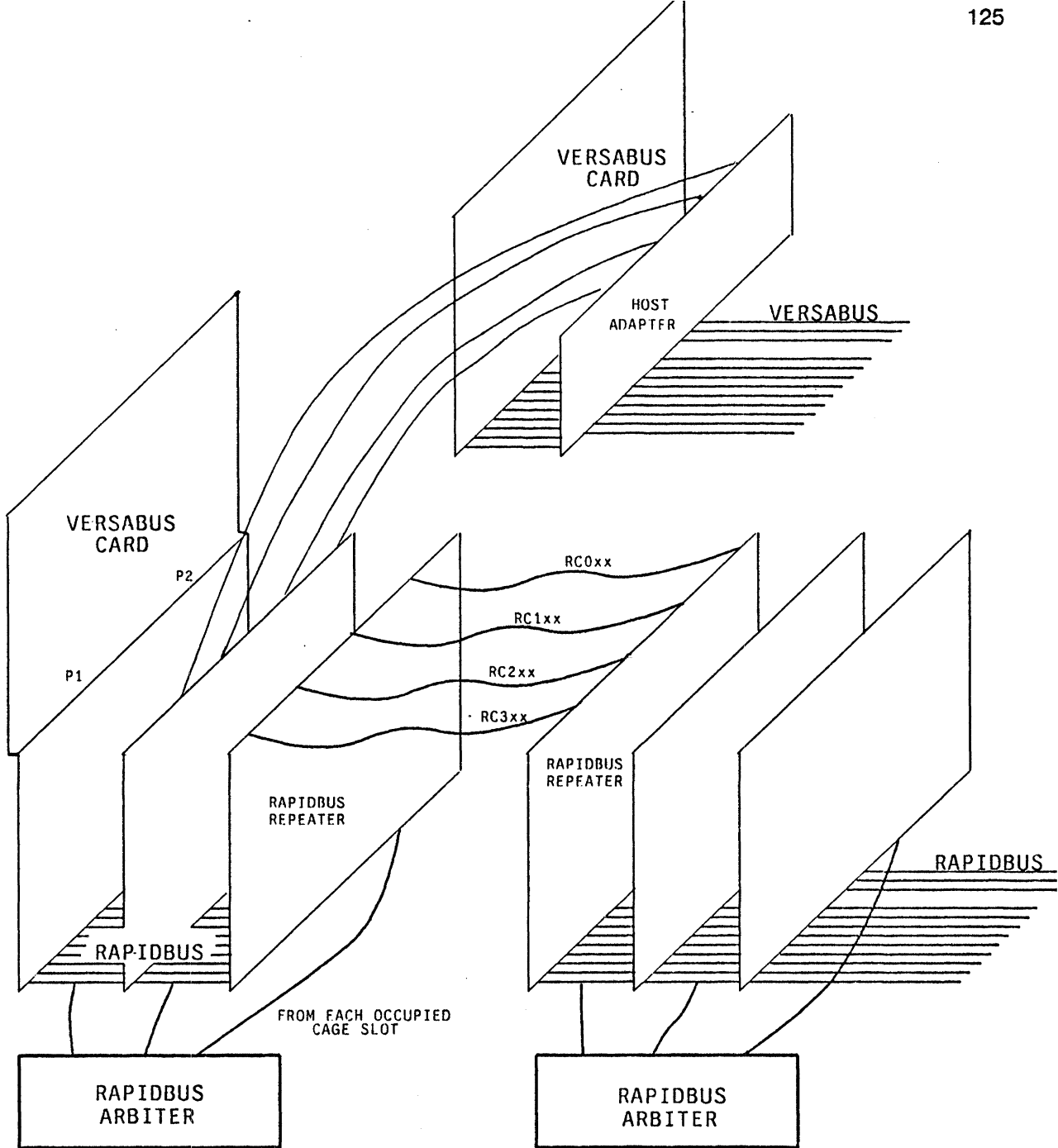
Figure 5-11: RAPIDbus II proof-of-concept realization.
