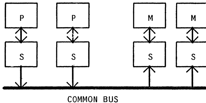
Figure 2-3: Separation of processor and memory functions on the bus maximizes bus loading and average memory reference latency.
