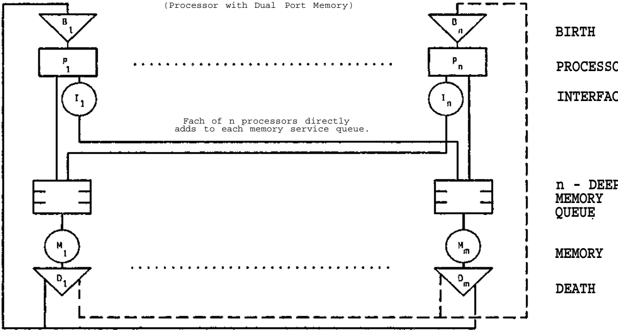
Figure 3-11: Addition of a RAPIDbus interface to a dual port Versabus system decreases bus contention while introducing the possibility of deadlock.
