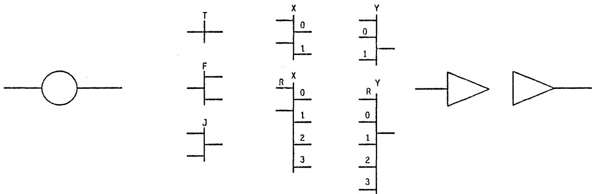
Figure 2-9: Locations and transitions are used to represent control flow using evaluation net notation.
