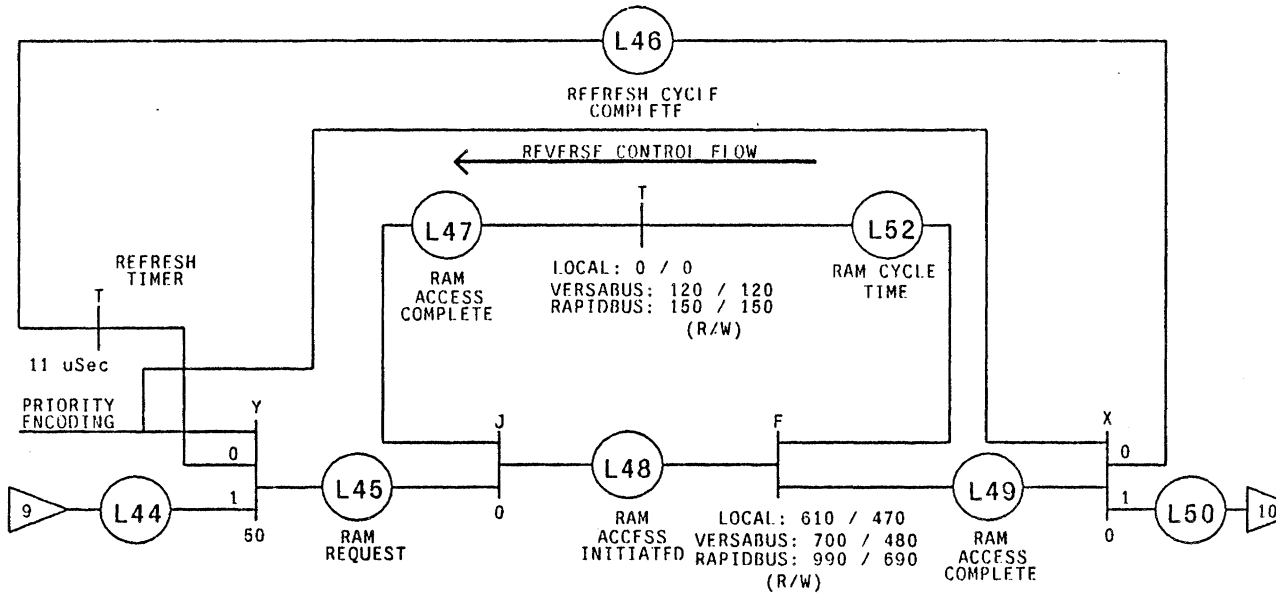
Figure 2-13: System memory cards resemble VM02 ram cards without the dual-port arbitration.
