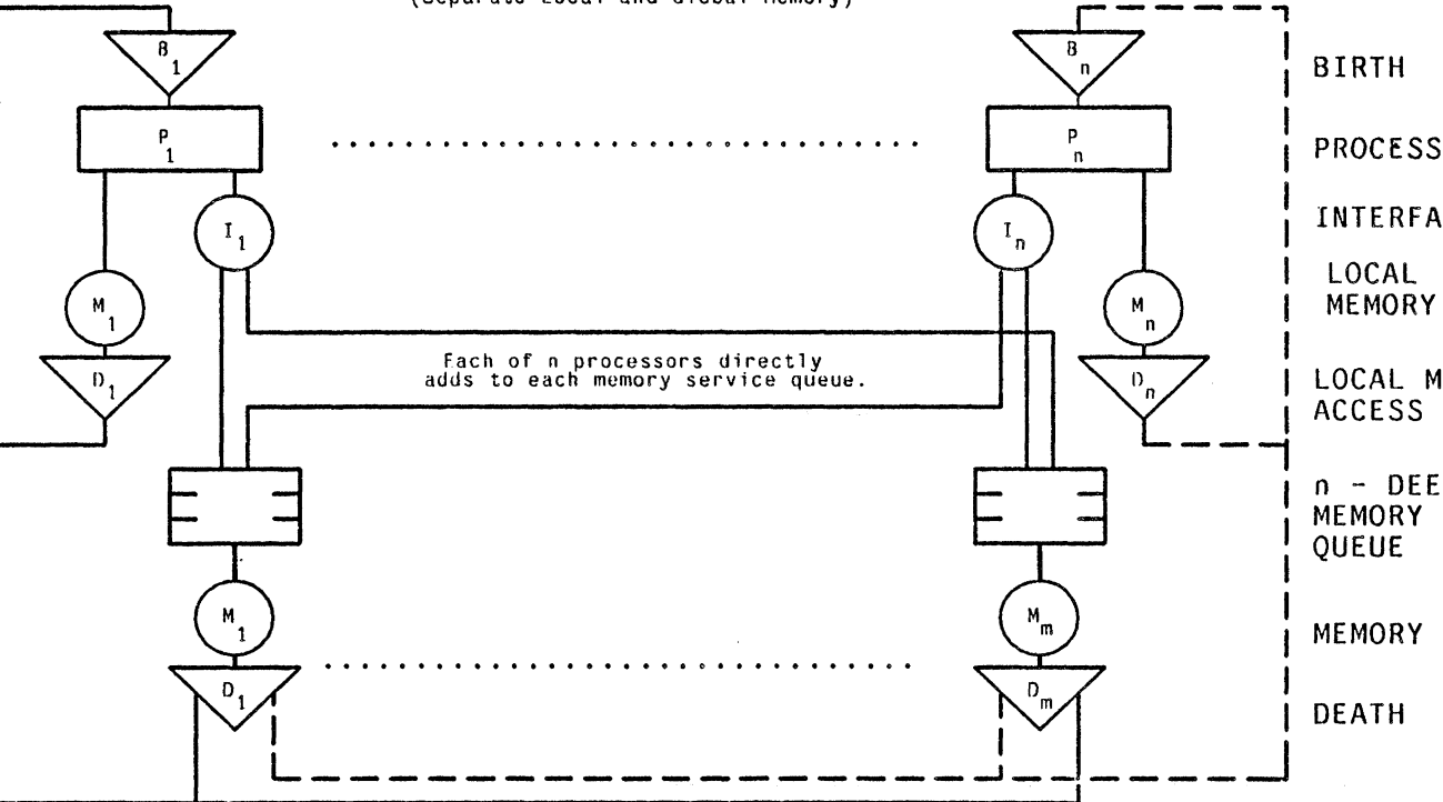
Figure 3-7: Addition of RAPIDbus interfaces to a Versabus system with local memory removes bus contention for those references mapped to the system bus.
