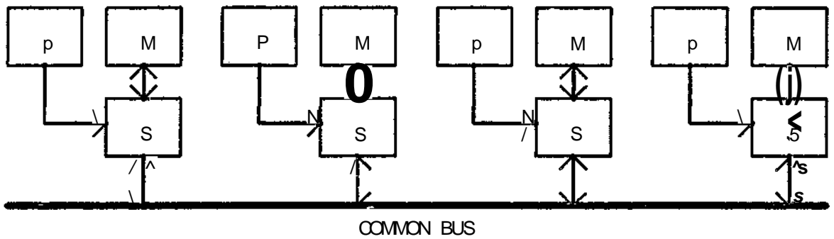
Figure 2-5: Dual porting of the local memory can economize en bus cycles required to access shared memory.
