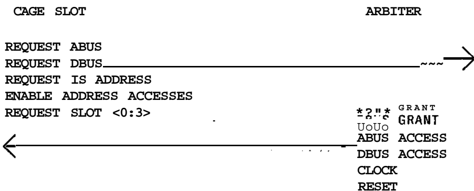
Figure 5-4: Timing for the high speed buses is done by one arbiter module global to each cage.
