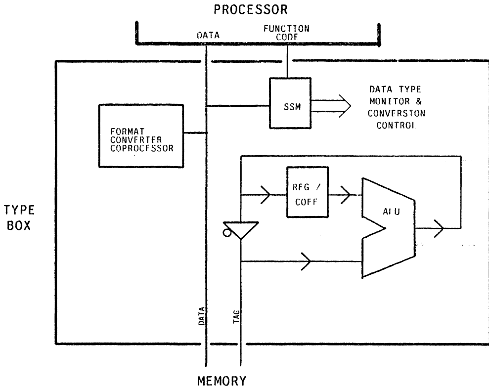
Figure 4-10: The type box is used to retrofit a variety of existing processors to an object based RAPIDbus II.
