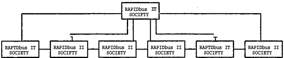
Figure 4-3: A pipeline of societies fits applications where most of the data flow obeys a linear, single input port, single output port relationship.
