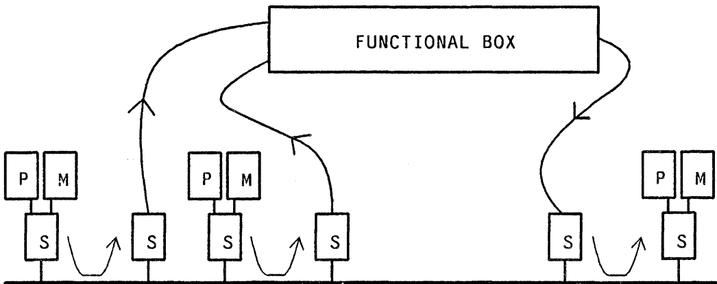
Figure 4-1: Multiword packets can be used to integrate a prototype functional box onto RAPIDbus while existing processors absorb overhead functionality.
