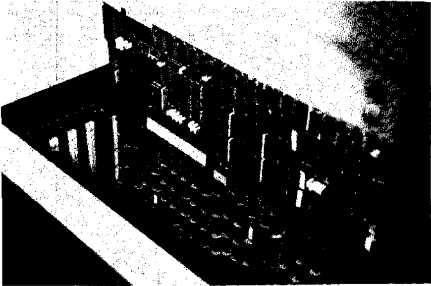
Figure 2-2: The RAPIDbus I interface was implemented on a mother-daughter board inserted between the physical bus and a commercial monoboard computer.
