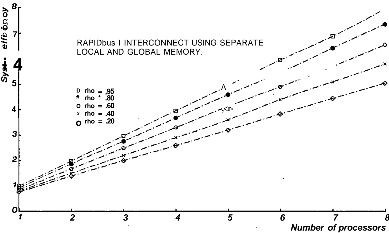
Figure 3-8: Addition of RAPIDbus interface cards decreases contention for the system bus, improving performance in systems with low p and more than three processors.
