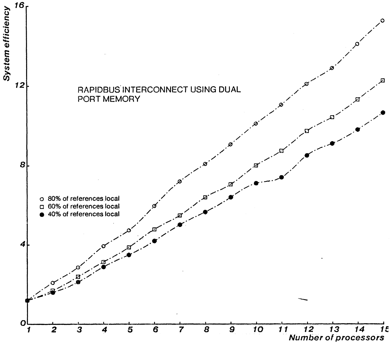
Figure 5-14: Use of a RAPIDbus II interchange network significantly reduces bus contention in a tightly coupled application with respect to a similar Versabus system.
