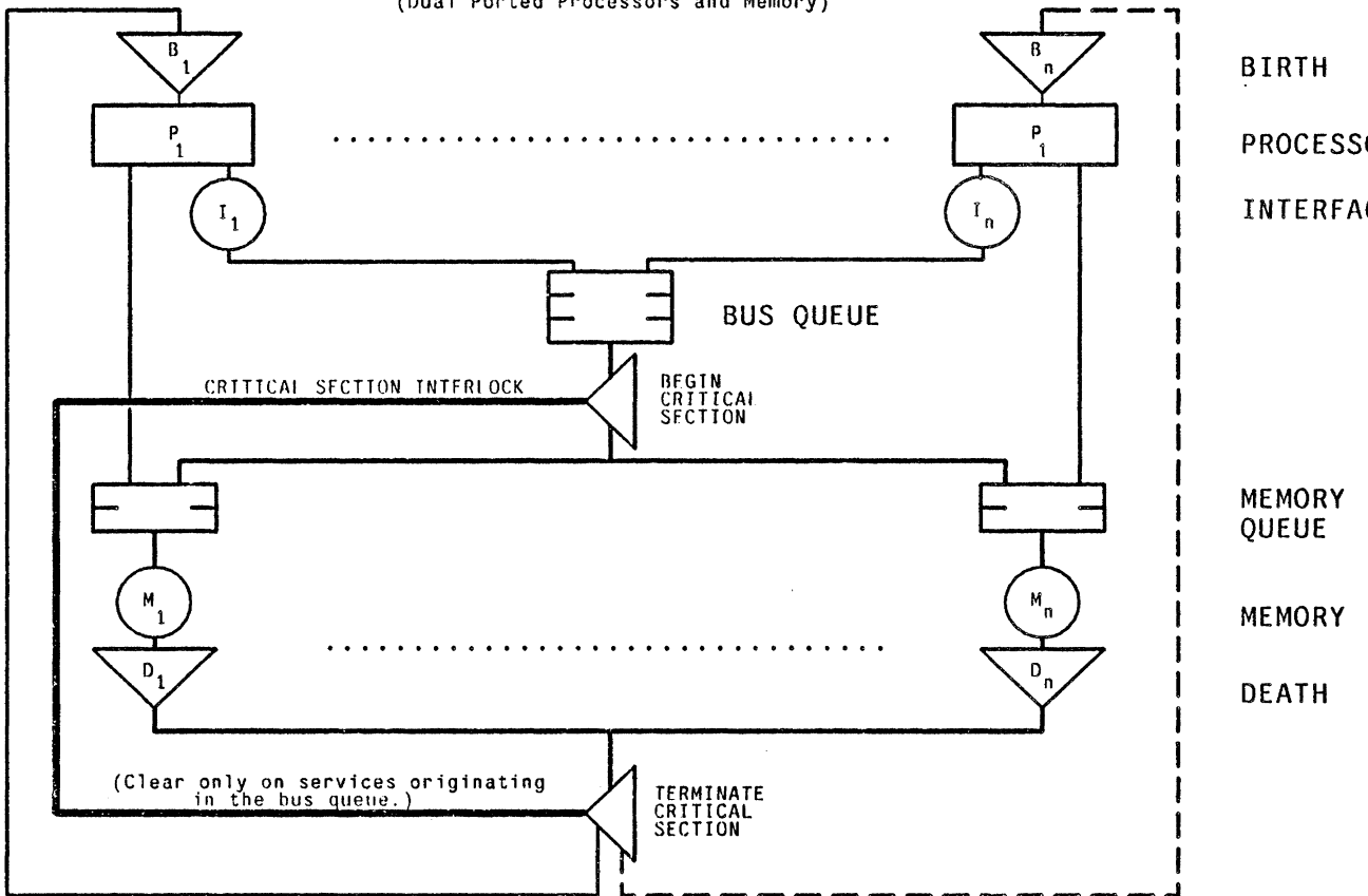
Figure 3-9: Dual porting the local memory to the system bus decreases bus contention relative to separate memory cards without the disadvantages of purely local memory.
