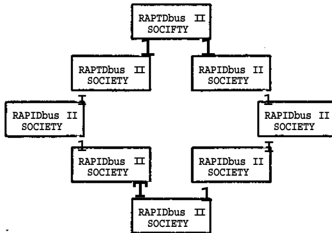
Figure 4-4: A ring of societies provides low latency communication throughout the address space with singly redundant paths between societies.
