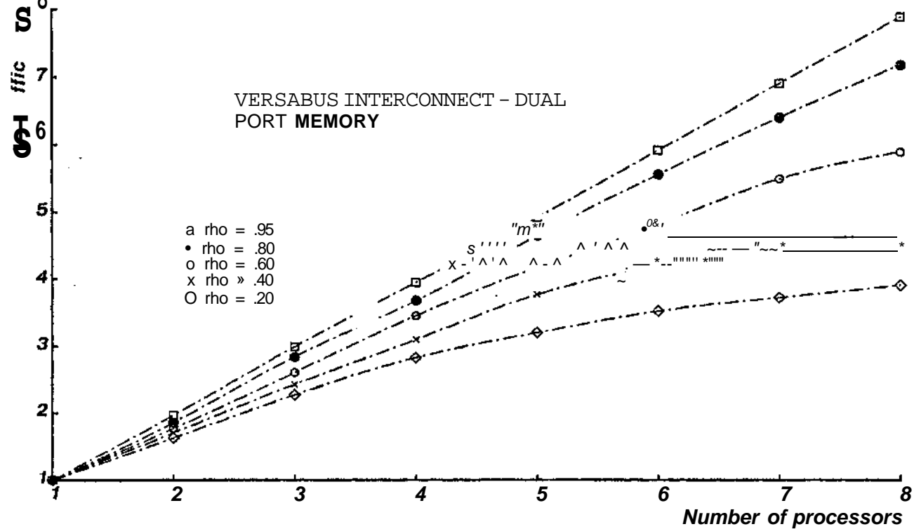
Figure 3-10: Dual porting the memory local to the processor decreases bus contention and simplifies restarting a suspended process.
