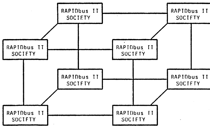
Figure 4-5: Rings of societies can be generalized into N-cube topologies, with arbitrarily many redundant paths between societies at the price of increased overhead.
