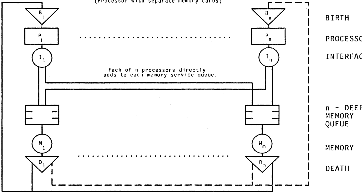
Figure 3-3: Addition of the RAPIDbus interface to a Versabus system with separate processors and memory removes the critical section enveloping bus memory.
