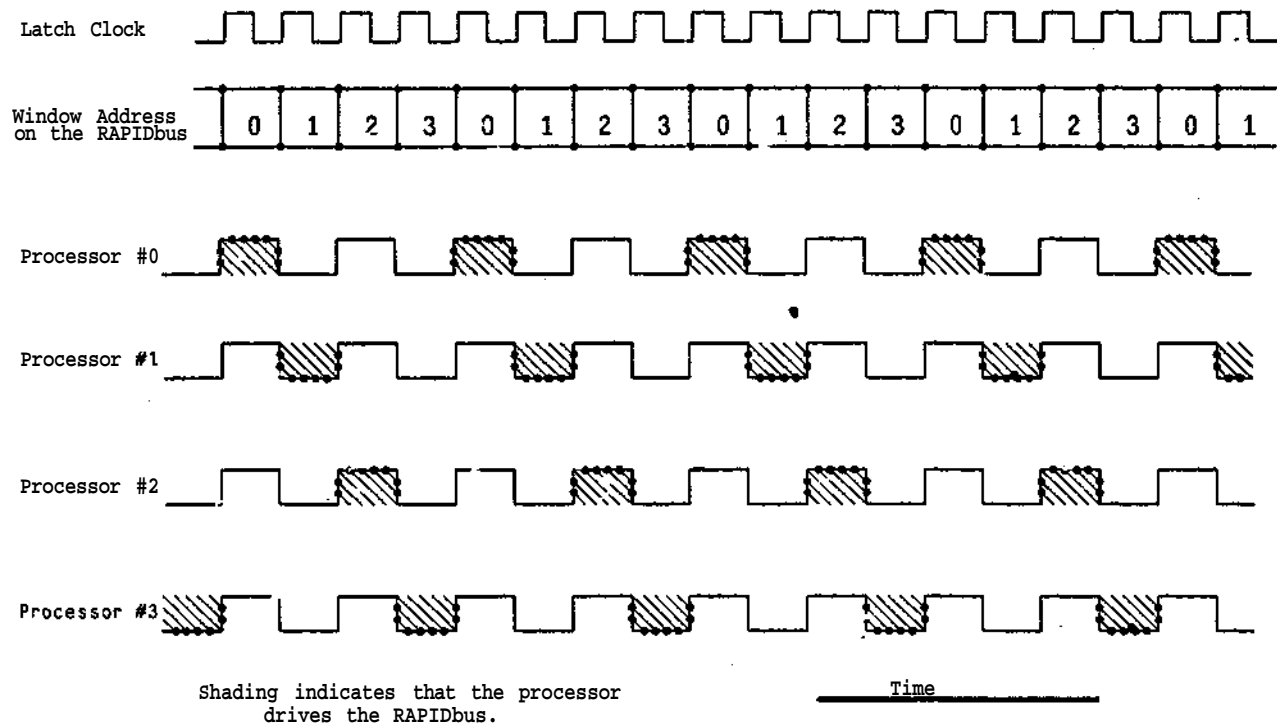
Figure 2-6: The virtual bus system is implemented using bus windows to link several masters and slaves simultaneously.
