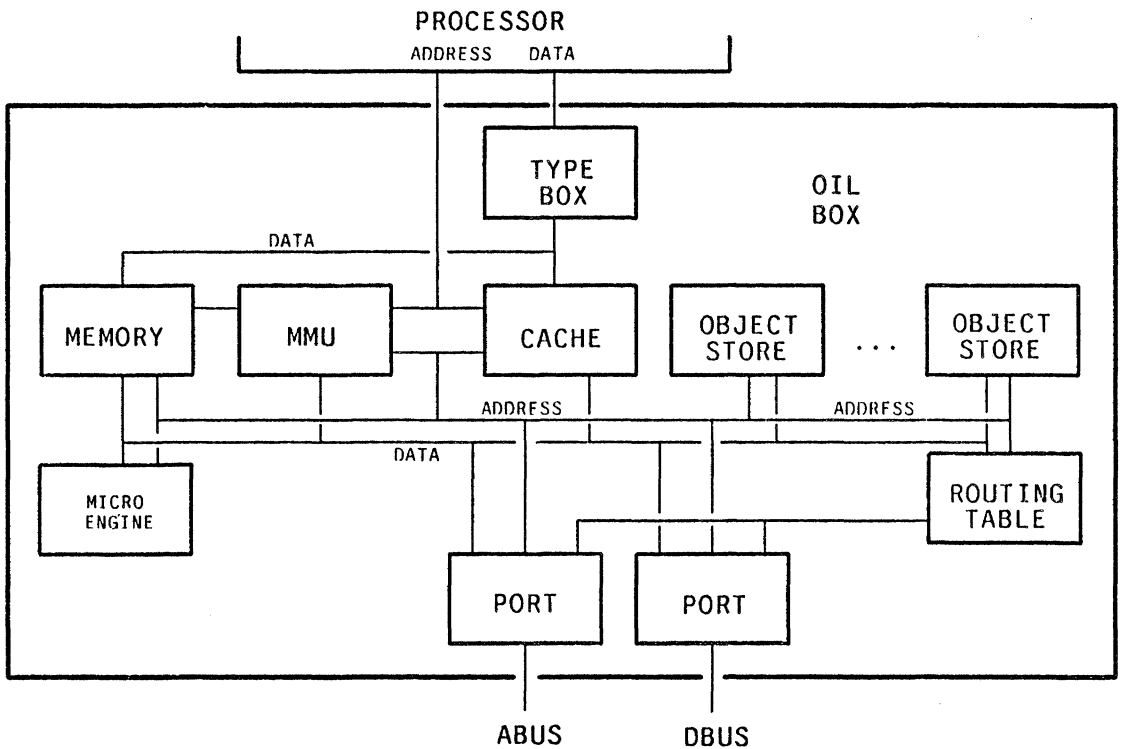
Figure 4-9: The object interface layer is inserted between processor and interchange to assist in operand management.
