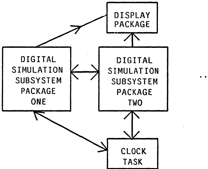
Figure 1-2: Mapping subsystems to separate simulation packages with inter process communication along well defined interface paths can improve simulator throughput.
