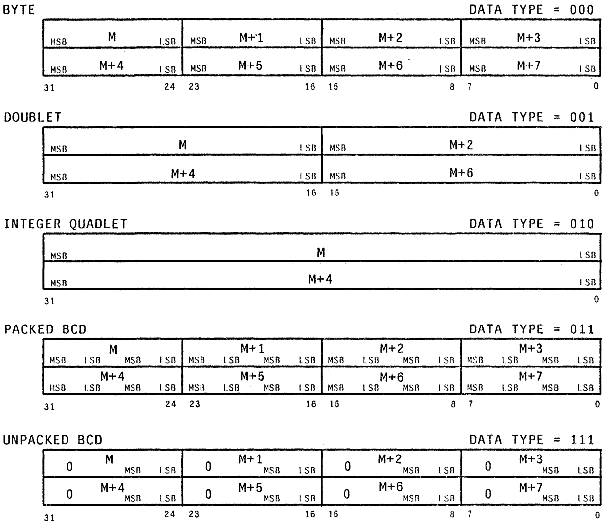
Figure 4-7: Five primitive scalar data types are supported based on Motorola 68000 representations.
