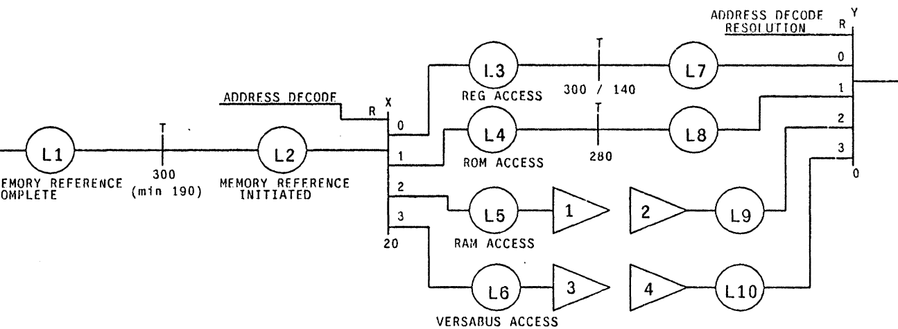
Figure 2-10: The processor's local bus allows access to local memory, board registers, and the Versabus port.
