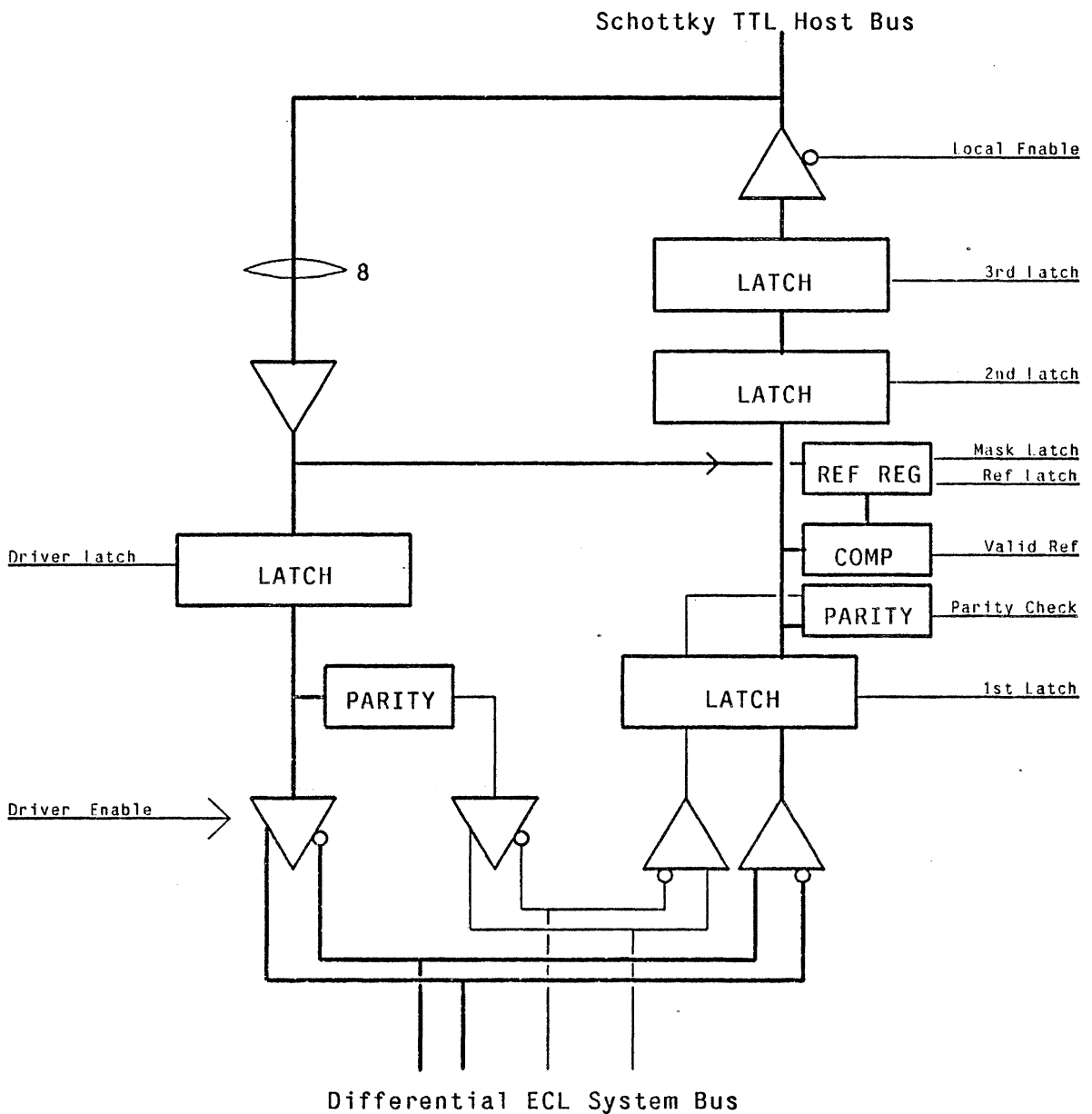
Figure 3-19: Consolidation of latches, drivers, parity logic, and comparators into a translator slice results in a fast, compact time-multiplexed bus.
