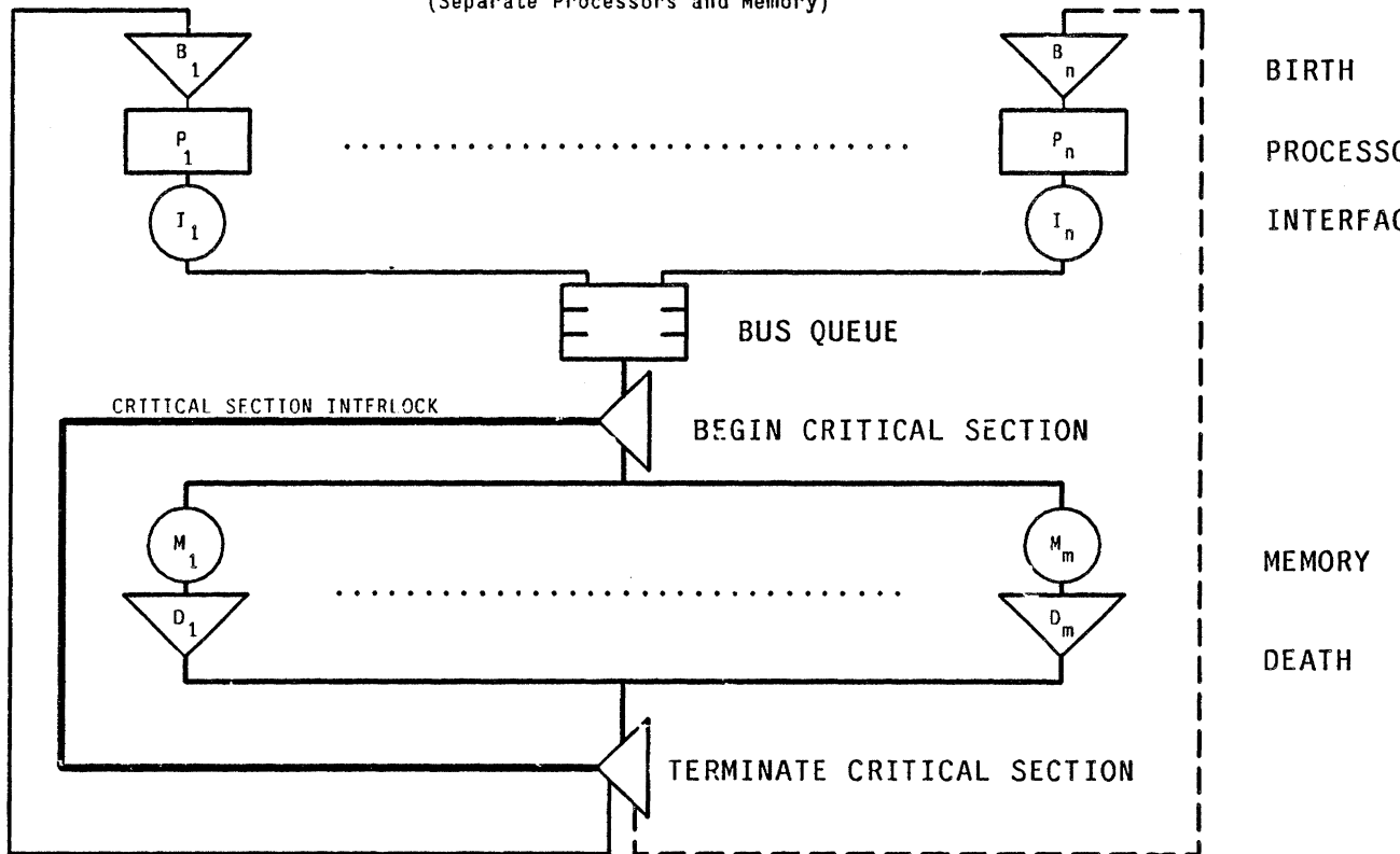
Figure 3-1: Use of separate processor and memory cards forces all processors to be served by a central memory server on all memory reference cycles.
