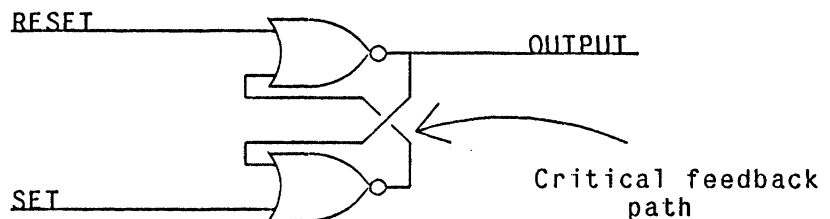
Figure 3-14: Bistable elements, designed conceptually like that above form the basis of the metastable problem.
