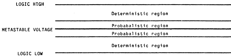
Figure 3-16: The metastable voltage is surrounded by a small probabilistic region, where escape is noise dependent, and a larger deterministic region where the propagation delay is design dependent.
