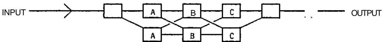
Figure 5-7: Dividing a system into many, spared modules can increase fault tolerance.
