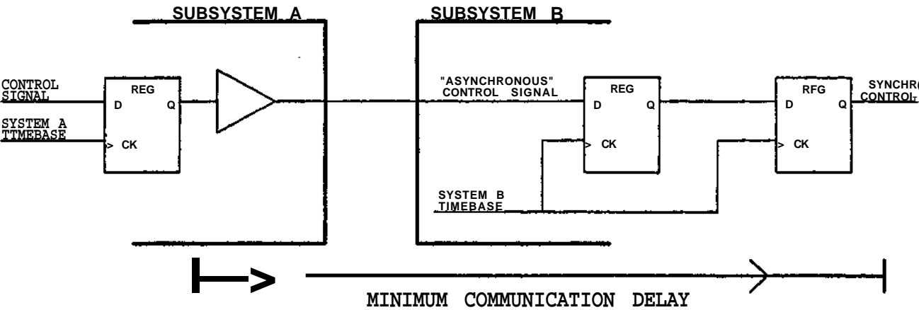
Figure 3-17: Design of a practical system using an asynchronous interface requires a synchronization latency to increase the mean time between metastables that propagate through to the second subsystem.
