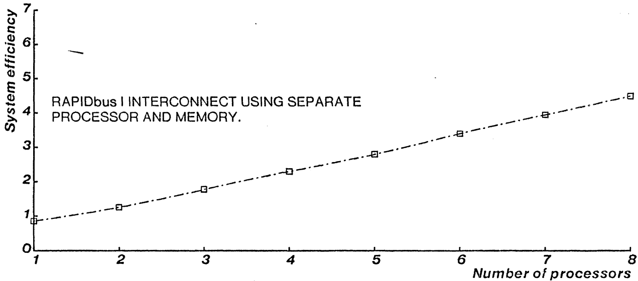
Figure 3-4: Separate processors and memory cards running with the RAPIDbus interface dramatically improve the throughput, but in an absolute sense, still runs poorly.
