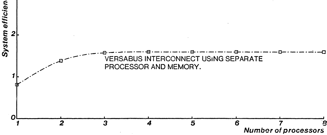
Figure 3-2: With separate Versabus processor and memory cards communicating on the bus, our system would level out at less than twice the performance of a single processor.
