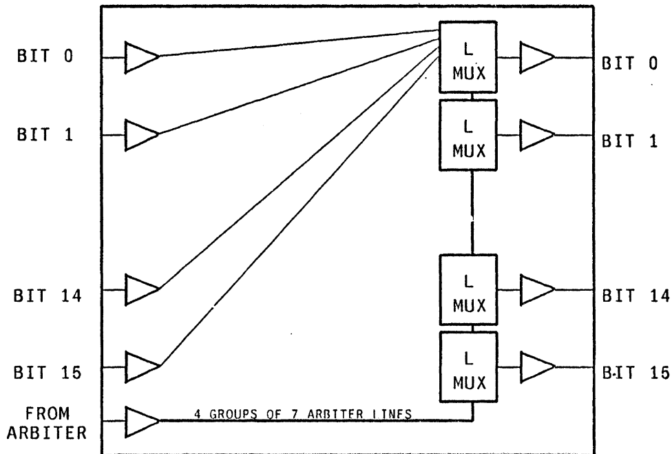
Figure 5-8: Bit slice crosspoint switch permits changing one routing per cycle in each of four groups.
