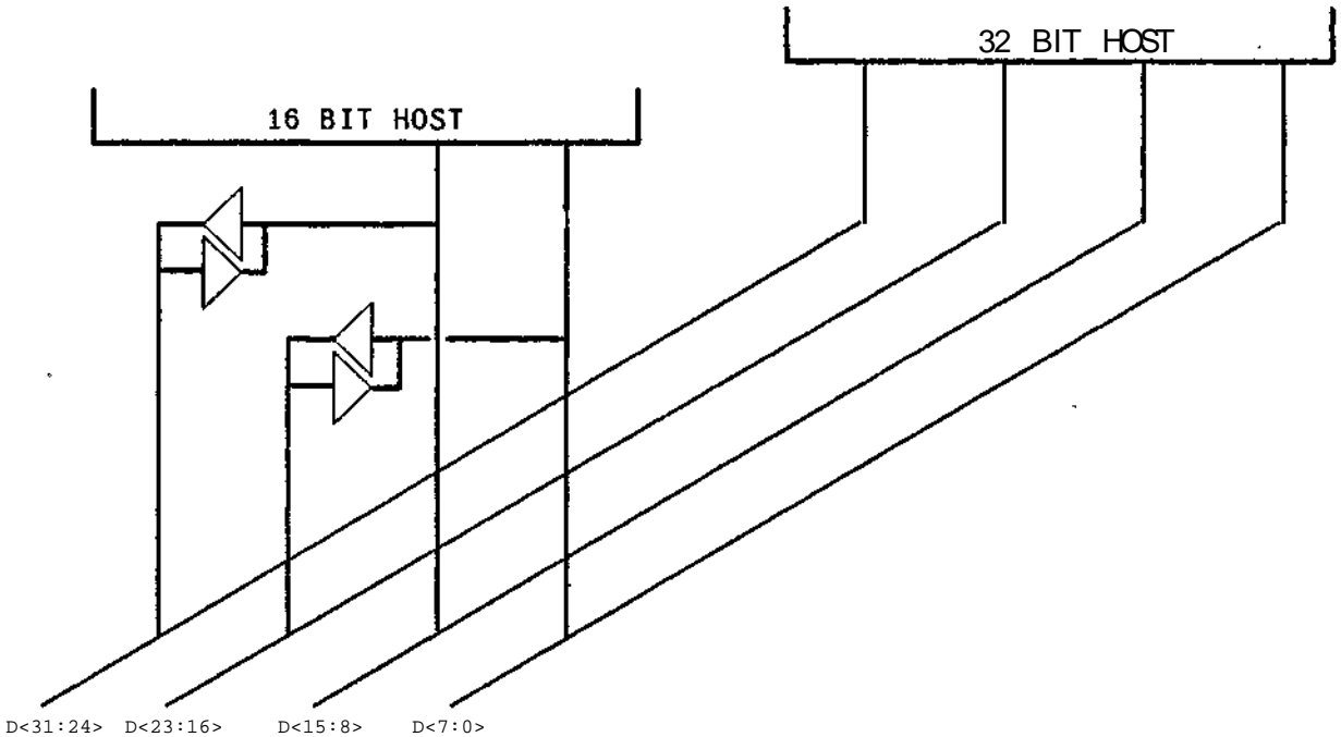
Figure 5-5: Use of a sixteen bit host on a thirty-two bit unjustified bus requires a crossover to allow access to all bytes in memory along low data lines.
