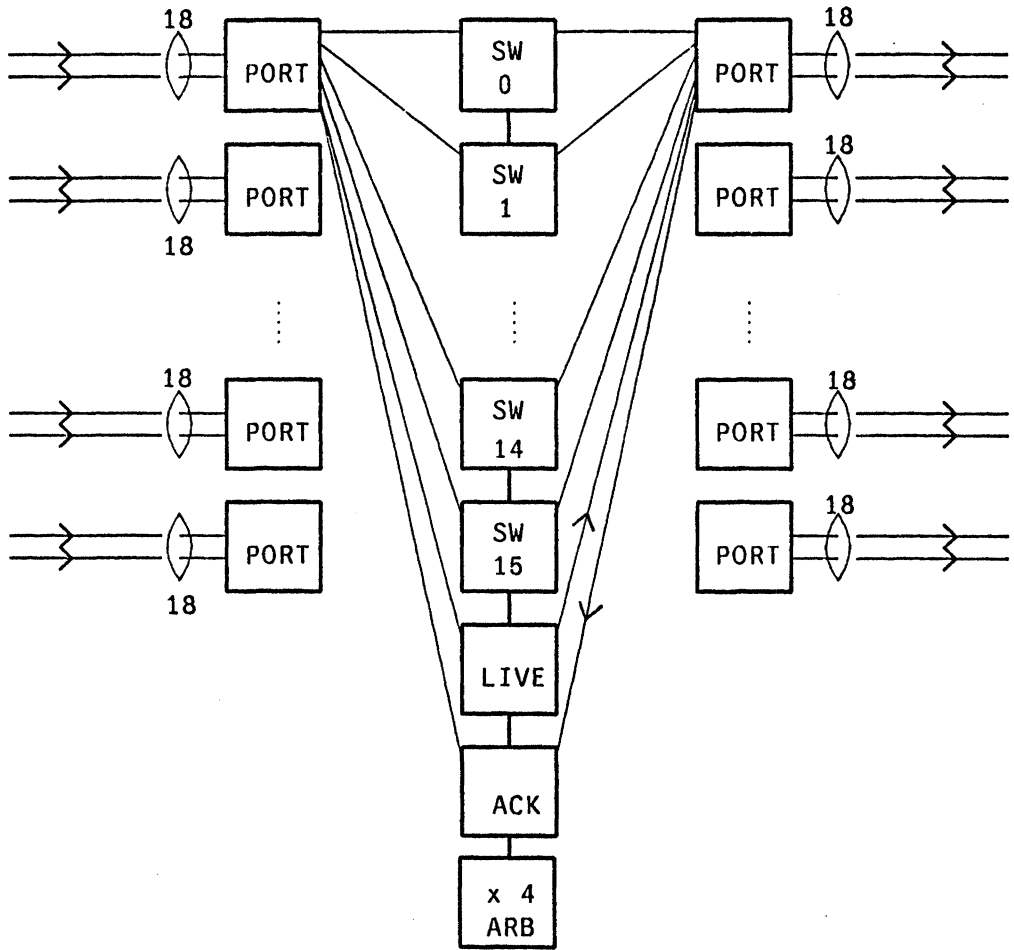
Figure 5-10: Eighteen bit slice crosspoint chips interconnect a society of RAPIDbus II processor nodes.
