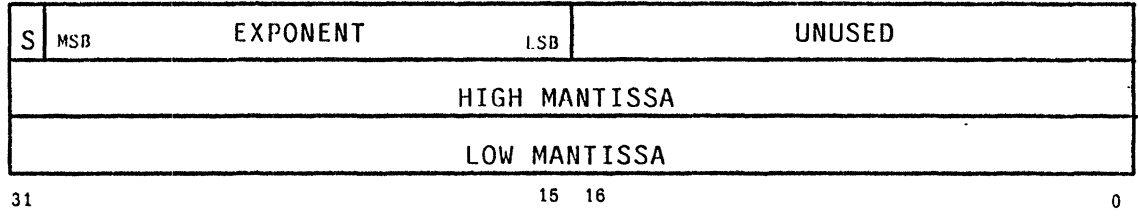
Figure 4-8: Three different floating point representations are supported based on the Motorola packing of the proposed IEEE floating point specification P754.
