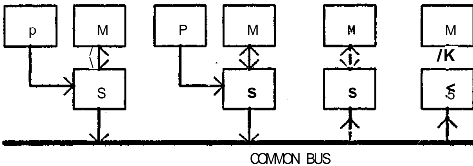
Figure 2-4: Addition of local memory on the processor card permits quick access to private data and instructions.
