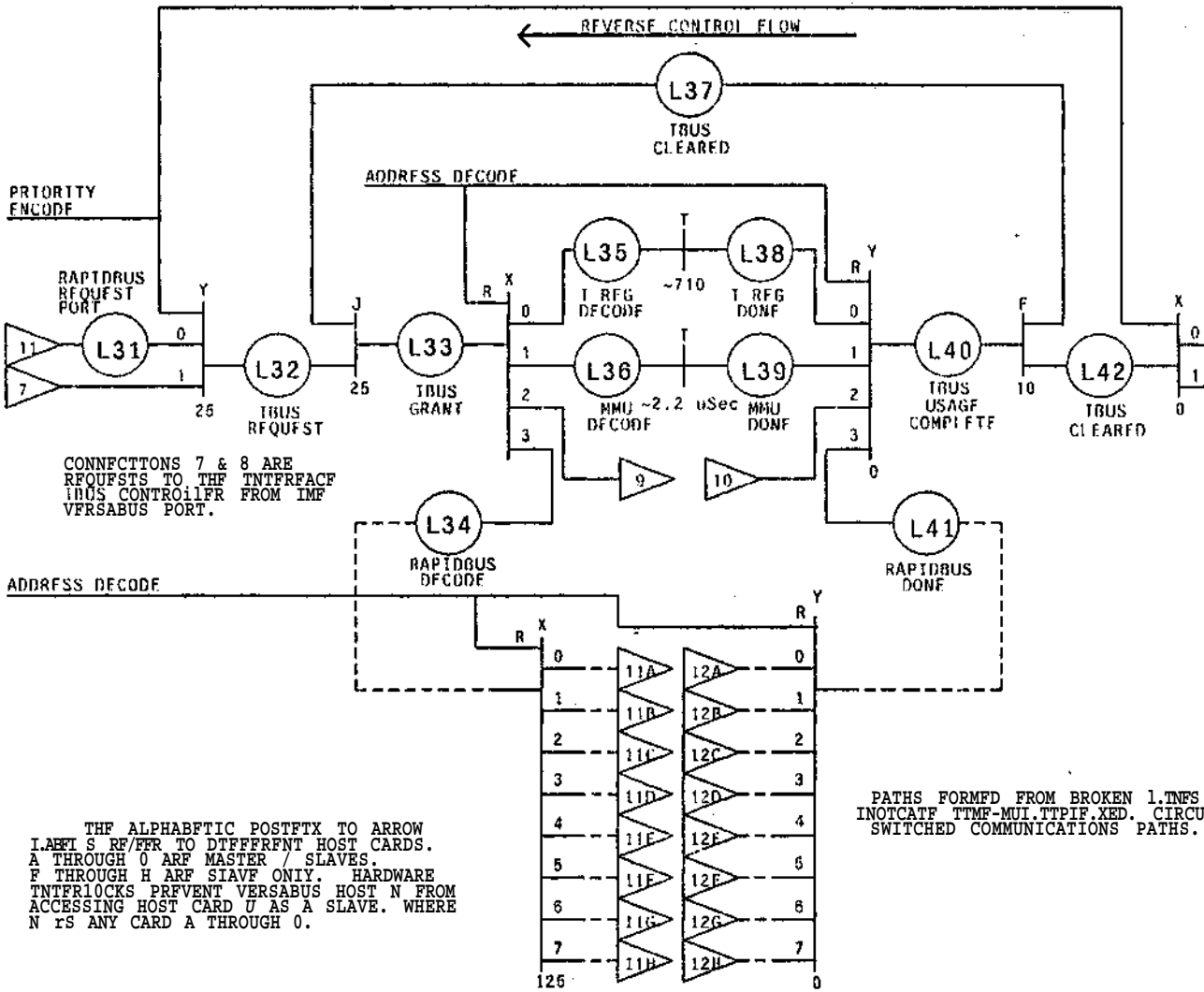
Figure 2-15: The RAPIDbus interconnect provides four virtual bus paths, each of which is described by the graph above.
