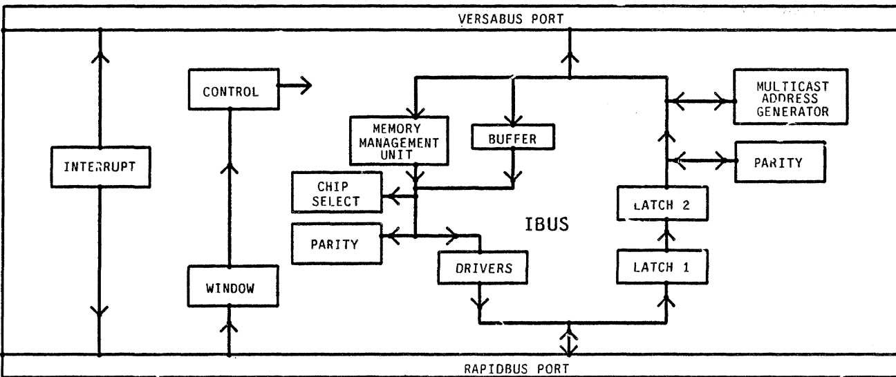
Figure 2-7: Each RAPIDbus interface card is composed of multiple modules, centered around the Ibus.
