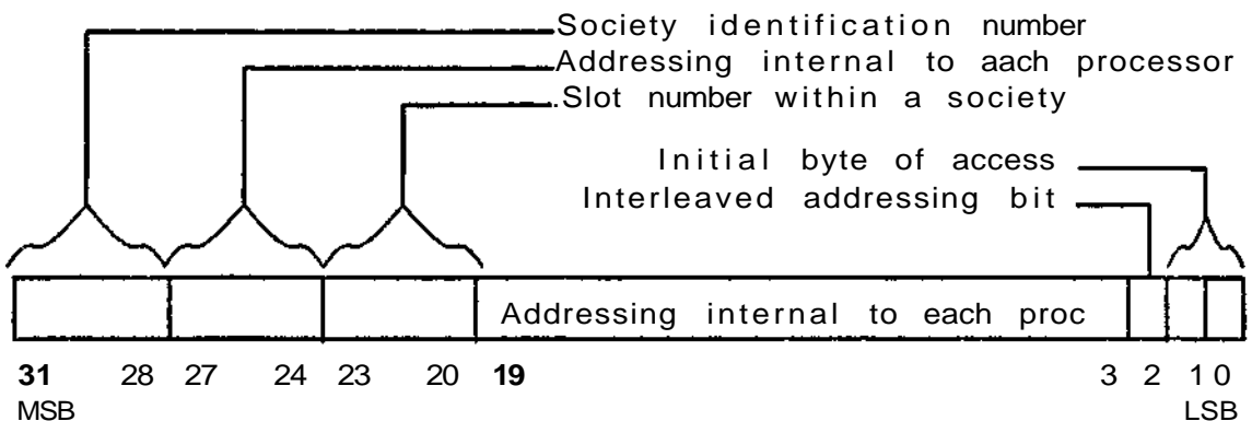
Figure 4-6: The physical address space is partitioned hierarchically into societies and then host nodes within a society.
