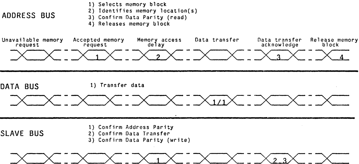
Figure 3-13: Analysis of the information content during each window of a RAPIDbus I data transfer operation suggests more efficient transmission protocols.
