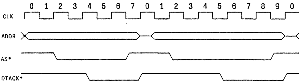
Figure 2-8: Bus transfer timing relative to the processor clock for two cycles, the first in zero wait states, the second requiring an extra clock cycle.
