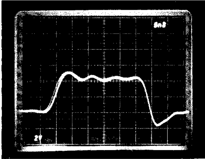
Figure 3-20: Use of a good ground plane, bypassing, and short lines, acceptable waveforms were achieved using wire wrap on RAPIDbus I.
