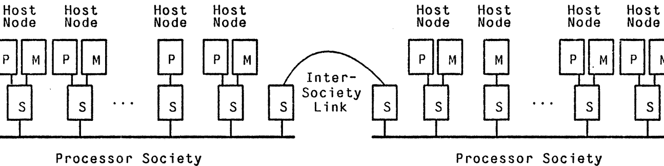
Figure 4-2: The RAPIDbus II architecture is composed of societies with up to fifteen host nodes. High speed parallel links between societies can be configured in response to research requirements.
