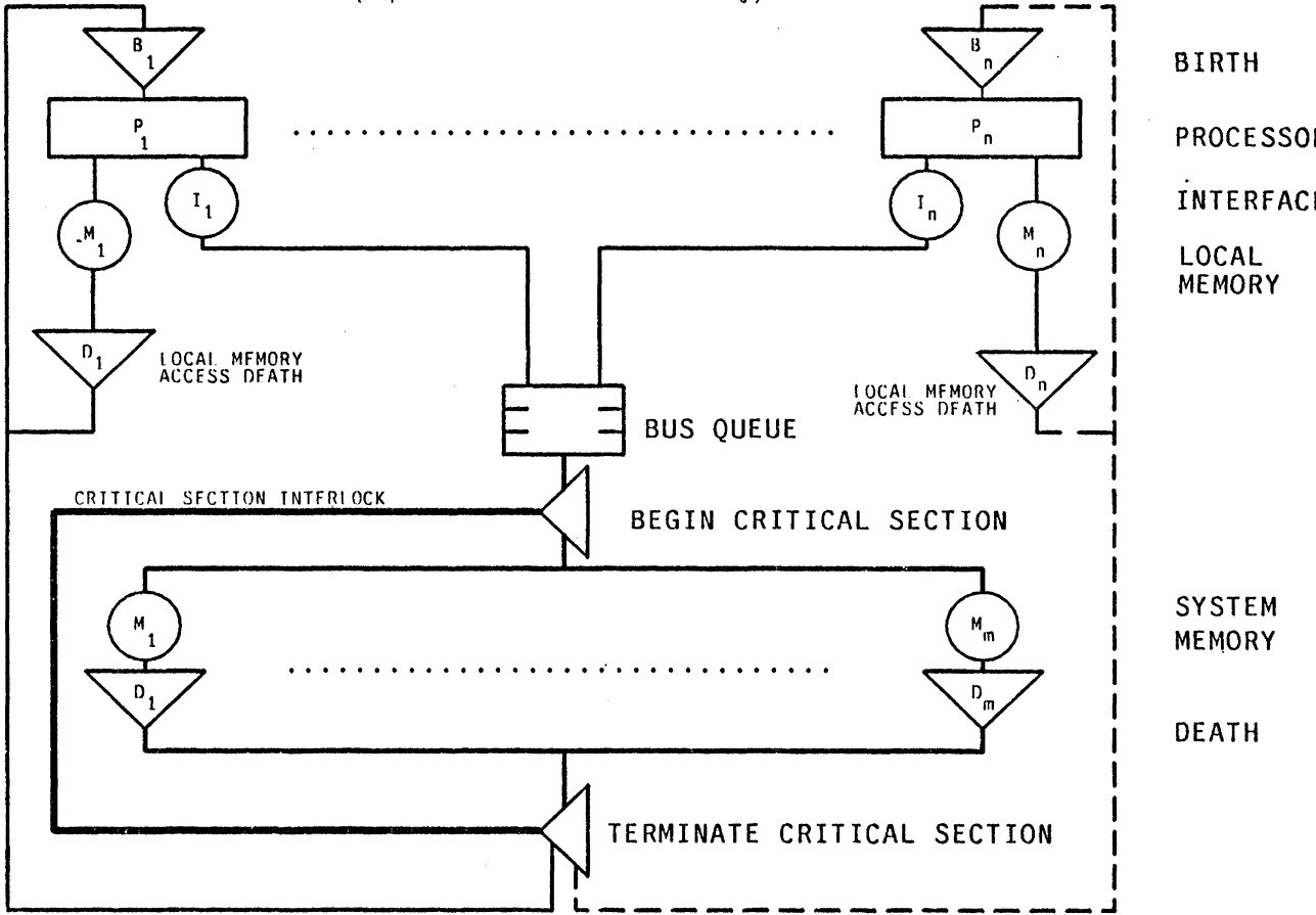
Figure 3-5: Addition of local memory on each processor decreases contention for main memory while increasing the complexity of memory allocation.
