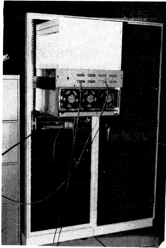
Figure 2-1: A dual height Versabus card cage was constructed to house the two processor RAPIDbus I prototype.
