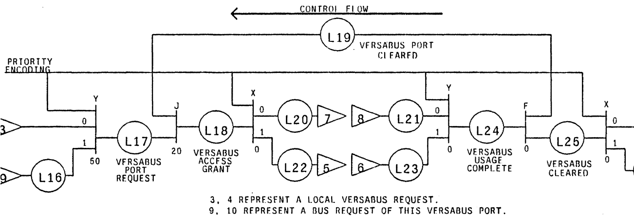
Figure 2-12: The dual port arbiter allows a connection between local bus and Versabus or between local ran and the Versabus.
