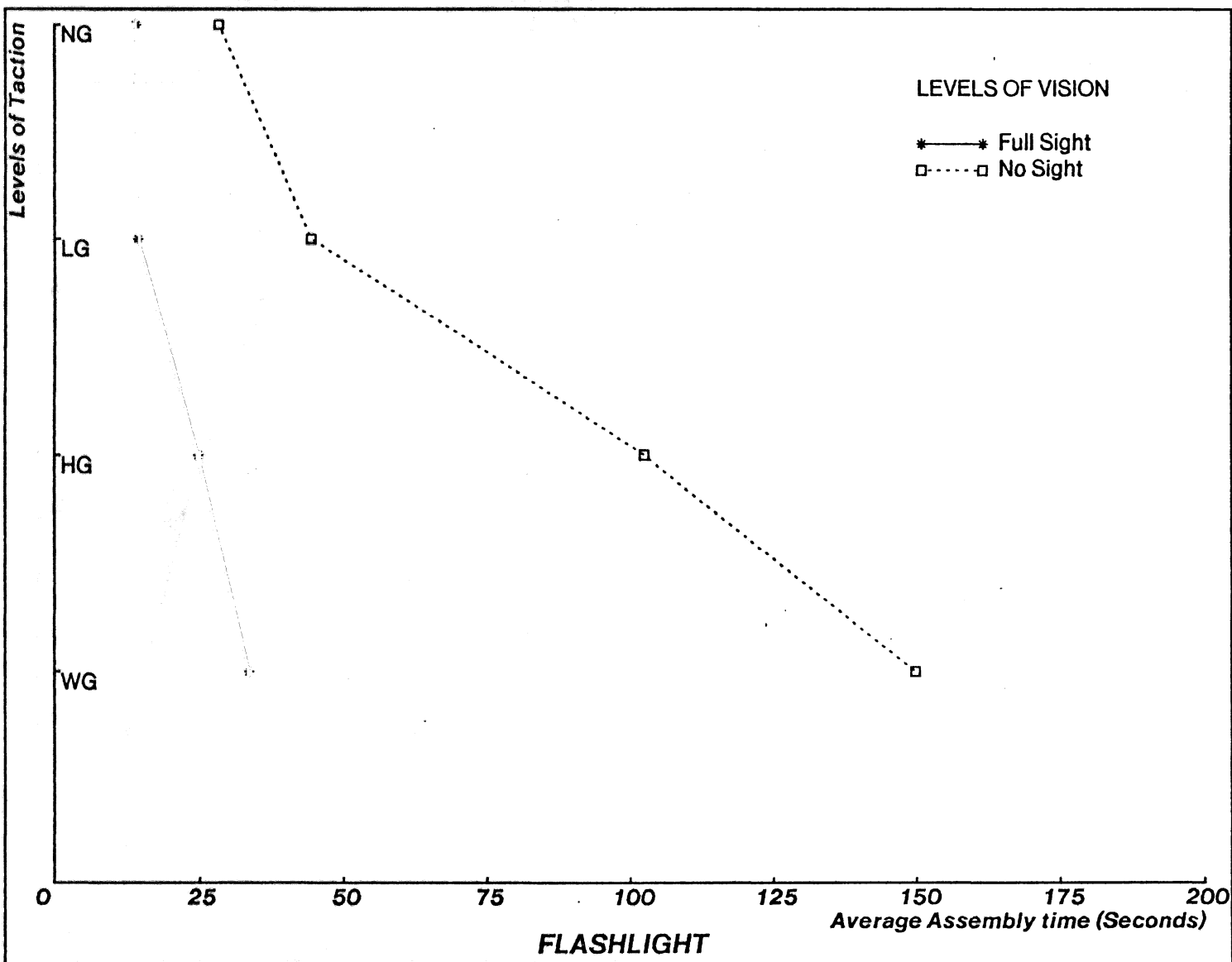
Figure 1-12: Flashlight: Average Assembly Time Vs Vision (Full Sight/No Sight) and Taction
