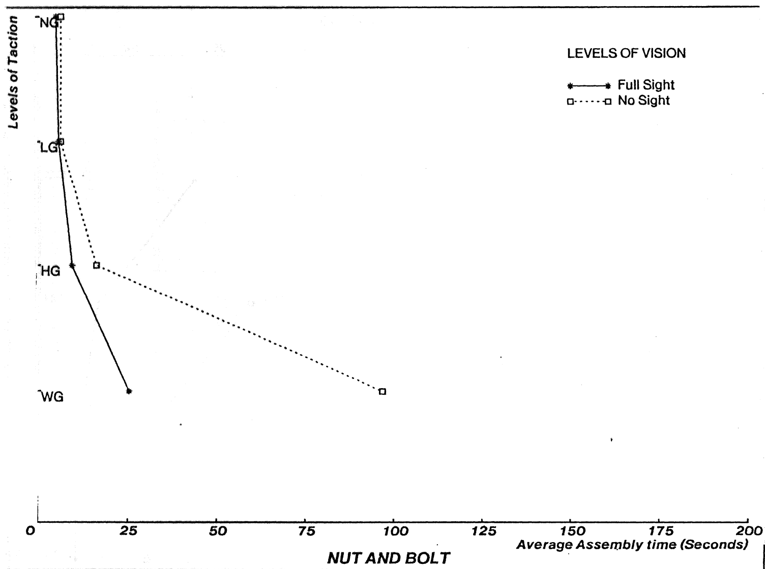
Figure 1-11: Nut and Bolt: Average Assembly Time Vs Vision (Full Sight/No Sight) and Taction
