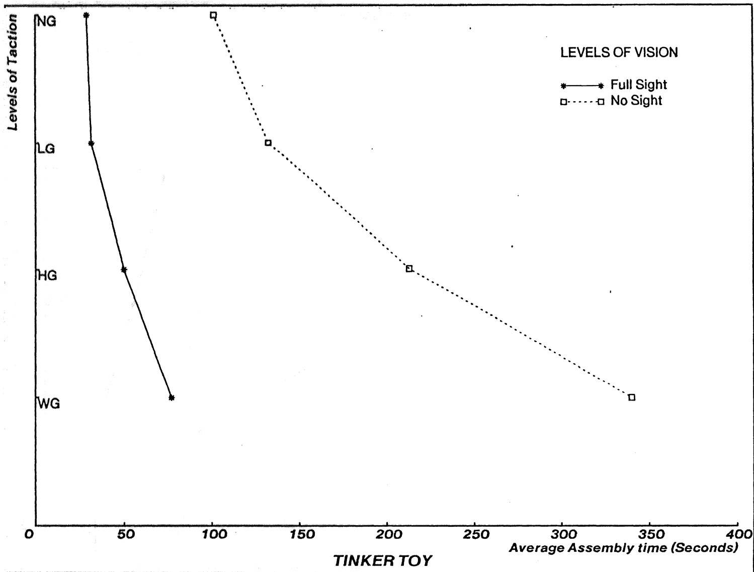
Figure 1-13: Tinker Toy: Average Assembly Time Vs Vision (Full Sight/No Sight) and Taction
