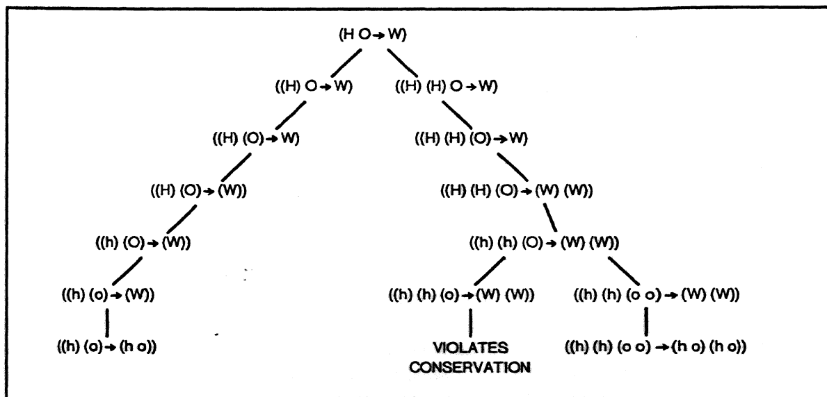
Figure 3. DALTON's search for a model of the water reaction.
