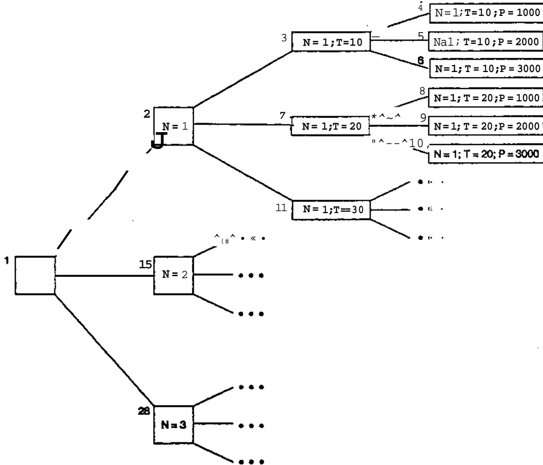
Figure L BACON'S search through the space of data.
