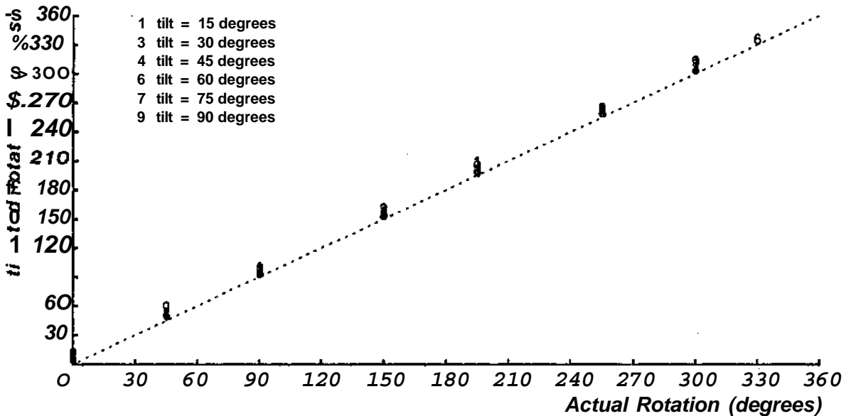
Figure 5.12s Actual vs. estimated rotation from combined system. Data is labelled by tilt for 49 images under normal illumination.
