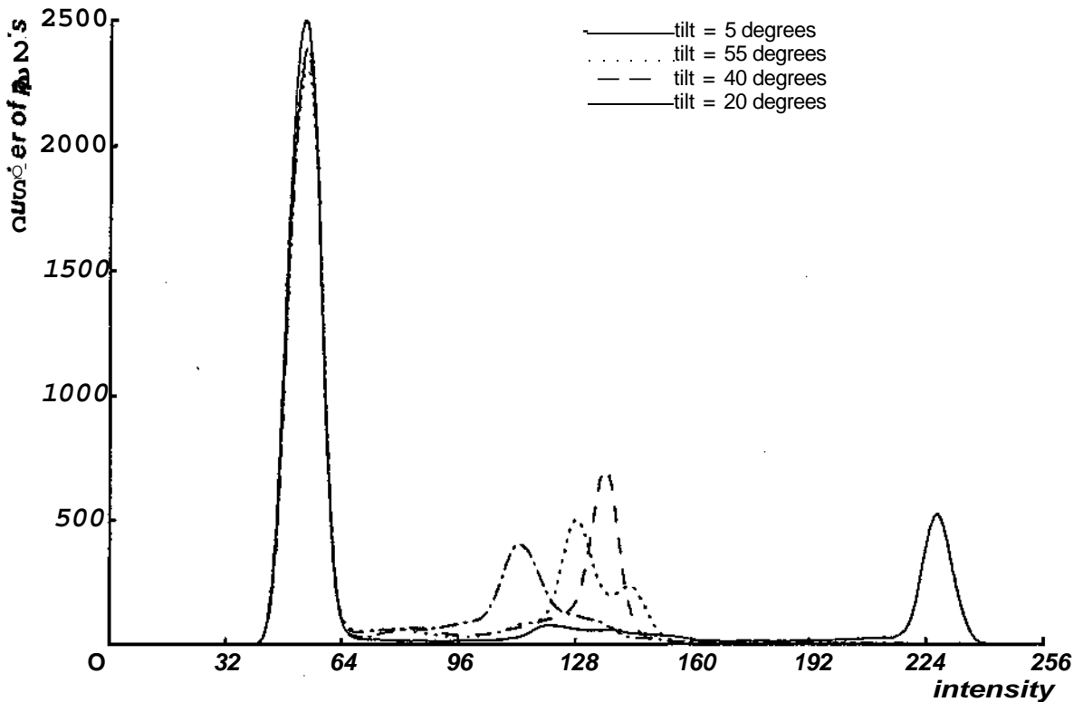
Figure 2.2: Actual histogram data for a single transistor, against a dark background, at four different orientations. There are 256 different grey-levels and a total of 36,864 pixels.
