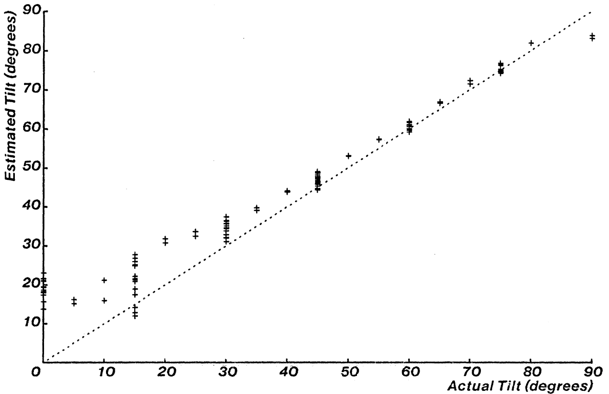
Figure 4.17: Actual transistor tilt vs. tilt estimated from ellipse parameters. Ellipse fit was obtained using intensity gradient information, as well as selected transistor boundary points.
