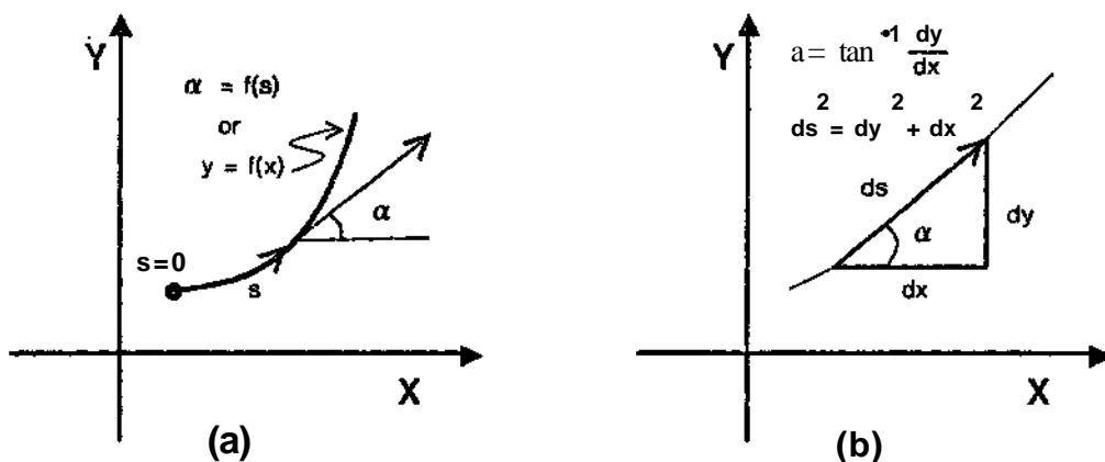
Figure 4.7: (a) The definition of a curve as either y = f(x) or a = f(s) . (b) The relationship between dy/dx and a , ds .
