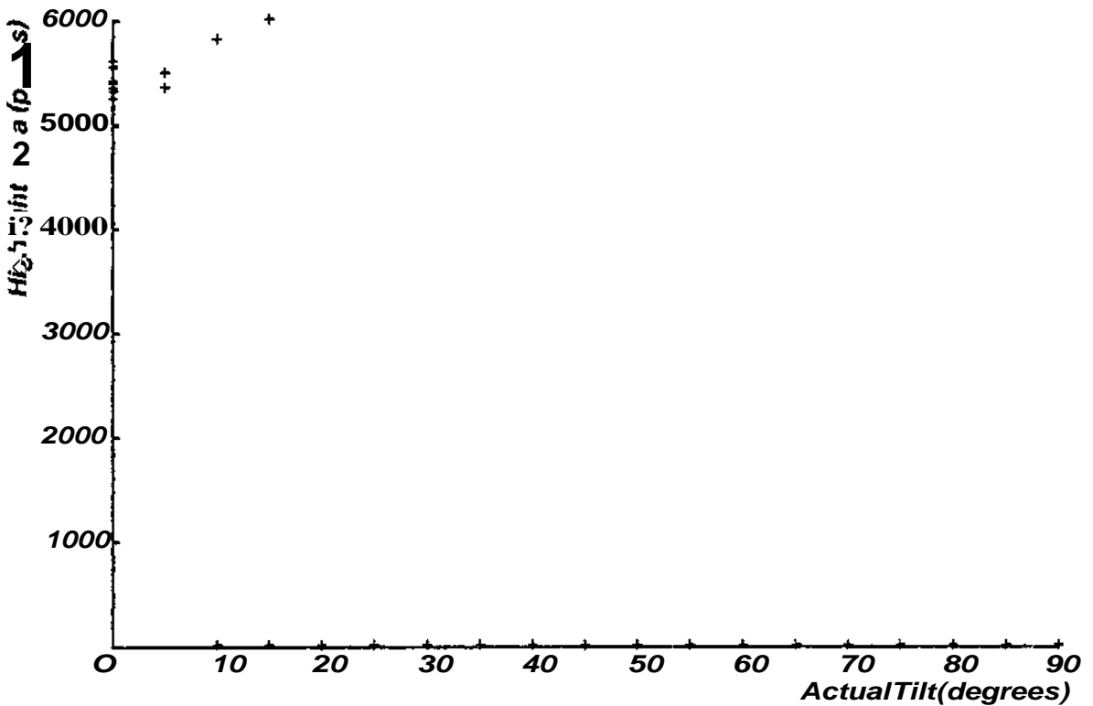
Figure 2.6: Transistor tilt vs. area of the highlight region. If no histogram highlight region is found, the area is assumed to be zero.
