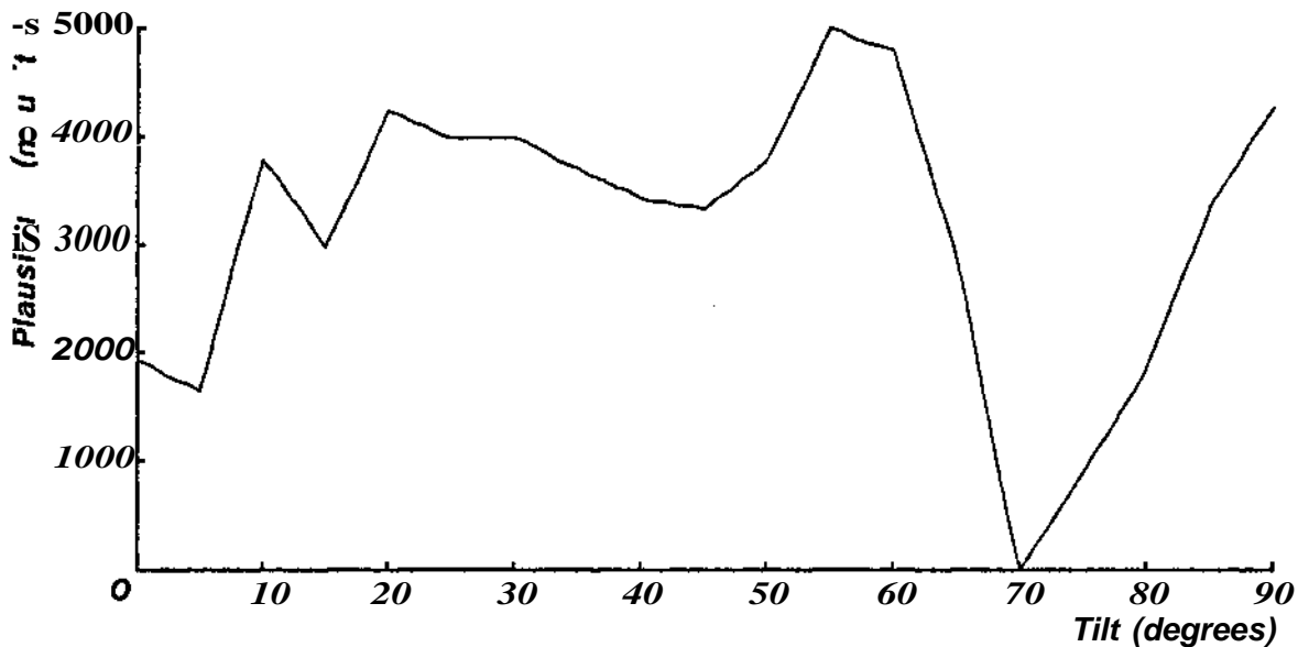
Figure 5.4: Tilt plausibility function obtained from histogram template matching. Maximum plausibility occurs at tilt of 55°. The actual transistor tilt is 60°.
