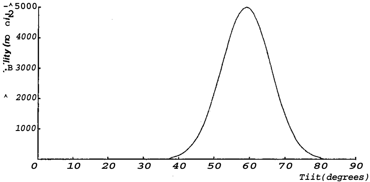
Figure 5.3: Tilt plausibility function obtained using ellipse fitting. Maximum plausibility occurs at tilt of 59.3°. The actual transistor tilt is 60°.
