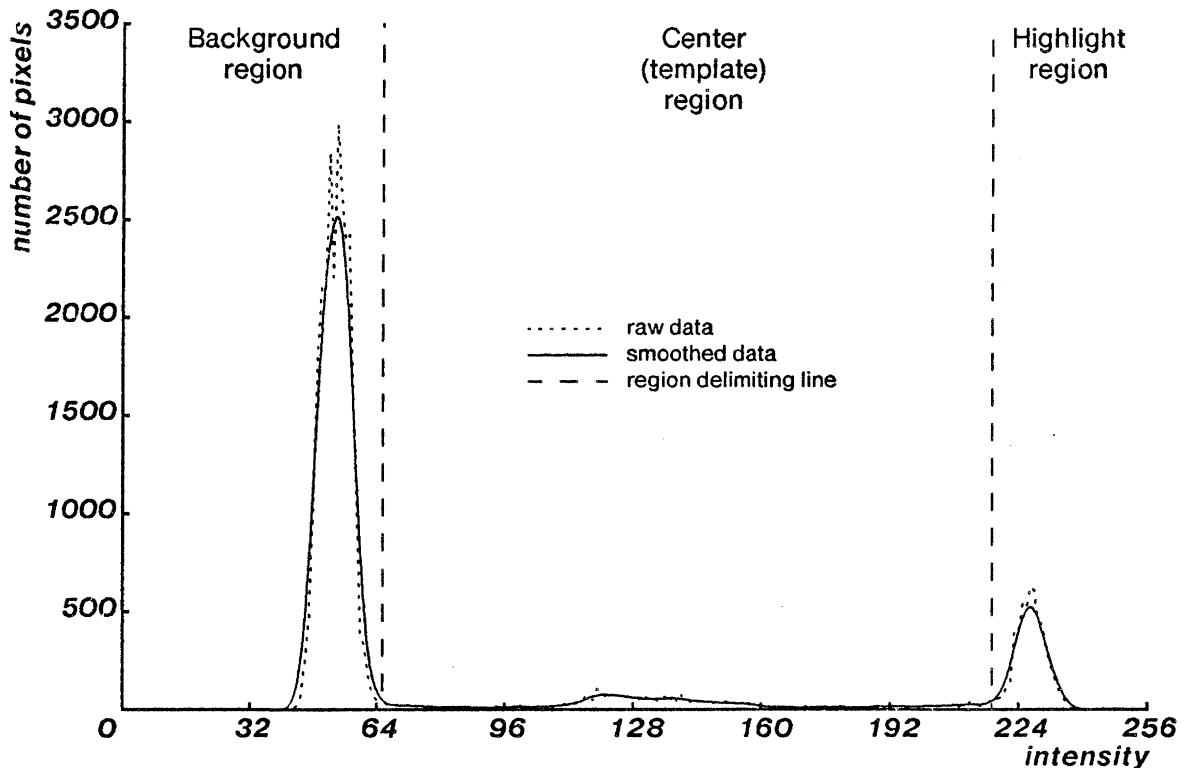
Figure 2.3: Transistor histogram for tilt = 5°. Both the raw and smoothed data are shown along with the 3 different regions of the histogram.
