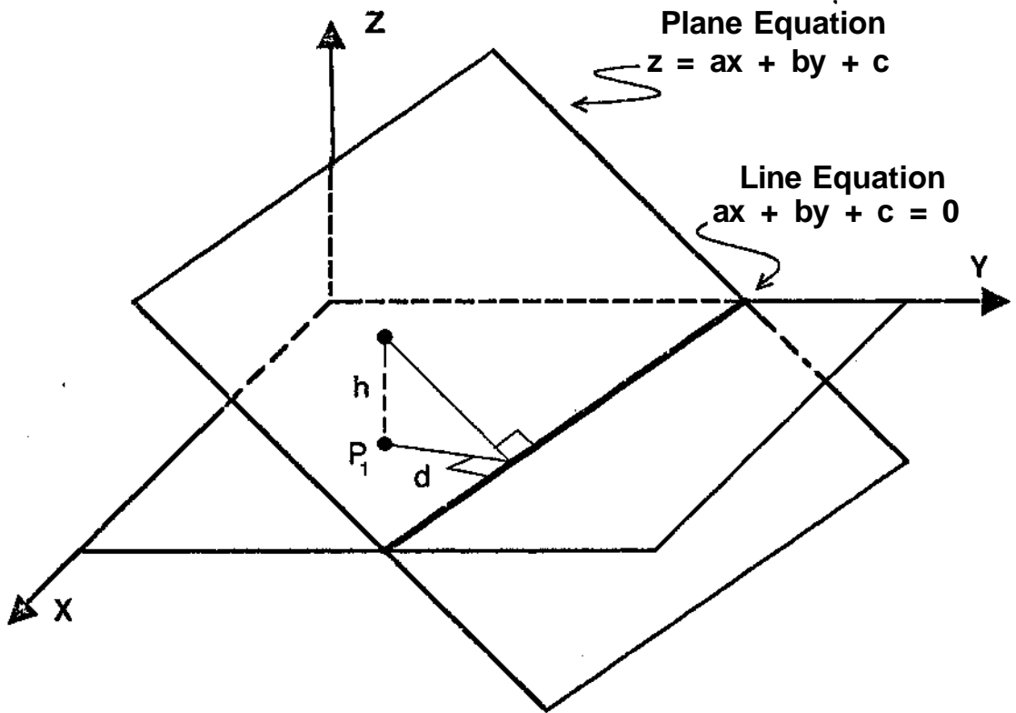
Figure 4.2: The line ax+by+c = 0 is represented by the intersection of the plane z = ax + by + c with the xy plane. The distance d from the line to point P = (z_i, y_i) in the xy plane is equal the height h of the plane at (z_i, y_i) divided by the magnitude of the plane gradient, \| \nabla G \| .
