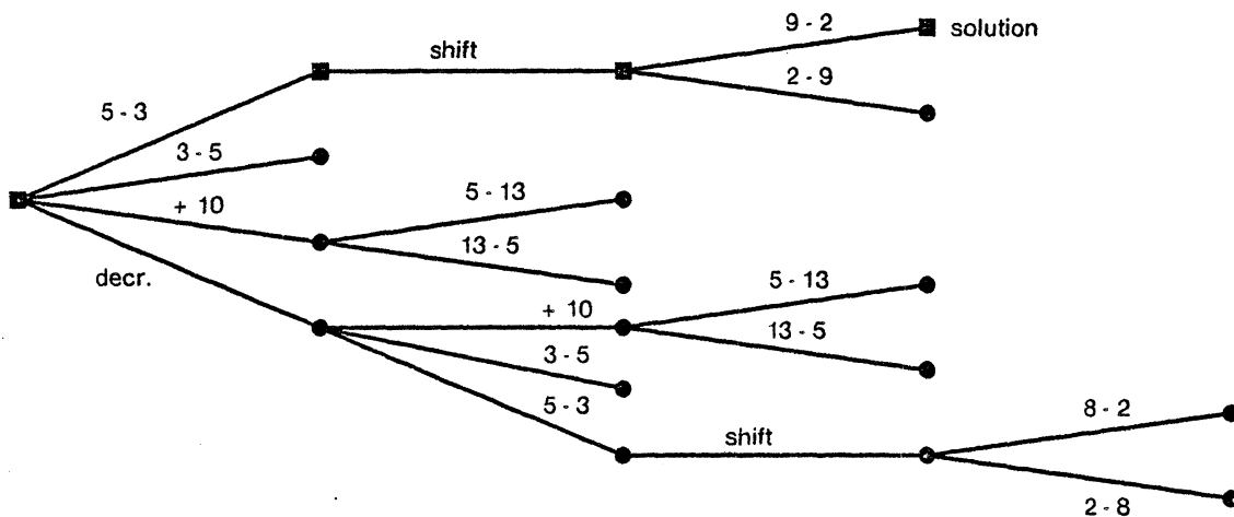
Figure 5. Search tree for the problem 93 - 25 = 72 .
