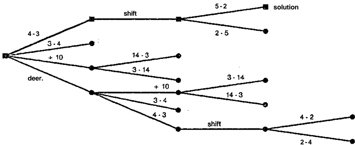
Figure 2. Search tree for the problem 54 - 23 = 31 .
