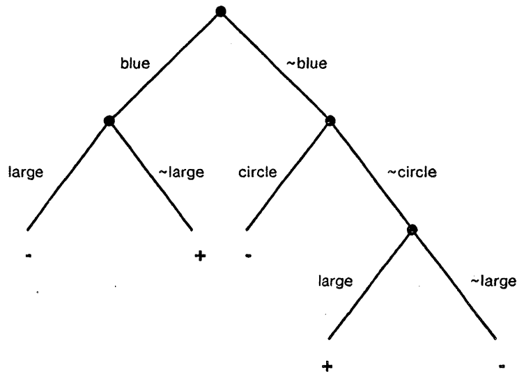
Figure 1. A sample discrimination network.
