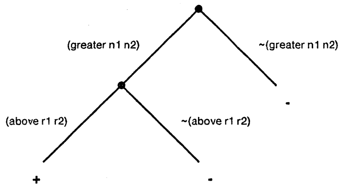
Figure 4. Correct discrimination network for the find-difference operator.
