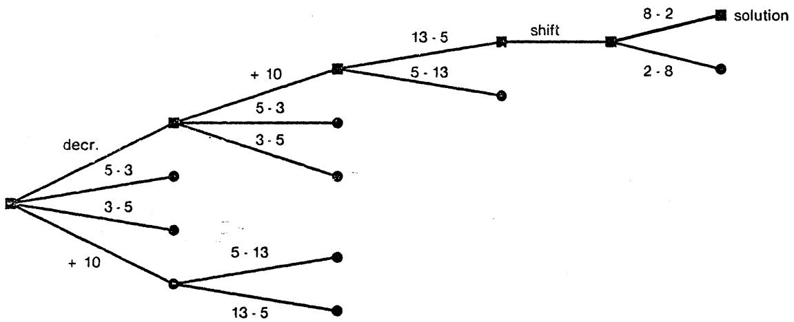
Figure 3. Search tree for the problem 93 - 25 = 68 .
