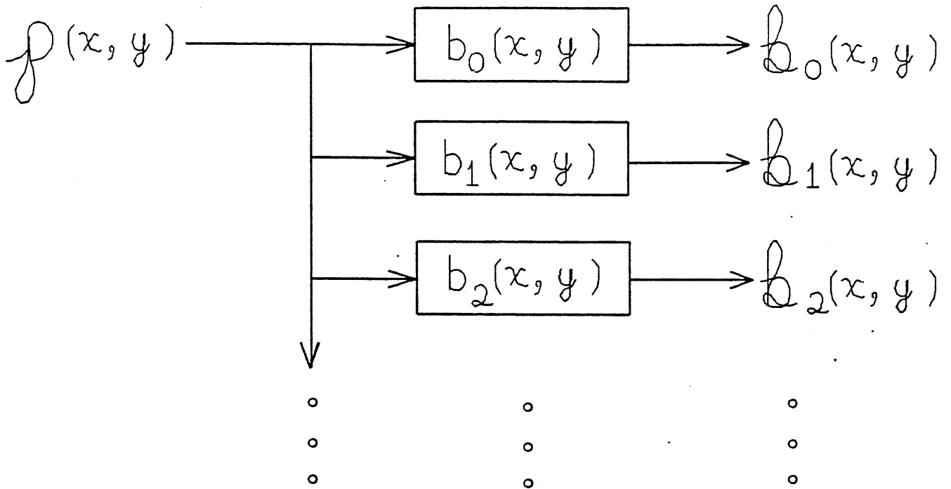
Figure 1: The Difference of Low-Pass (DOLP) Transform
