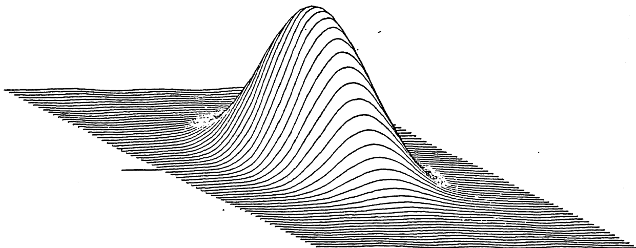
Figure 9: Transfer Function G_o(u,v) for R = 4.0 , \alpha = 4.0 Before \sqrt{2} Expansion
