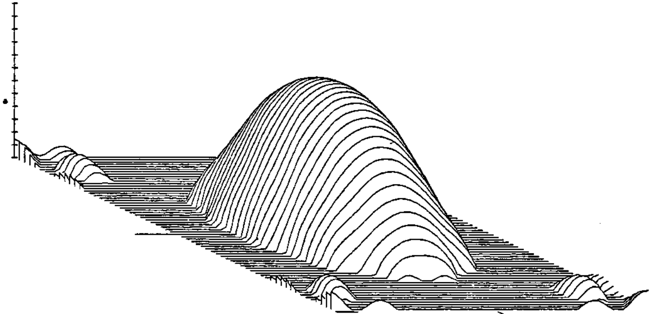
Figure 12: Plot of 20 \text{ Log}_{10}[G_2(u,v)] Scale (shown at left) spans -120 dB.
