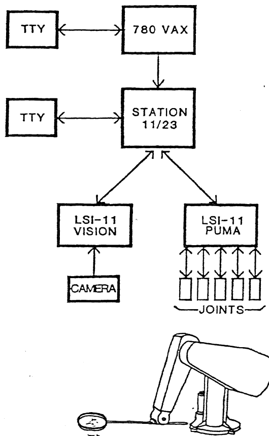
Figure 3-1: Hardware Components
