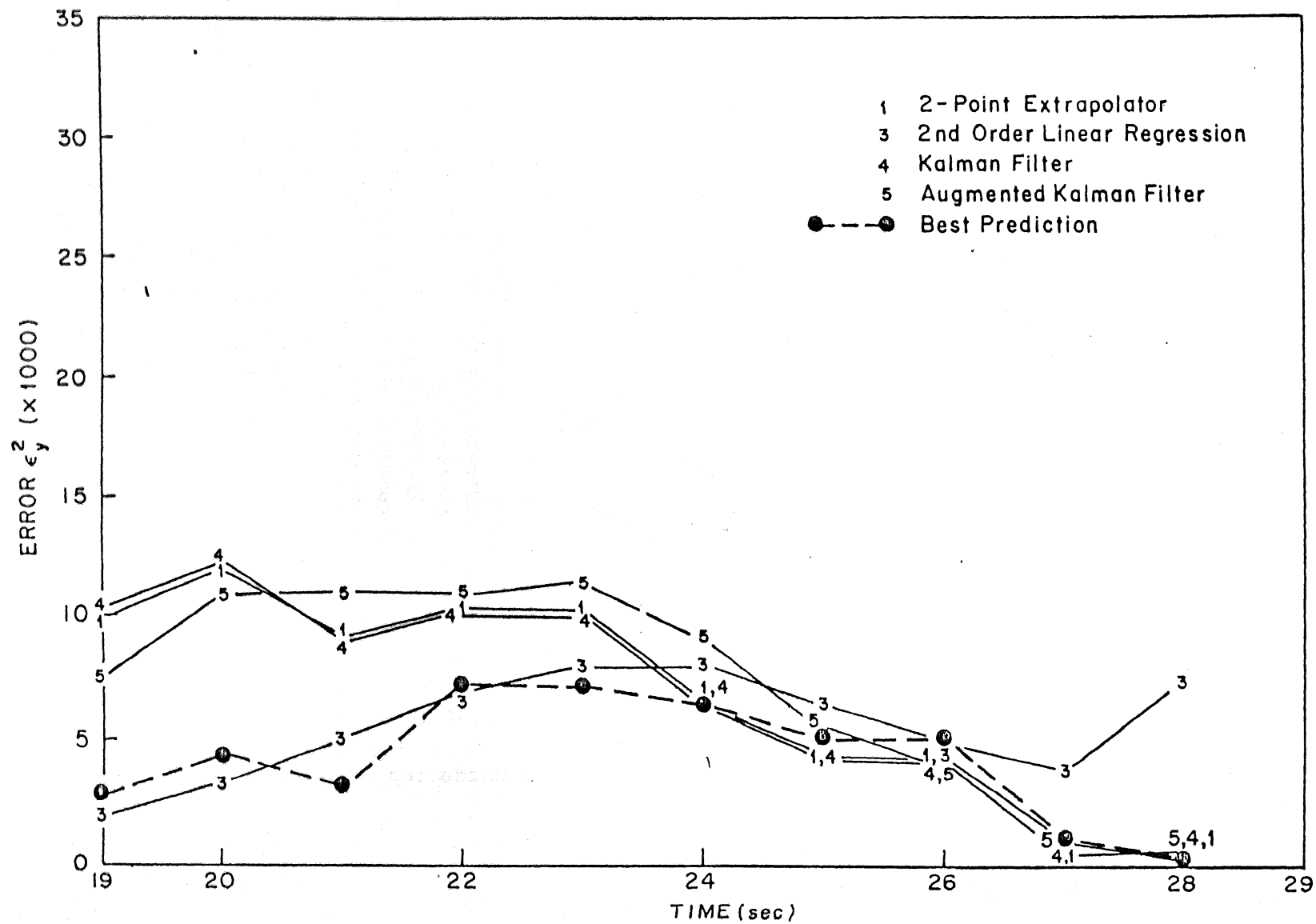
Figure 1-7: Smoothed \epsilon_y^2 vs T - Relative 3-Step Prediction, Target
