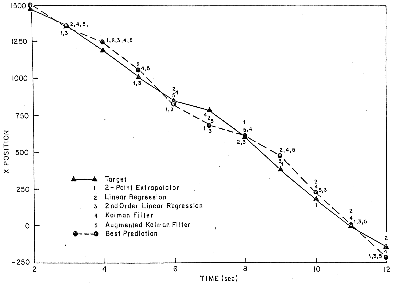
Figure 4-3: X vs T Relative 1-Step Predictions, Target Moving
