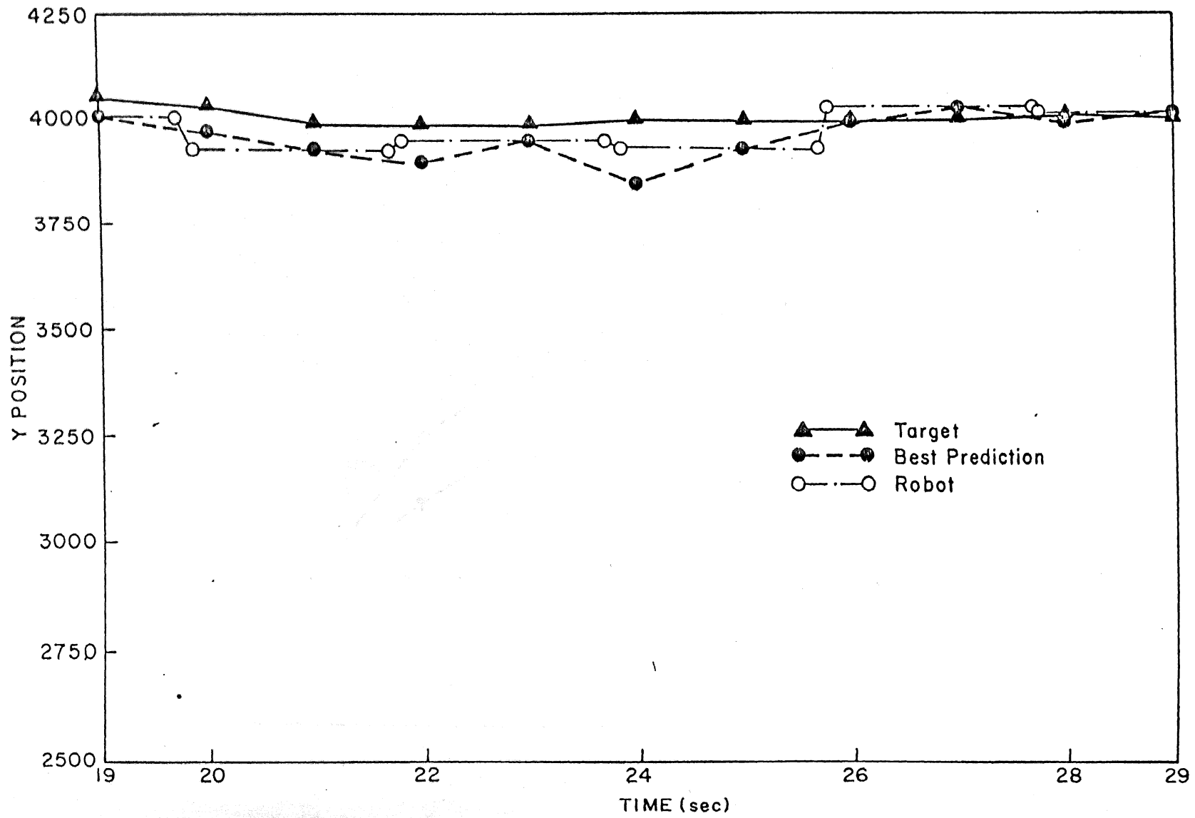
Figure 4-10: Y vs T Robot Trajectory - Relative 3-Step Prediction, Target
