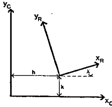
Figure 3-3: Illustration of Camera to Robot Coordinate Transformation
