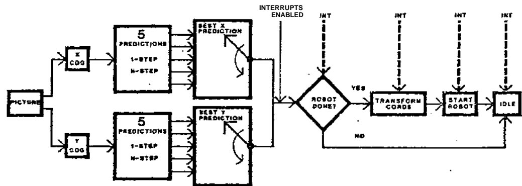
Figure 3-2: Robotic Tracking Control System
