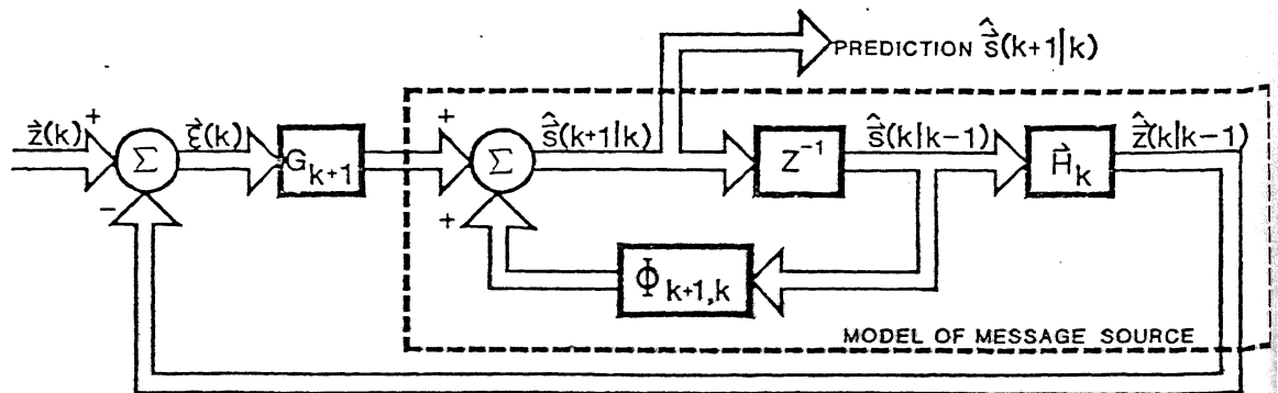
Figure 2-2: Optimum filter based on the one-step prediction algorithm
