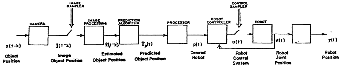
Figure 1-1: Target Tracking Control System
