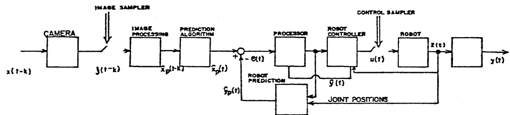
Figure 5-1: Closed-Loop Tracking System
