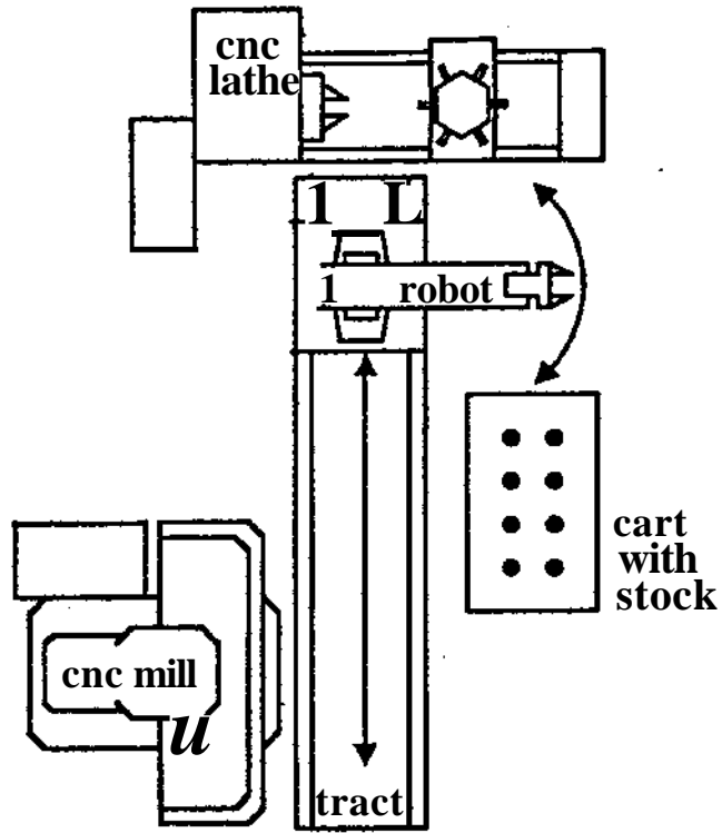
Figure 3-3: First Variation on Machining Cell Layout - Second Arrangement
