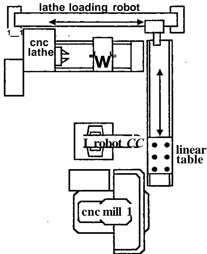
Figure 3-2: Machining Cell Layout - First Arrangement
