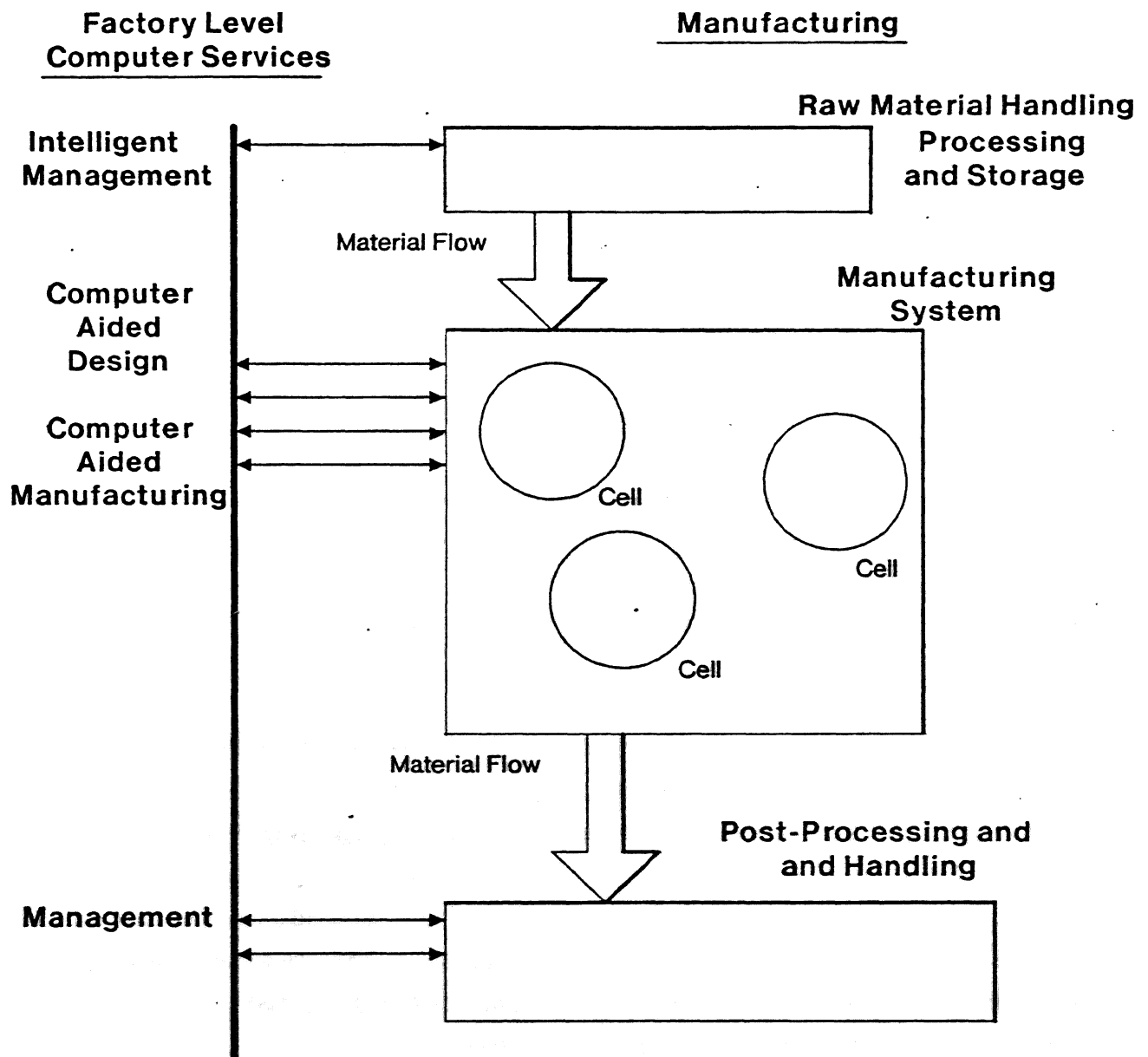
Figure 4-1: A Schematic of the Manufacturing System and the Factory Support Environment
