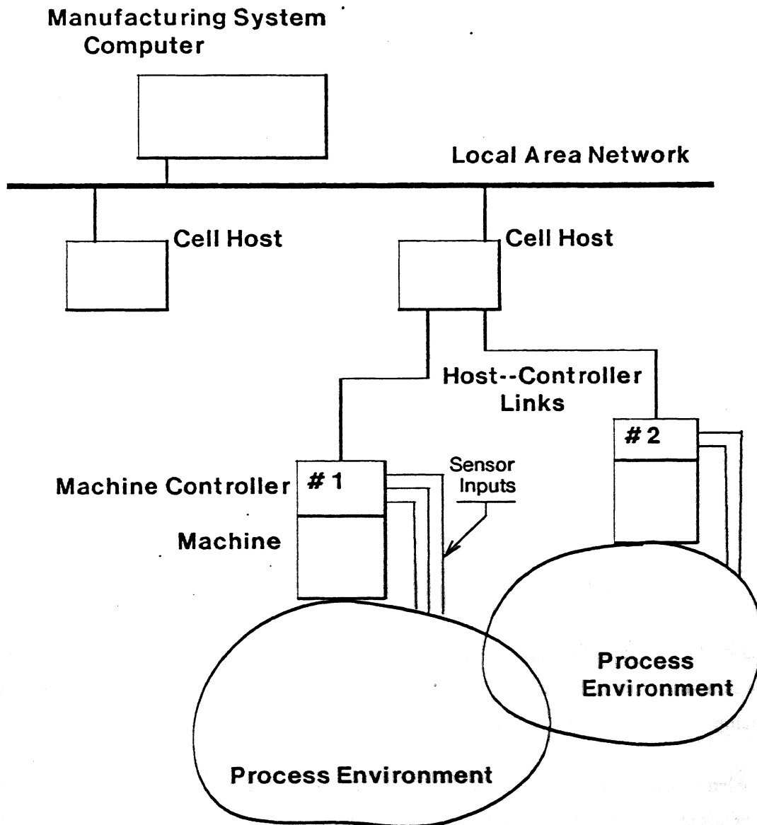
Figure 2-1: Hierarchical System Design
