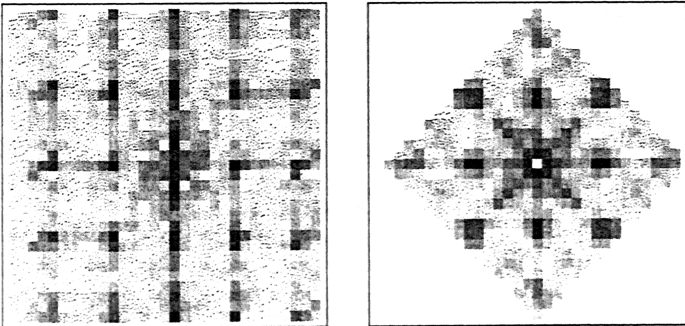
Figure 4-3: Power spectrum of Figure 4-2, and folded transform
