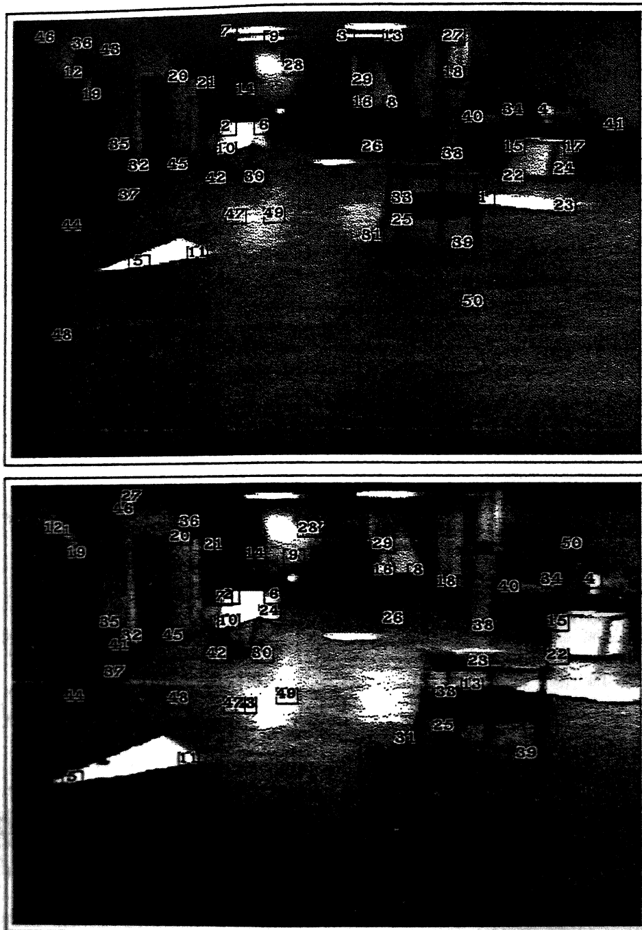
Figure 6-3: Example of the correlator's performance on a difficult example. The interest operator has chosen features in the upper image, and the correlator has attempted to find corresponding regions in the lower one. The cart moved about one and a half meters forward between the images. Some mistakes are evident. The correlator had no a-priori knowledge about the relationship of the two images and the entire second image was searched for each feature.
