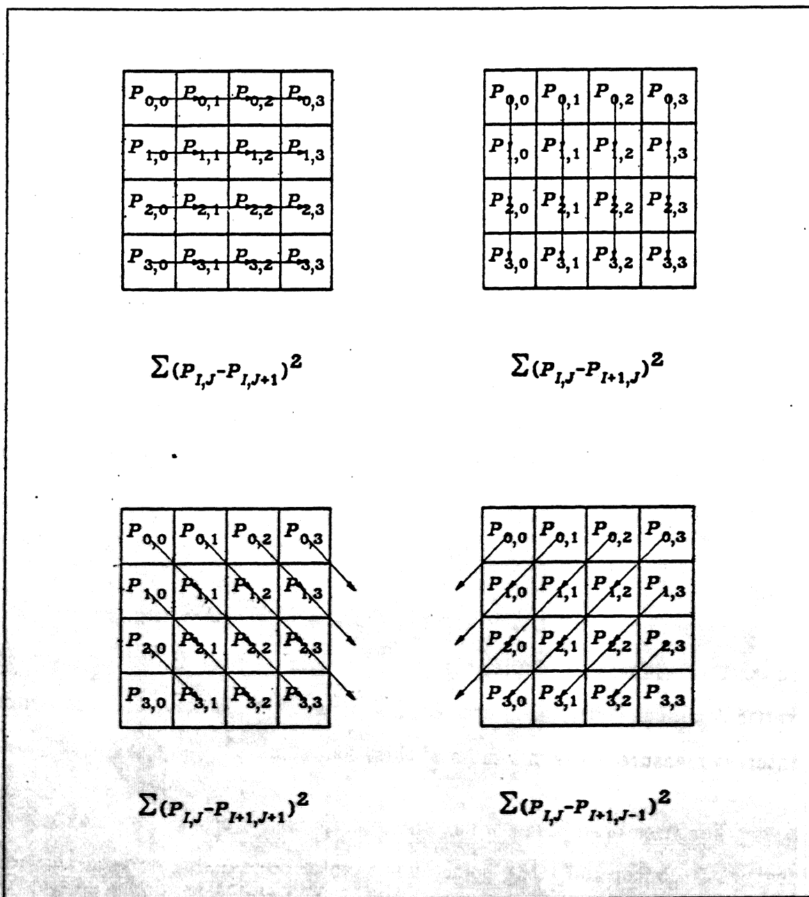
Figure 5-2: A typical interest operator window, and the four sums calculated over it ( P_{I,J} are the pixel brightnesses). The interest measure of the window is the minimum of the four sums.
