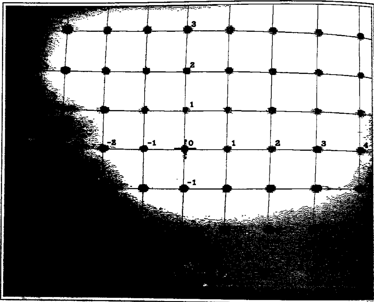
Figure 4-4: Results of the calibration program. The distortion polynomial it produced has been, toed to map an UMdistorted grid of ideal spot positions into the calculated real world ones. The result is superimposed on the original digitised spot image, making any discrepancies obvious.
