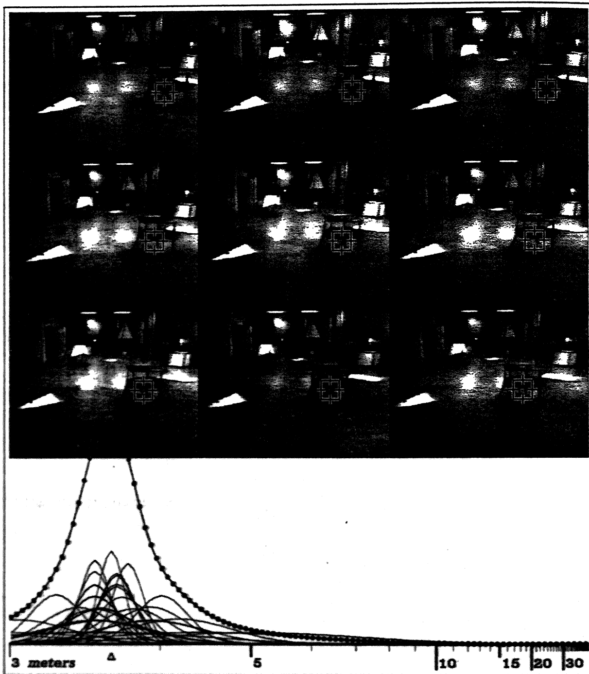
Figure 7-1: A typical ranging. The nine pictures are from a slider scan. The interest operator chose the marked feature in the central image, and the correlator found it in the other eight. The small curves at bottom are distance measurements of the feature made from pairs of the images. The large beaded curve is the sum of the measurements over all 36 pairings. The horizontal scale is linear in inverse distance.
