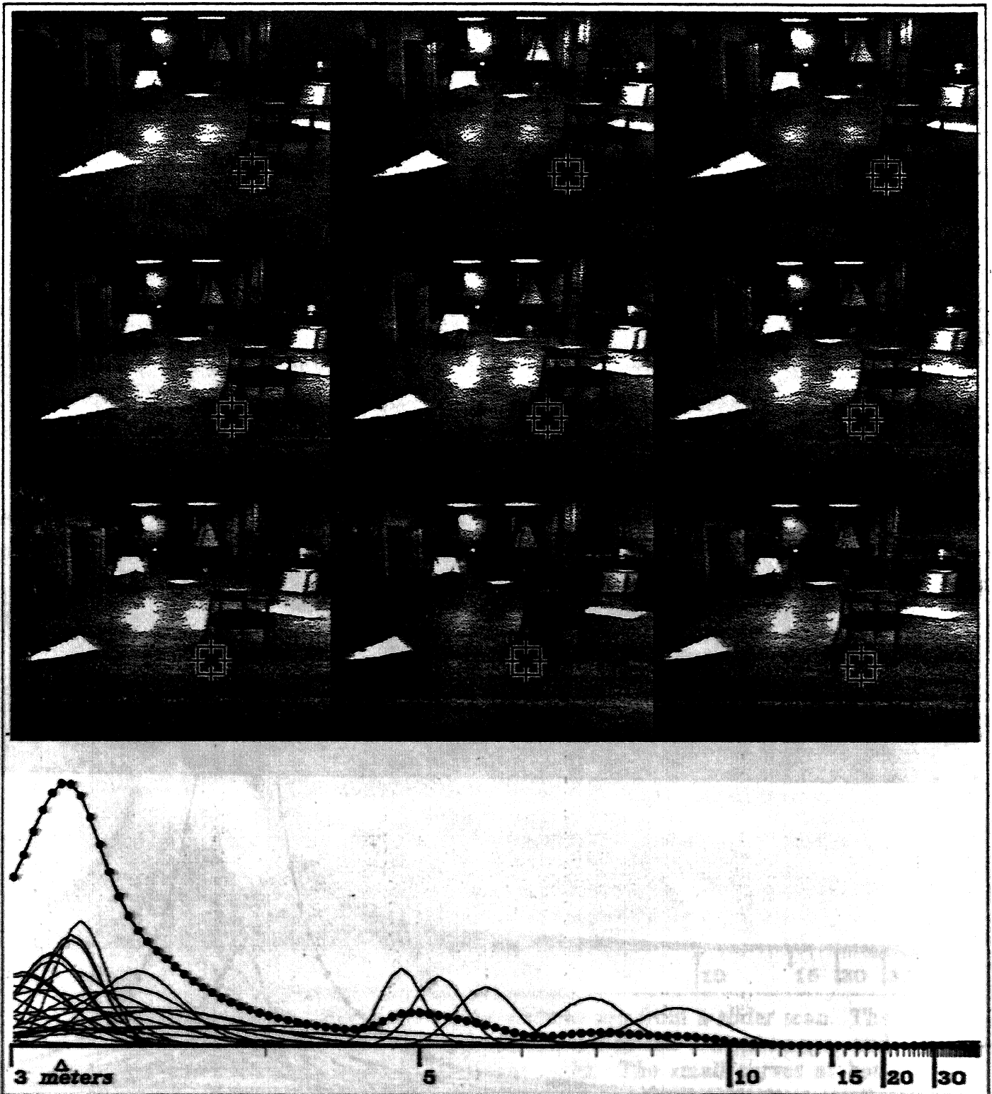
Figure 7-3: Ranging in the presence of a correlation error. Note the mismatch in the last image.
