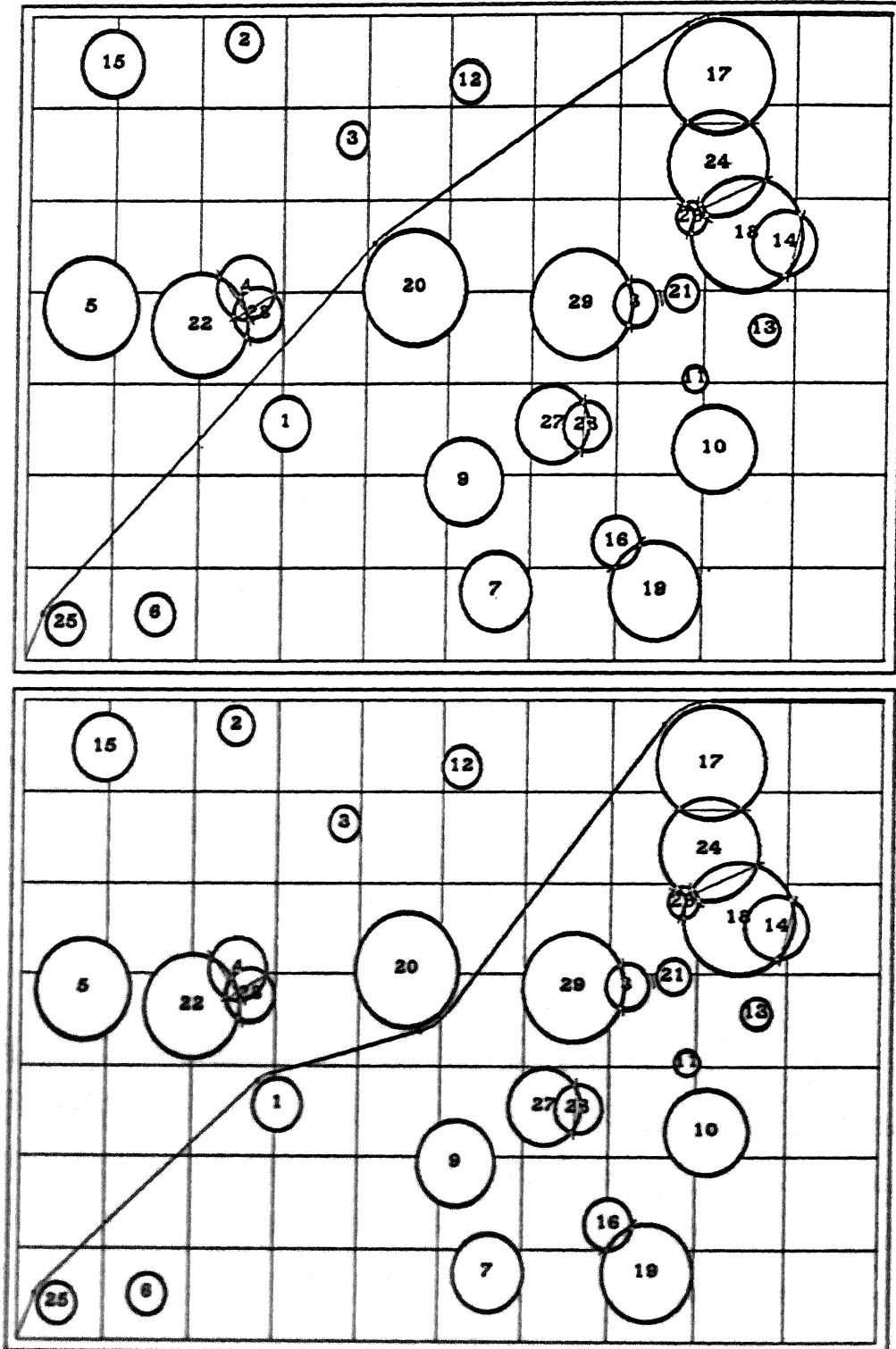
Figure 8-4: A case where the approximate and exact methods differed. Top diagram is the exact solution, bottom one is the approximate algorithm's guess.
