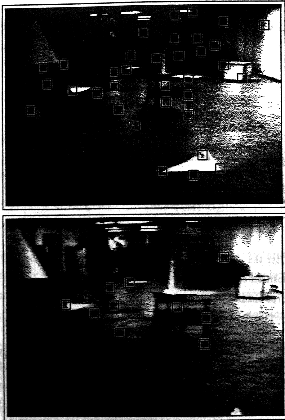
Figure 7-4: The feature list before and after the mutual-distance pruning step. In this diagram the boxes represent features whose three dimensional position is known.
