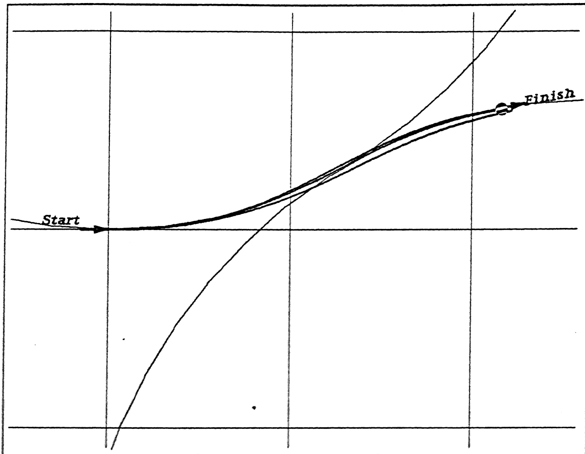
Figure 8-5: An example of the simulator's behavior. The diagram is a plan view of the path executer's world model; the grid cells are one meter on a side. The cart's starting position and final destination and orientation are indicated by arrows. The two large circles, only portions of which are visible, represent the analytic two-arc path. It goes from Start through the tangent of the two circles to Finish. The heavier paths between the two points represent the iterations of the simulator as its parameters were adjusted to compensate for the cart's dynamic response.
