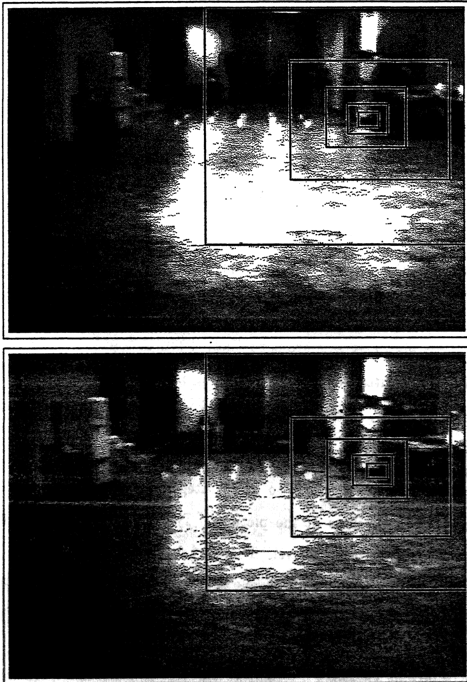
Figure 6-1: Areas matched in a binary search correlation. Picture at top contains originally chosen feature. The outlined areas in it are the prototypes which are searched for in the bottom picture. The largest rectangle is matched first, and the area of best match in the second picture becomes the search area for the next smaller rectangle. The larger the rectangle, the lower the resolution of the pictures in which the matching is done.
