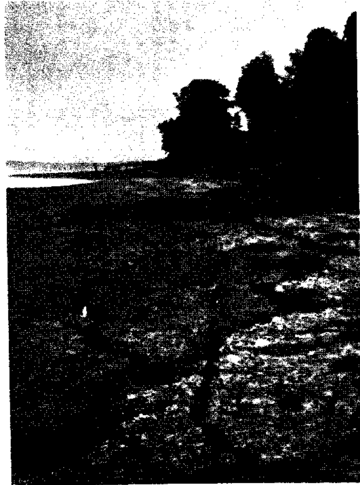
B. Cracks made by earthquake in tidal mud near head of Bolinas Lagoon. O.K.G.
