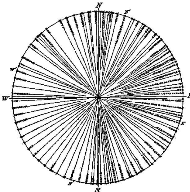
FIG. 65.—Directions of earthquake motion. FIG. 66.—Statistical representation of the directions of fall of monuments in the cemeteries south of San Francisco. Each x represents a monument which fell in the direction indicated by the radius on which the x is placed. After Omori.
