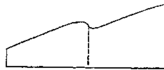
FIG. 6.—Cross-profile of side-hill sag shown in plates 7B and 10B.
