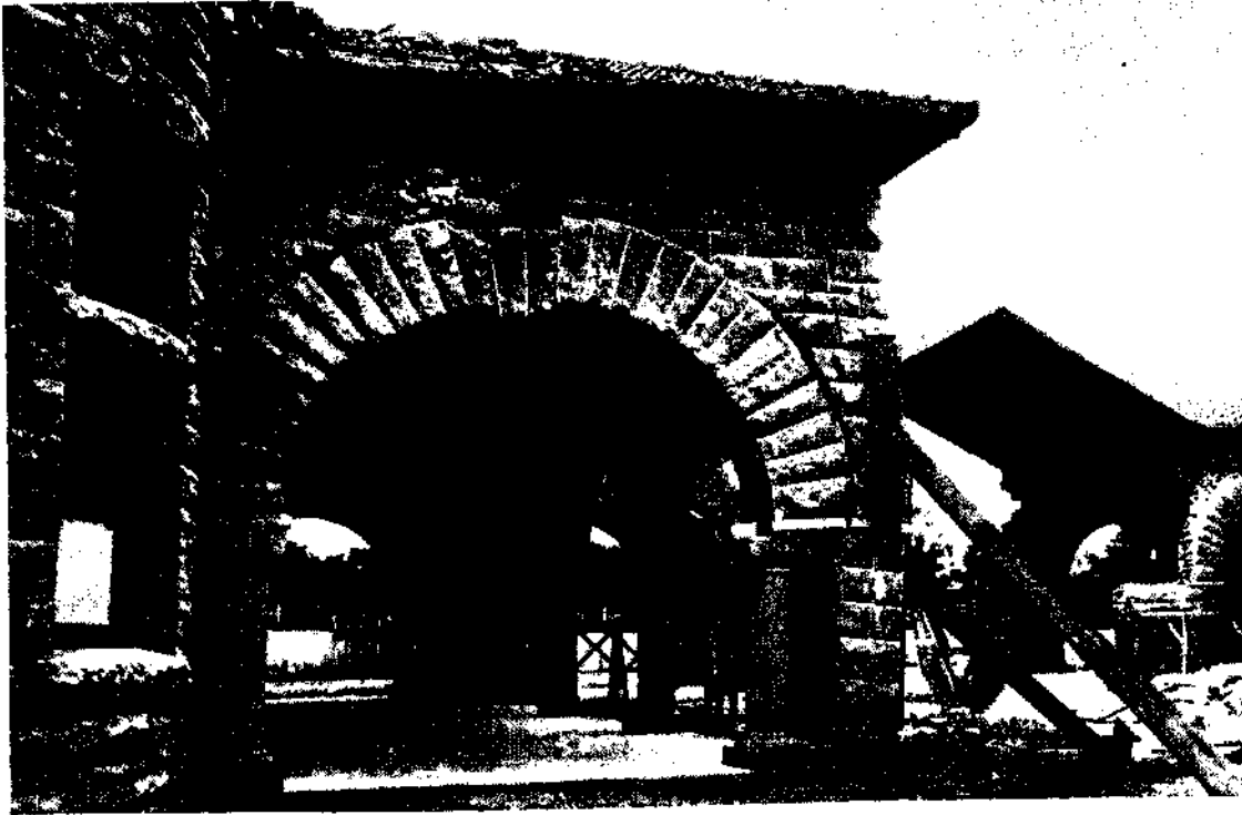
A. "Wrecked arolea, Geology Building, Stanford University. Per J, O. B.
