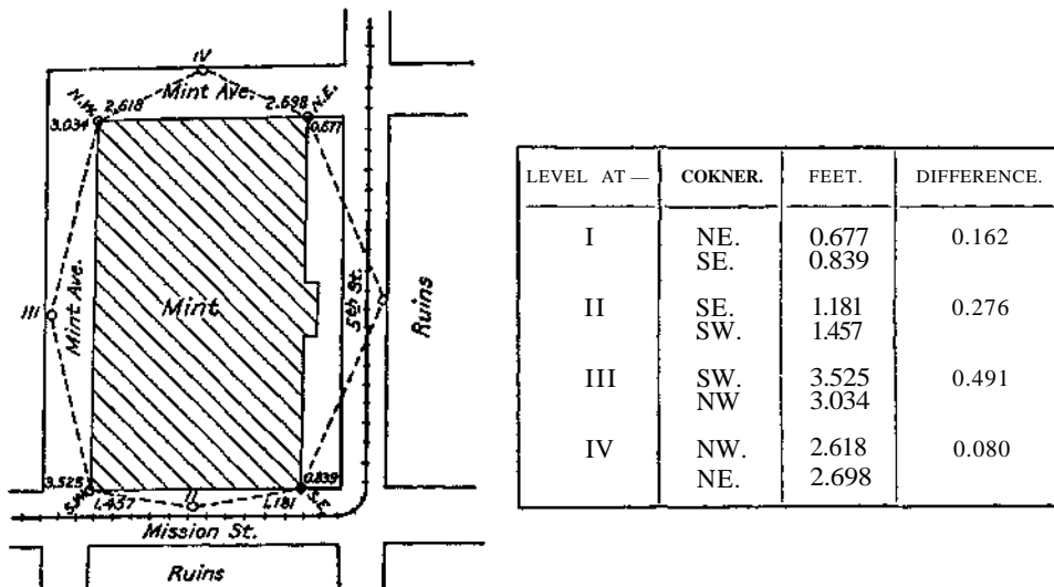
FIG. 54.—Map showing relative levels of four corners of Mint, San Francisco.
