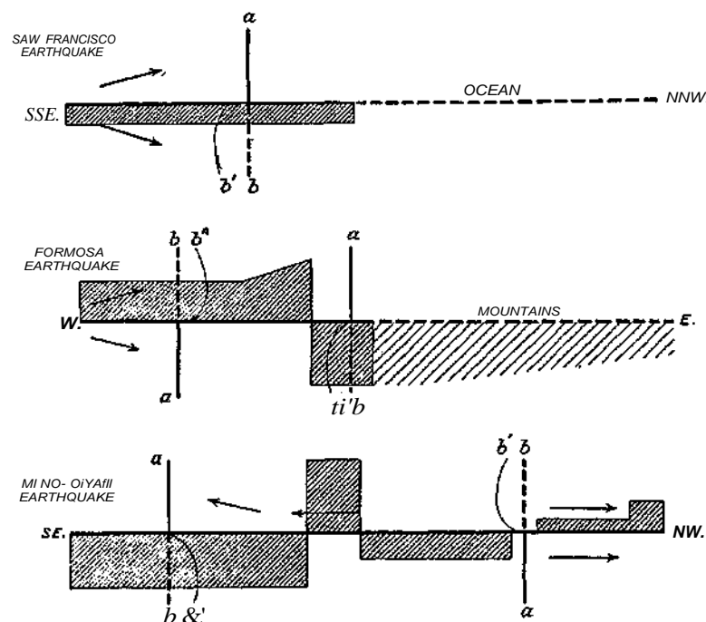
FIG. 43 a. — Full line is fault (ascertained). Shaded part is depressed region. Dotted line is probable continuation of fault. Lightly shaded part represents probable depression. Arrow indicates the direction of maximum (vibratory) motion.
