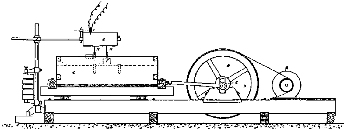
FIG. 60.—Diagram of construction of apparatus used in experiments
