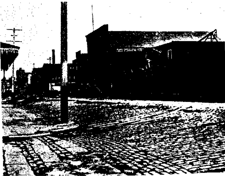
C. Eighteenth Street, just east of Shotwell, Fissuring and depression of Pavement. H. O. W.
