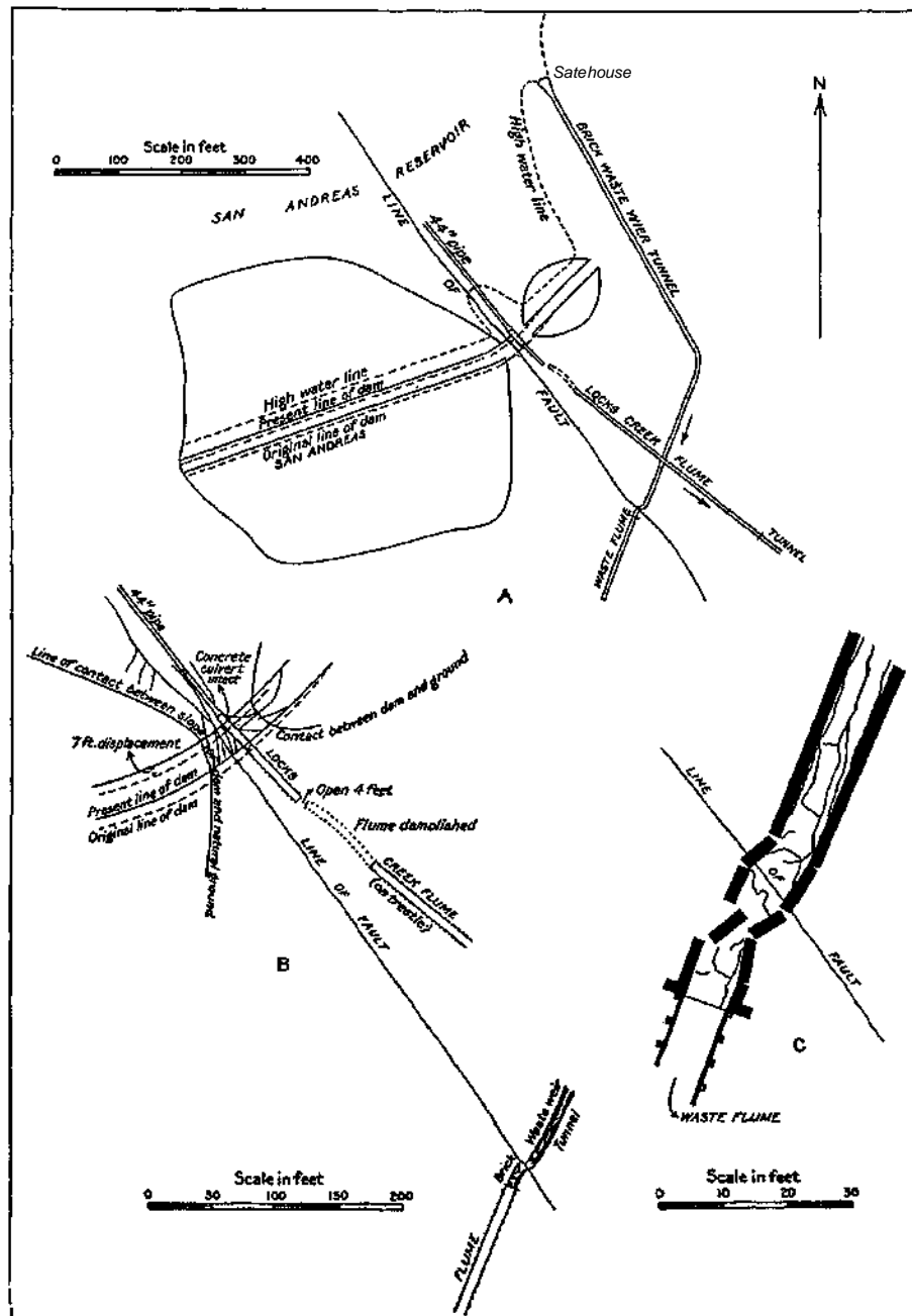
FIG. 3.— Intersection of San Andreas dam by fault. A. Plan of dam in two parts, with rock between. B. Relation of dam to waste weir tunnel. C. Detail of waste weir tunnel.
