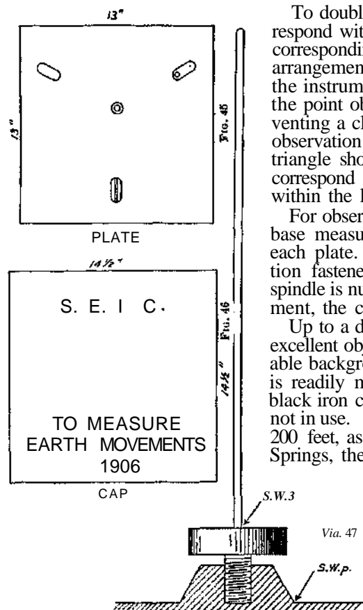
FIG. 46. — Diagram of bronze plate on monuments.
