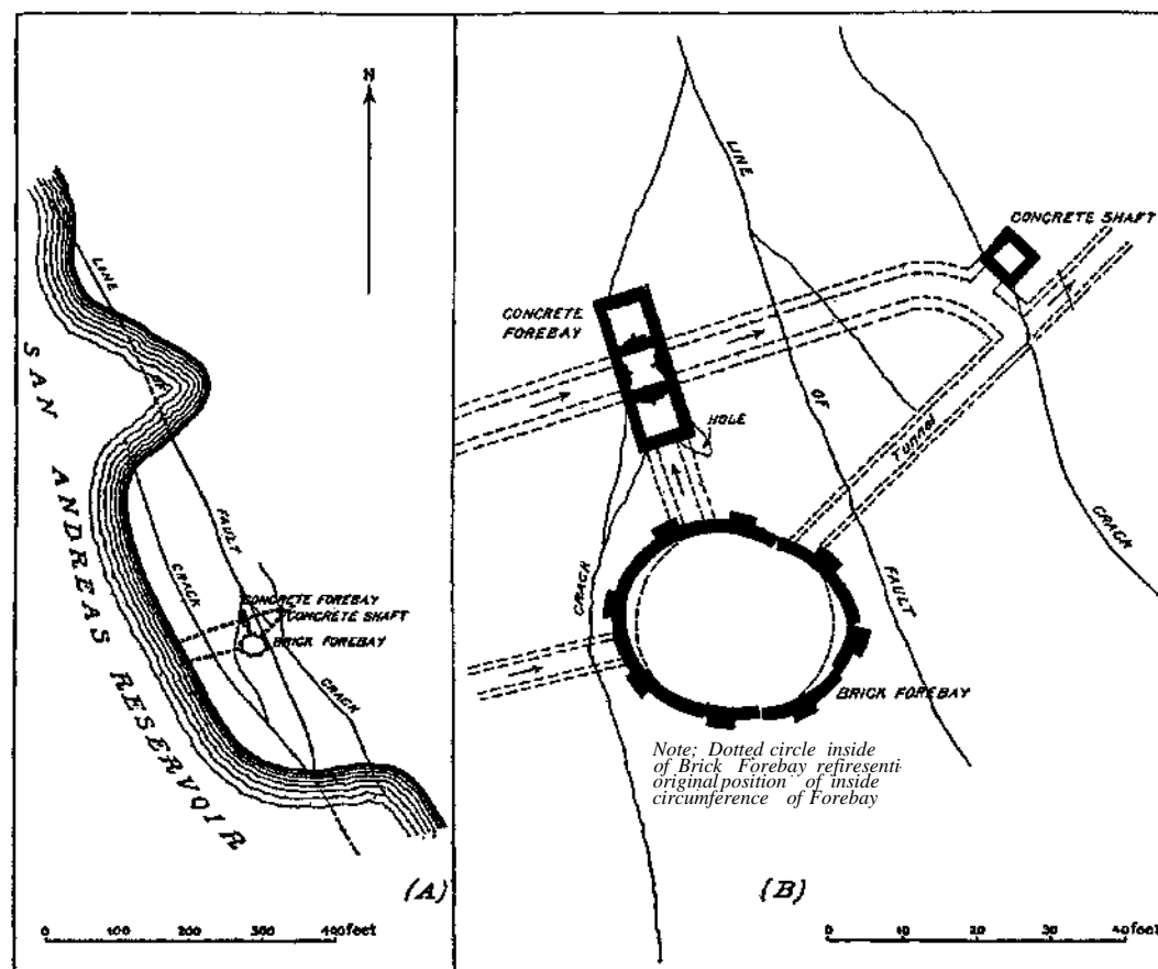
FIG. 35. — Main and auxiliary faults, San Andreas Lake. A. General Plan. B. Detail. After H. Schussier.
