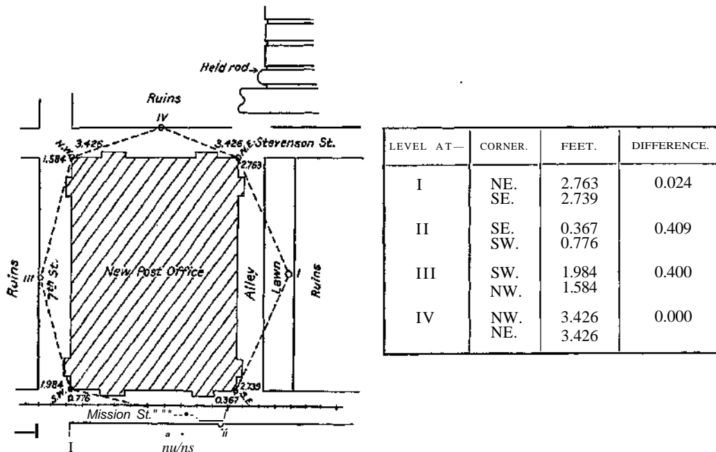
FIG. 52. — Map showing relative levels of four corners of new Post-office, San Francisco.
