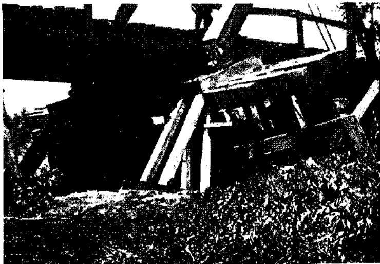
A. Bridge over Salinas Eiver, 4 miles south of Salinas. South terminal pier thrust south 7 feet. A. O. L.
