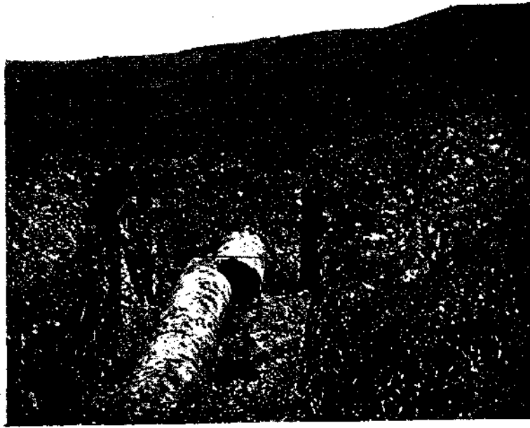
A. Offset in 30-inch water-pipe by fault. Northwest of San Andreas Lake. E. L. H.
