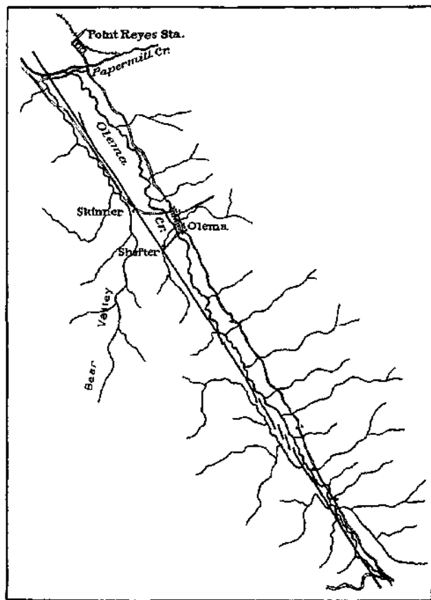
FIG. 1(i). — Map of fault-trace from Papormill Creek southward. Scale, 1:112,500.
