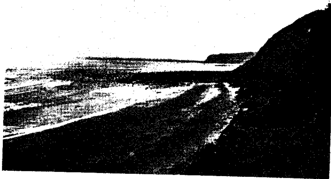
B. Bed-rock shoal Bear Boliaas, with clam patch near water edge. Dnxttry Point au3 reef is the distance. G. K. Q.
