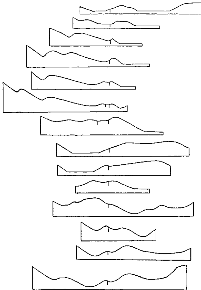
FIG. 9.—Cross-profiles of the Rift arranged in geographical order with the most northerly at top and northeast ends at the right. Positions of fault-trace and its branches are indicated. The profiles are copied from field sketches made without measurement.
