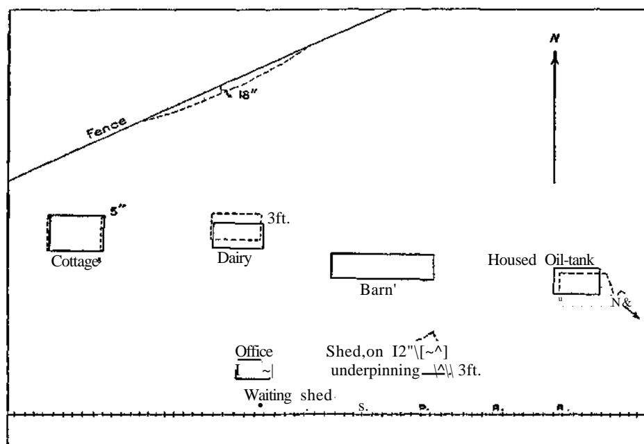
FIG. 48—Displacement of buildings at Chittenden
