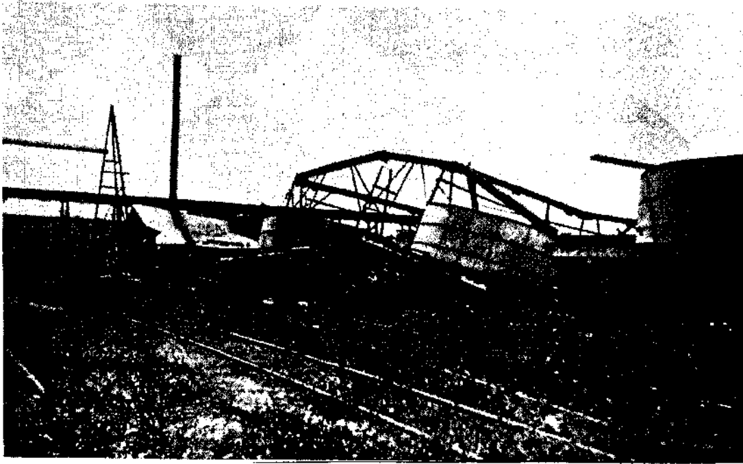
A. Alvatadoi Wreok of molasses tankB, Alameda Sugar Company, E. W. B.
