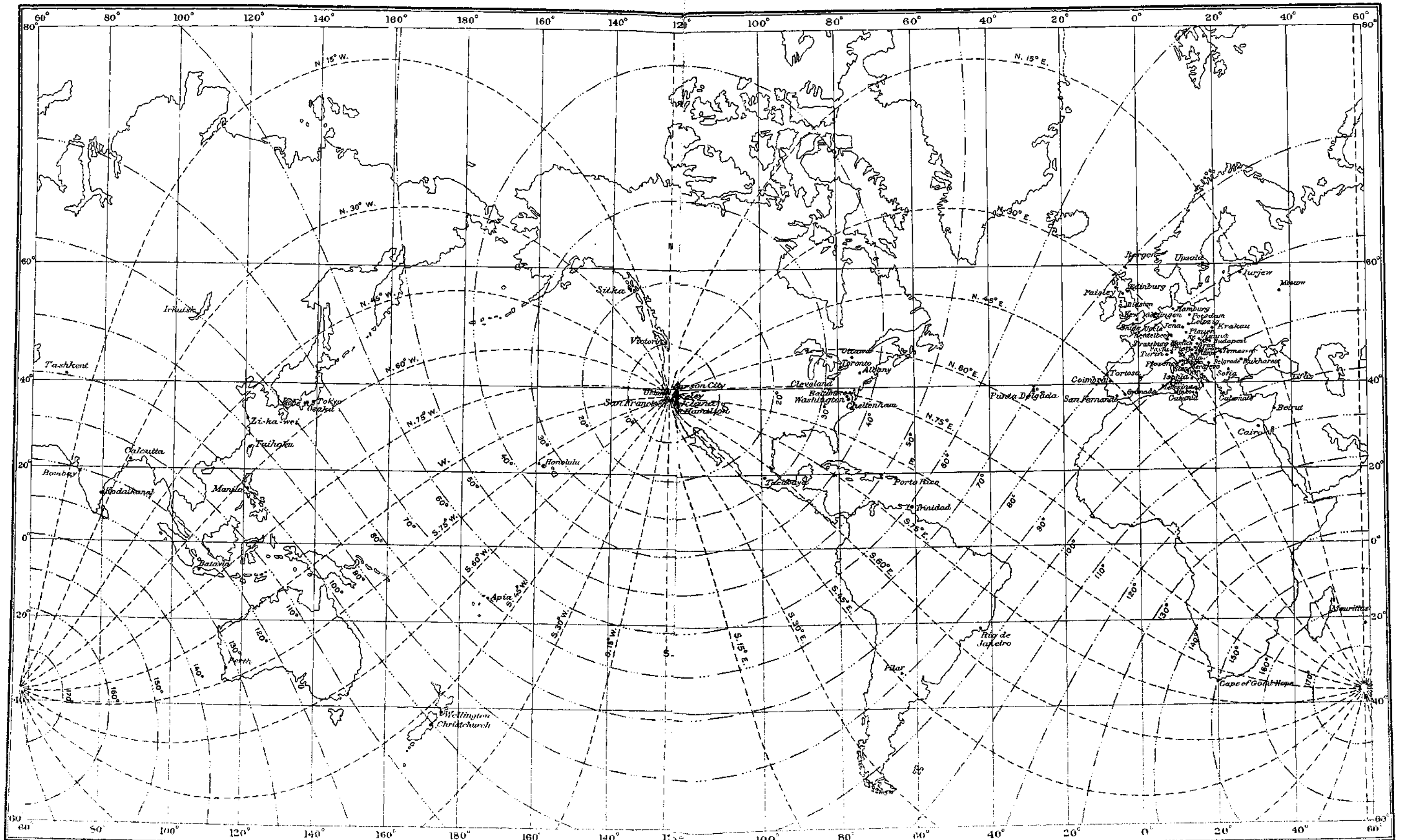
MAP SHOWING DISTANCES AND DIRECTIONS FROM THE ORIGIN OF THE SHOCK
