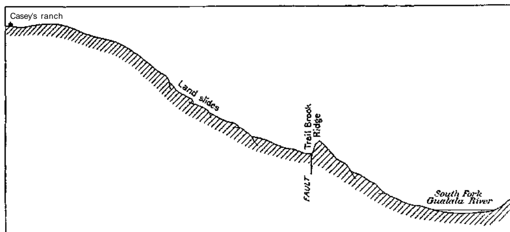
FIG. 14.—Profile of southwest side of South Fork of Gualala River, showing relation of fault to geomorphie features.
