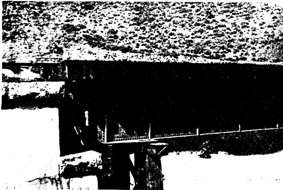
B. Steel bridge over Pajtro Eirer, near Oiiittenden, dragged from its abutment 3.5 fwt. Compare Fig. 43. A. O. L.
