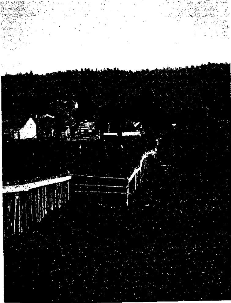
A. Fence offset by fault. Looking northwest. Camera was alined with straight part offence beyond the disturbance, to bring out flexure as well as offset of fence. Q. K. G.
