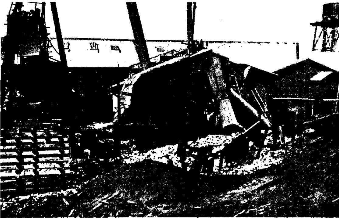
B. U. O. O.'s mill, Fort Bragg, Smoke stack 5 feet in diameter. Entire structure tilted out of plumb to south, 1 foot in 20 feet.
