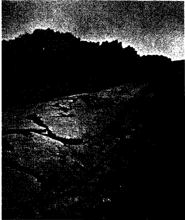
A. Road embankment broken by shaking of soft ground beneath. Southwest of Point Beyes Station and 10 rods from fault-trace. Q. K. Q.
