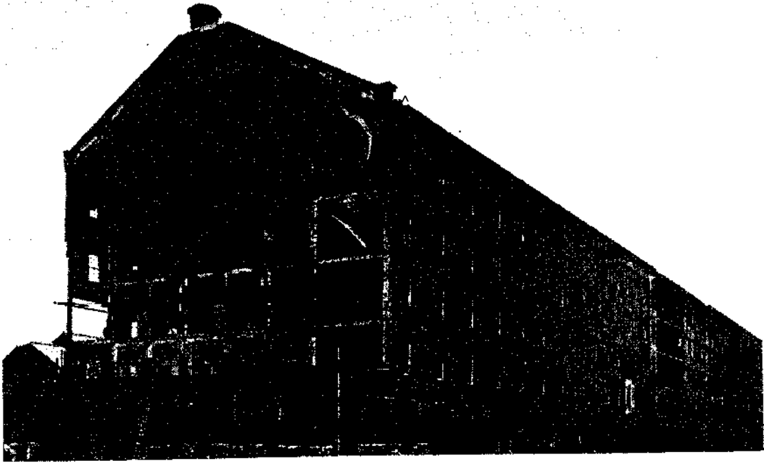
A. Spreckela sugar mill, near Salinas. Entire building buckled. Looking southeast. R. L. H.
