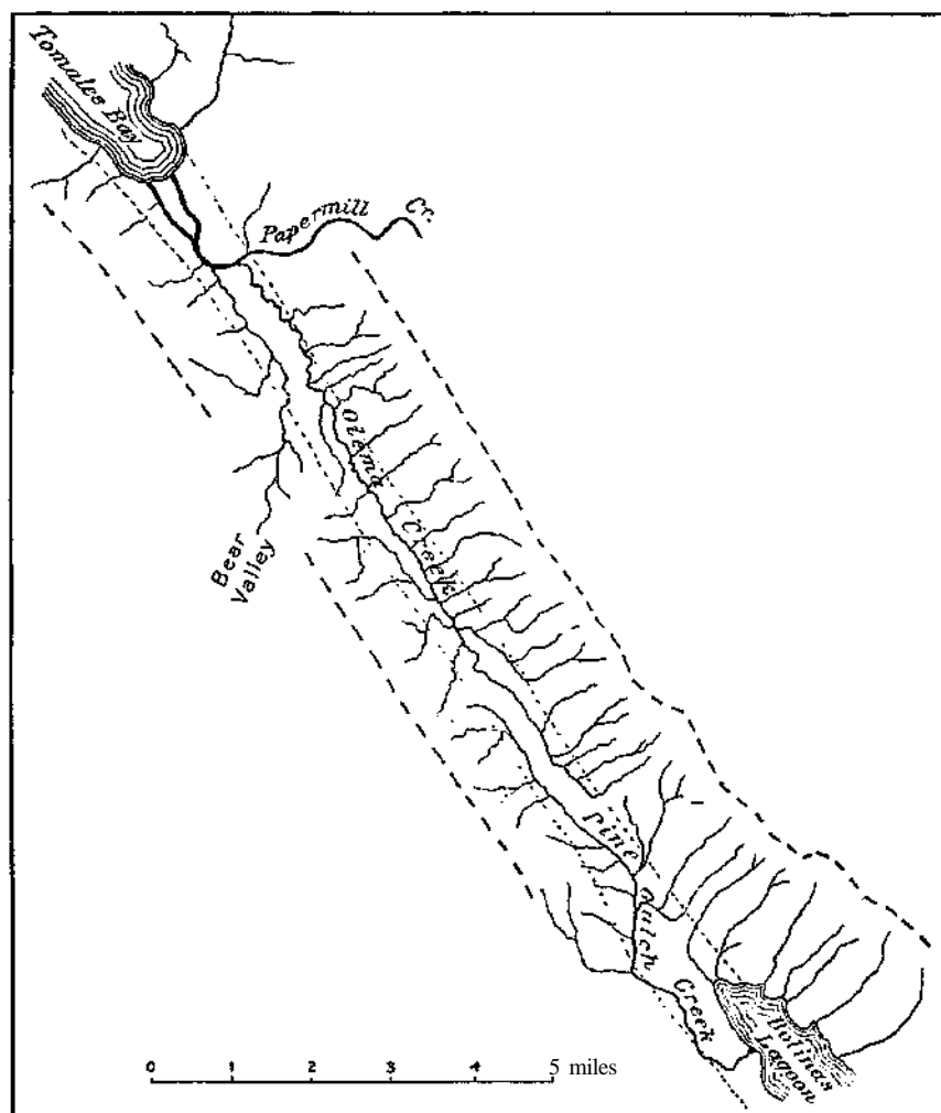
FIG. 2.—Drainage map of Bolinas-Tnmales Valley. Heavy broken lines show crests of bounding ridges. Light broken lines indicate limits of Rift topography.
