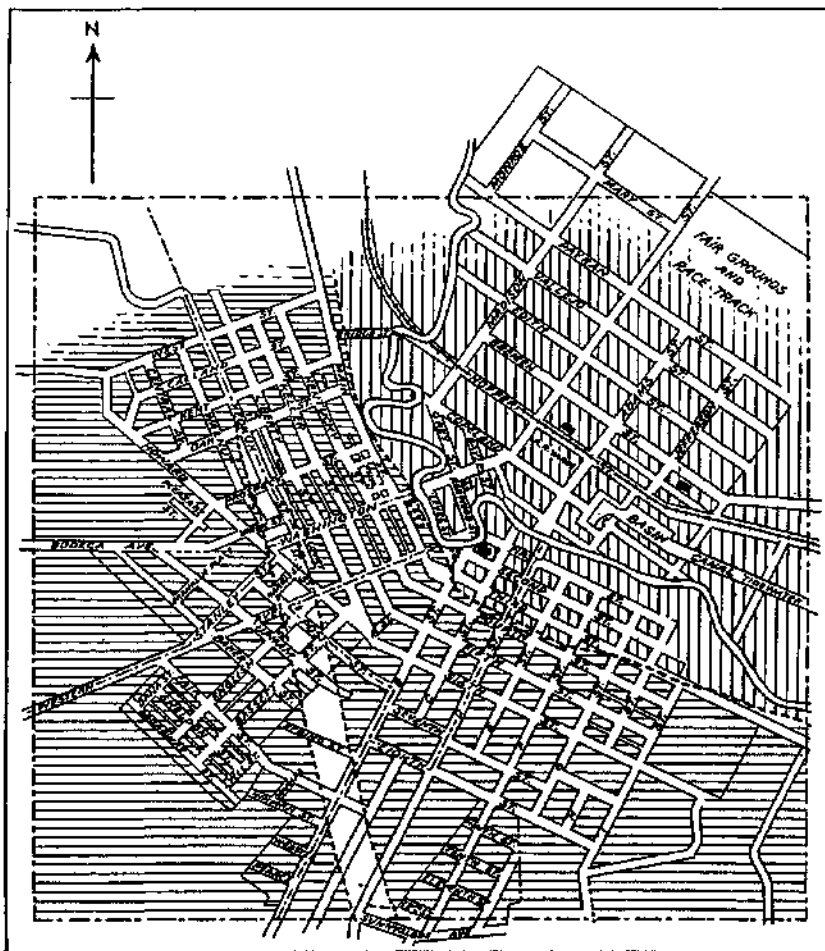
FIG. 04. — Distribution of intensity in Petaluraa. Vertical lines represent area of low-alluvial land, on which nearly all chimneys were damaged. Horizontal lines represent slopes underlain by rock, on which about half the chimneys were damaged. The solid black areas and dots represent exceptionally severe damage. The blank area inclosed by dotted lines represents a belt of practically no damage. By R. S. Hoiway.
